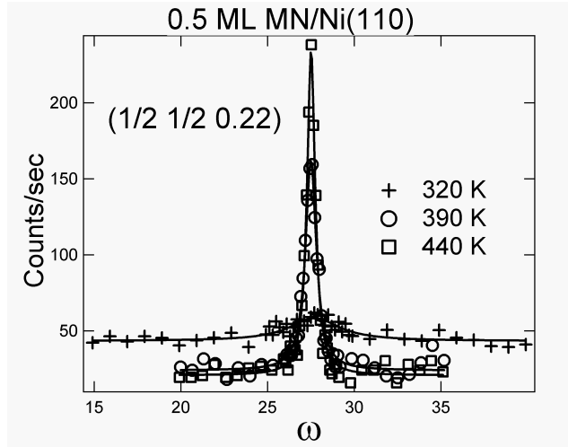
FIG. 19. Rocking scan through a superstructure reflection of Ni(110)- c(2 \times 2) Mn surface, showing the increasing of domain size with temperature.
