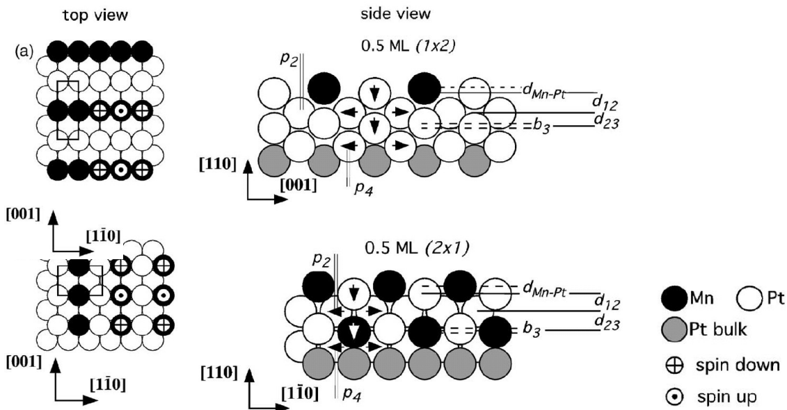
FIG. 23 Model structure of: (a) Pt(110)-(1×2)Mn, and (b) Pt(110)-(2×1)Mn. On the top view, the surface unit cell is shown and the magnetic order is sketched with arrows pointing up and down. Note that the AF ordering doubles the surface unit cell.
