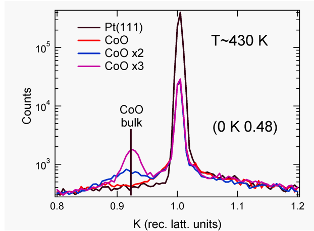
FIG. 39. SXR measurements collected by scanning the momentum transfer parallel to the \vec{b}_2 reciprocal space vector of the hexagonal Pt(111) surface cell. The curves refer to clean Pt substrate and to subsequent three steps of Co deposition (1 ML) and O_2 dosing (20 L).
