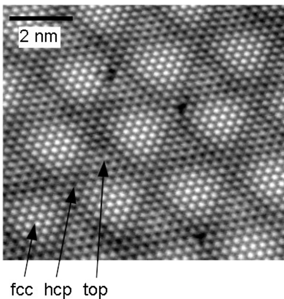
FIG. 35. Atomic resolved image of the CoO/Pt(111) moiré structure. ( I_t = 1 nA; V_s = -2 mV). Regions with Co in fcc, hcp, and on-top sites of the Pt substrate atoms were identified by comparison with images showing triangular stacking faults. 125
