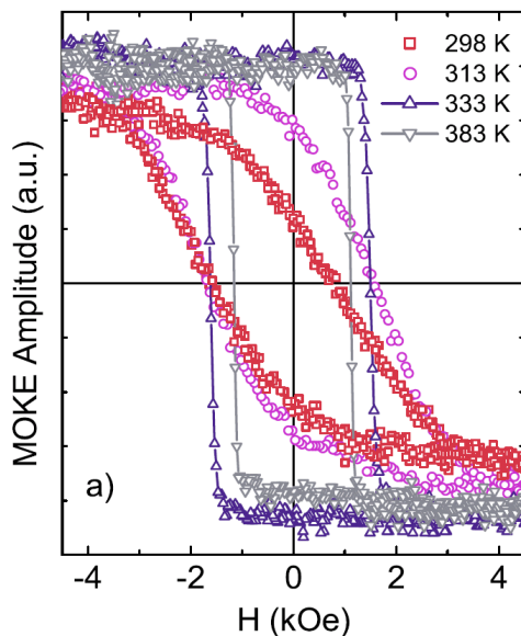
FIG. 42. Polar MOKE of (NiO 3ML /CoO 3ML ) 3 /PtCo/Pt(111) versus T close to T B .
