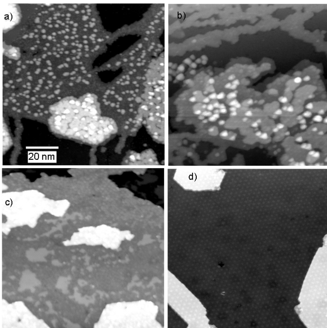
FIG. 34. 100 \times 100 \text{ nm}^2 STM images of 1 ML Co/Pt(111) deposited at RT and: (a) dosed with 50 L \text{O}_2 ; (b) annealed and dosed with 50 L \text{O}_2 at 450 K; (c) annealed and dosed with \text{O}_2 at 570 K; (d) sample (c) followed by a further annealing under oxygen at 730 K. Image processing was used in (d) to reduce the step height, making the corrugation on the terraces more apparent. ( I_t = 0.1 \text{ nA} ; V_s = +0.5 \text{ V} in (a), (b), and (d); V_s = +1.2 \text{ V} in (c)).
