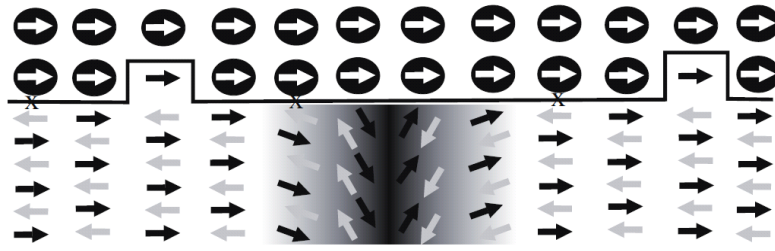
FIG. 6 Schematic view of a vertical domain wall in the AF layer. It appears as an energetically favorable state of F/AF systems with rough interfaces (from ref. 6)
