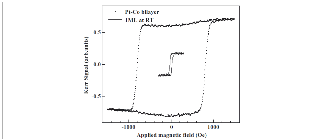
FIG. 33. Polar Kerr hysteresis loop for, respectively, 1 ML of Co/Pt(111) grown at RT (smaller loop) and at 540 K (larger loop) (from ref. 46)
