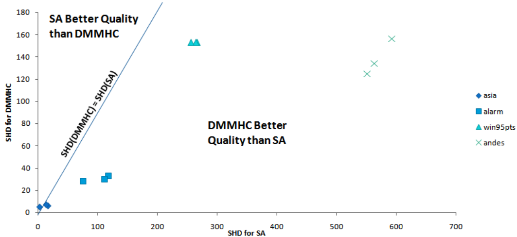
Figure 6.3: Average SHD(DMMHC) vs SHD(SA) with respect to sample size in transition graph
