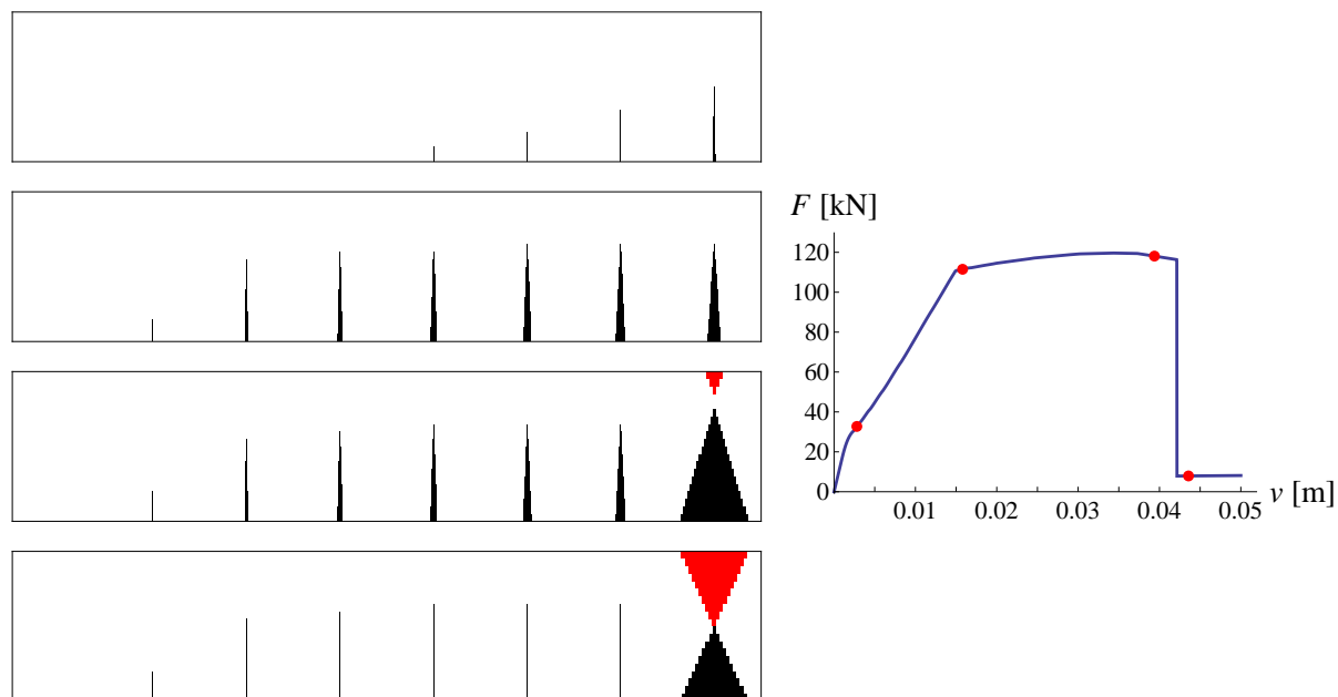
Figure 4.32: Simply supported beam: discontinuities (cracks) at different stages of analysis. Slika 4.32: Prostoležeći nosilec: nezveznosti (razpoke) u posameznih fazah analize.
