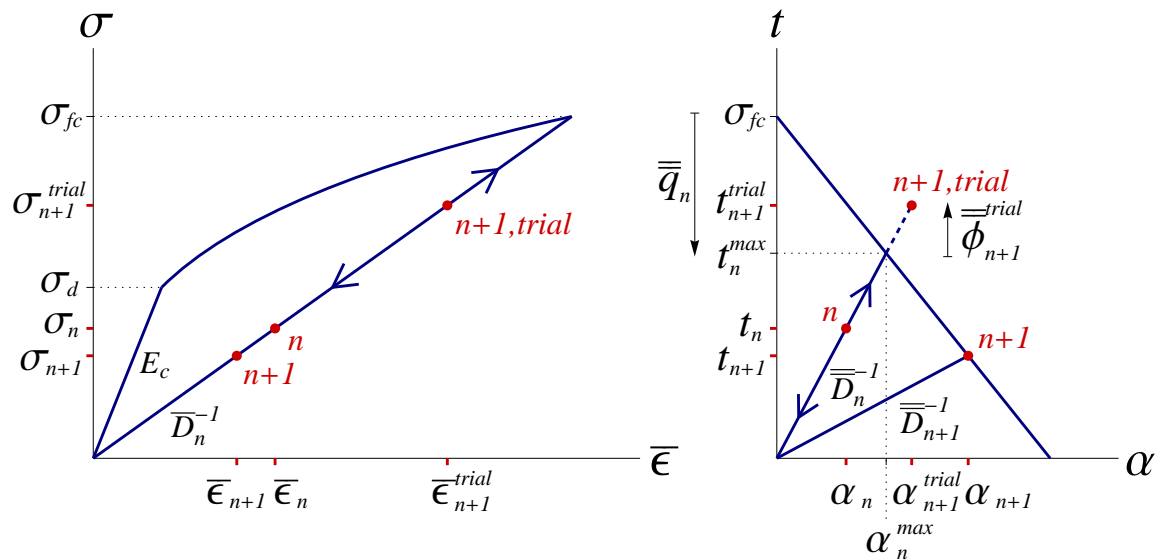
Figure 4.15: Stress in the bulk (left) and traction at the discontinuity (right) of a concrete layer: value from the previous step ( n ), and trial and final values from the current step ( n+1 ).
