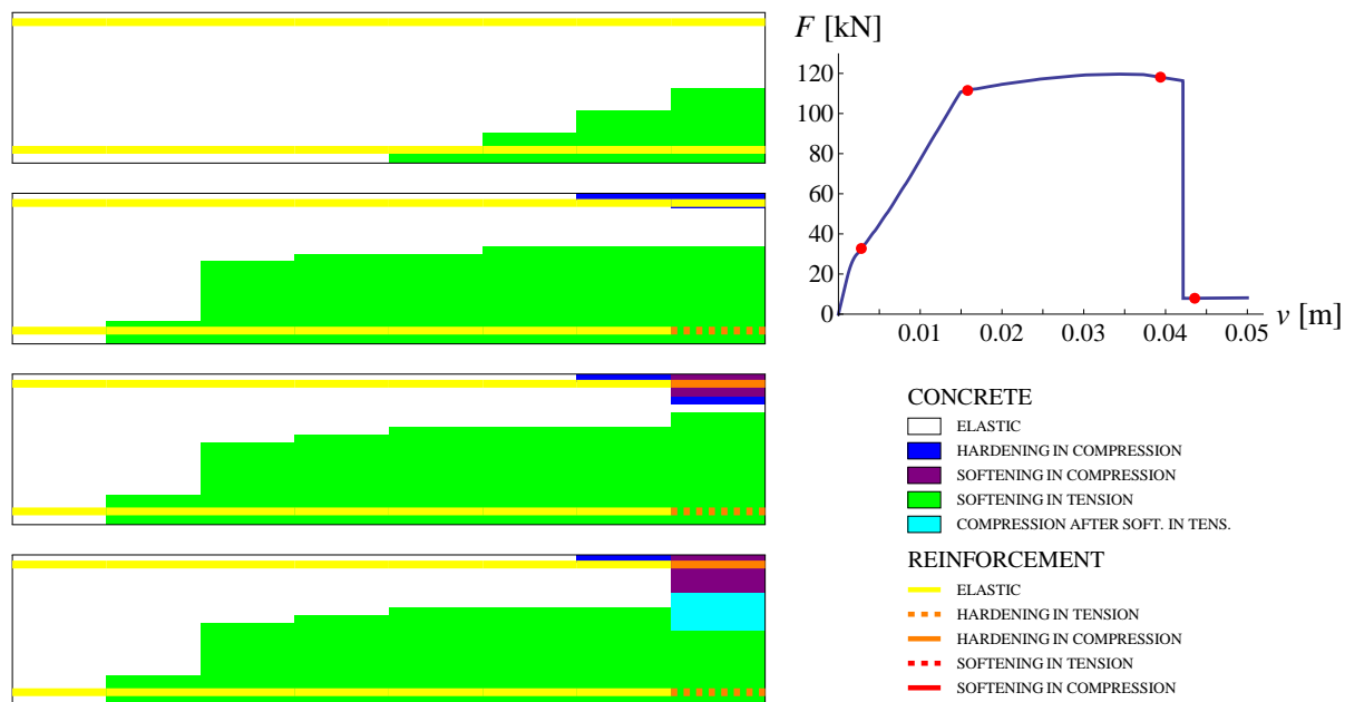
Figure 4.31: Simply supported beam: material state at different stages of analysis (marked with dots). Slika 4.31: Prostoležeći nosilec: stanje materijala u posameznih fazah analize (označene s pikami).
