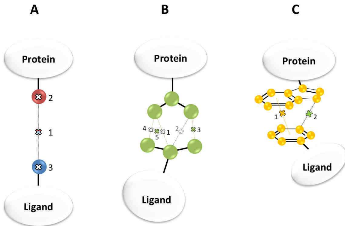
Figure 1- Definition of interaction pseudoatoms (IPAs). (A) Case of hydrogen bonding, ionic interaction, and metal complexation. Two atoms of complementary pharmacophoric properties (red and blue balls) fulfilling interaction rules describe an interaction (dotted line) at a pseudoatom (cross) located at three possible positions: (i) geometric center of interacting atoms (1), (ii) interacting protein atom (2), (iii) interacting ligand atom (3). (B) Case of hydrophobic interactions between protein and ligand hydrophobic atoms (green balls). Only the shortest interaction (number 1) between a single ligand atom and many protein atoms is kept (interaction 2 is not conserved). Remaining hydrophobic IPAs (1, 3, 4) are then clustered to yield IPAs 3 and 5. (C) Case of aromatic interactions between protein and ligand aromatic atoms (yellow balls). Protein and ligand aromatic atoms verifying the aromatic interaction rules define an aromatic interaction (yellow dotted line) with an aromatic IPA set at the mid-distance between both aromatic ring centroids (IPA 1). For aromatic interacting atoms, not respecting the aromatic interaction rule but fulfilling a hydrophobic interaction, a hydrophobic interaction (green dotted line) and IPA (IPA 2) is defined between the closest protein and ligand atoms.
