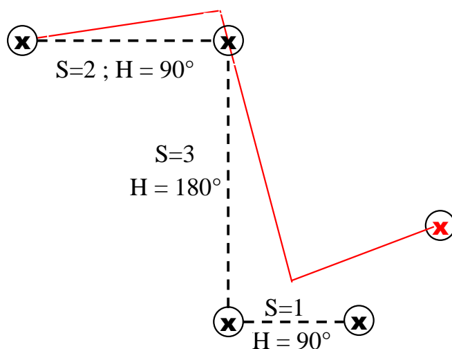
Figure 2.18: Drift errors of the PDR technique
