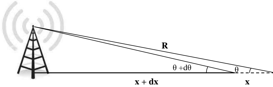
Figure 2.16: typical measurement error in AOA method
