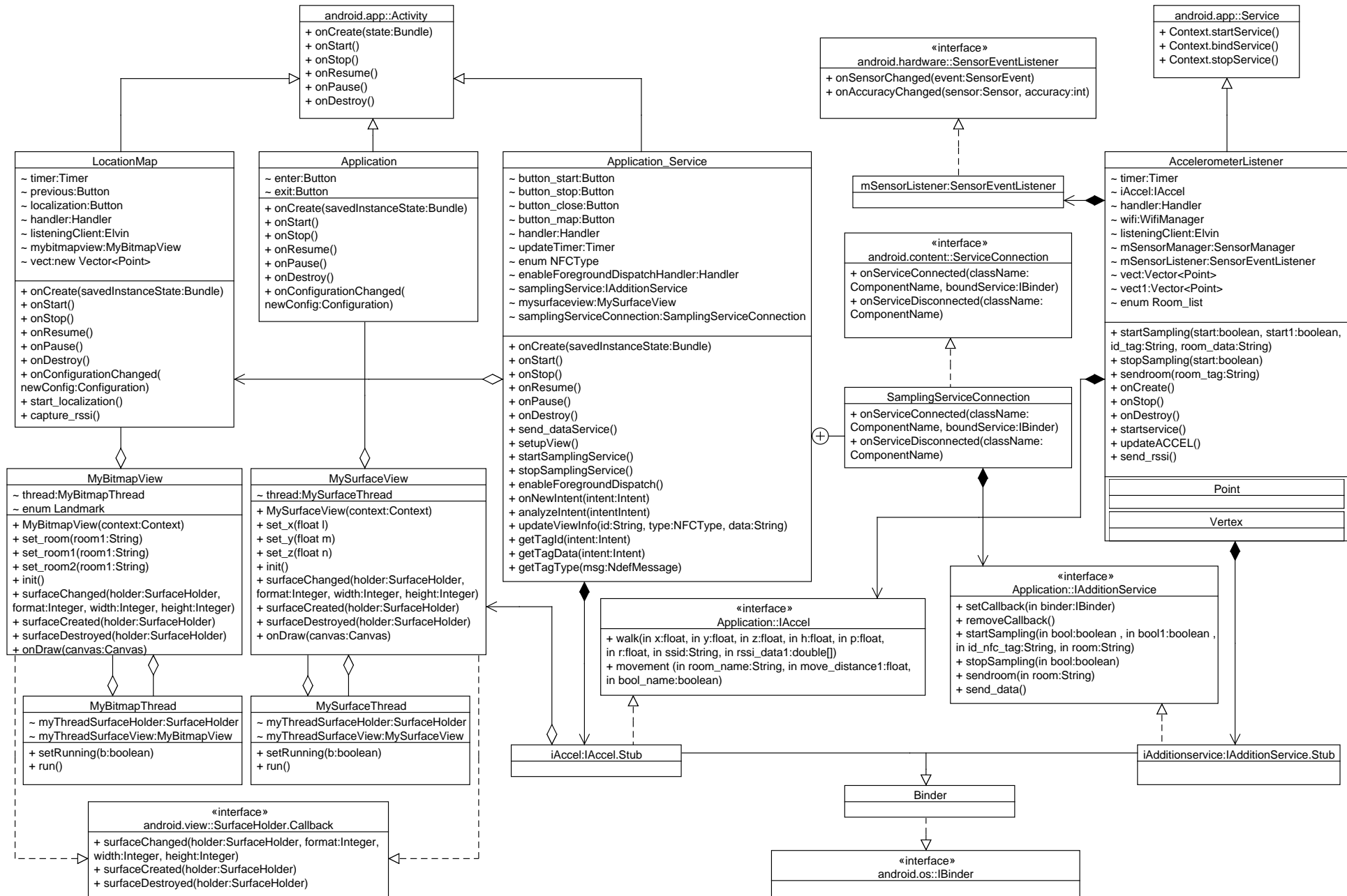
Figure 2: The User side program described by the UML diagram
