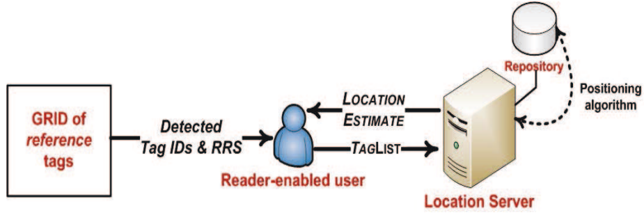
Figure 4.2: RFID-based Positioning System Architecture.
