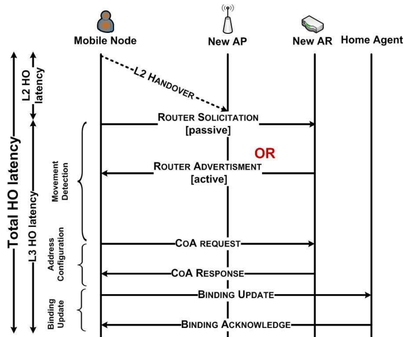
Figure 6.3: Mobile IP handoff mechanism.
