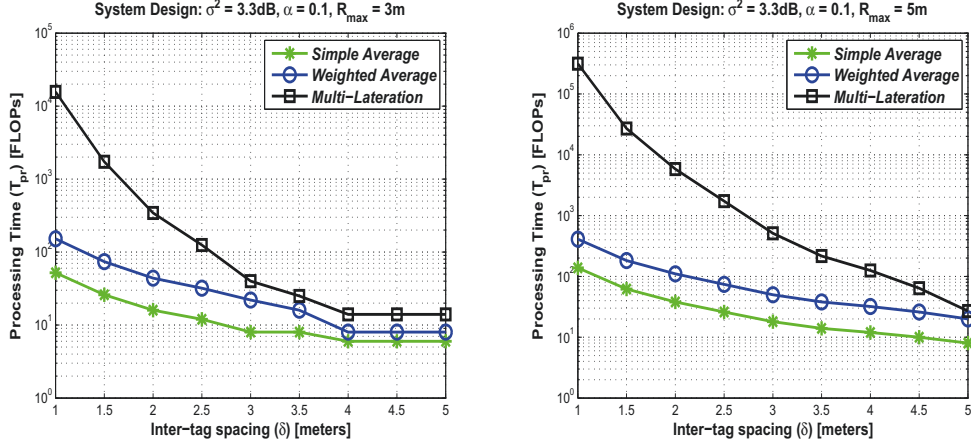
(a) Processing time vs \delta when R_{max} = 3m .
