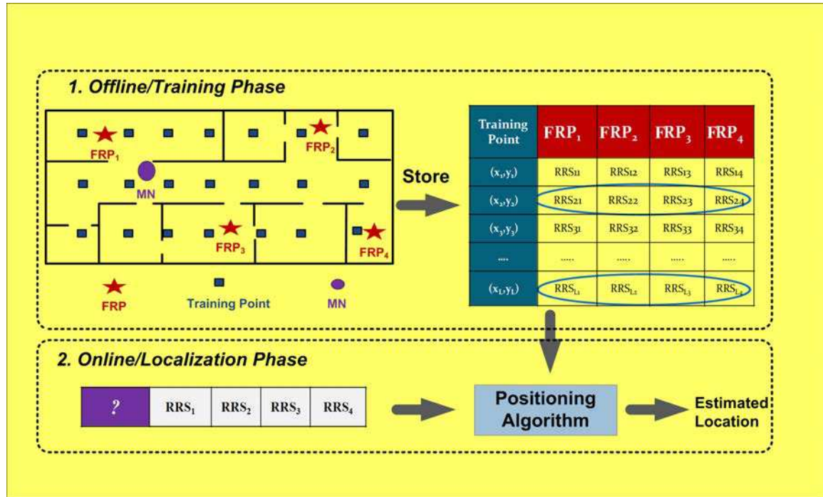
Figure 2.3: Scene Analysis Positioning Technique.
