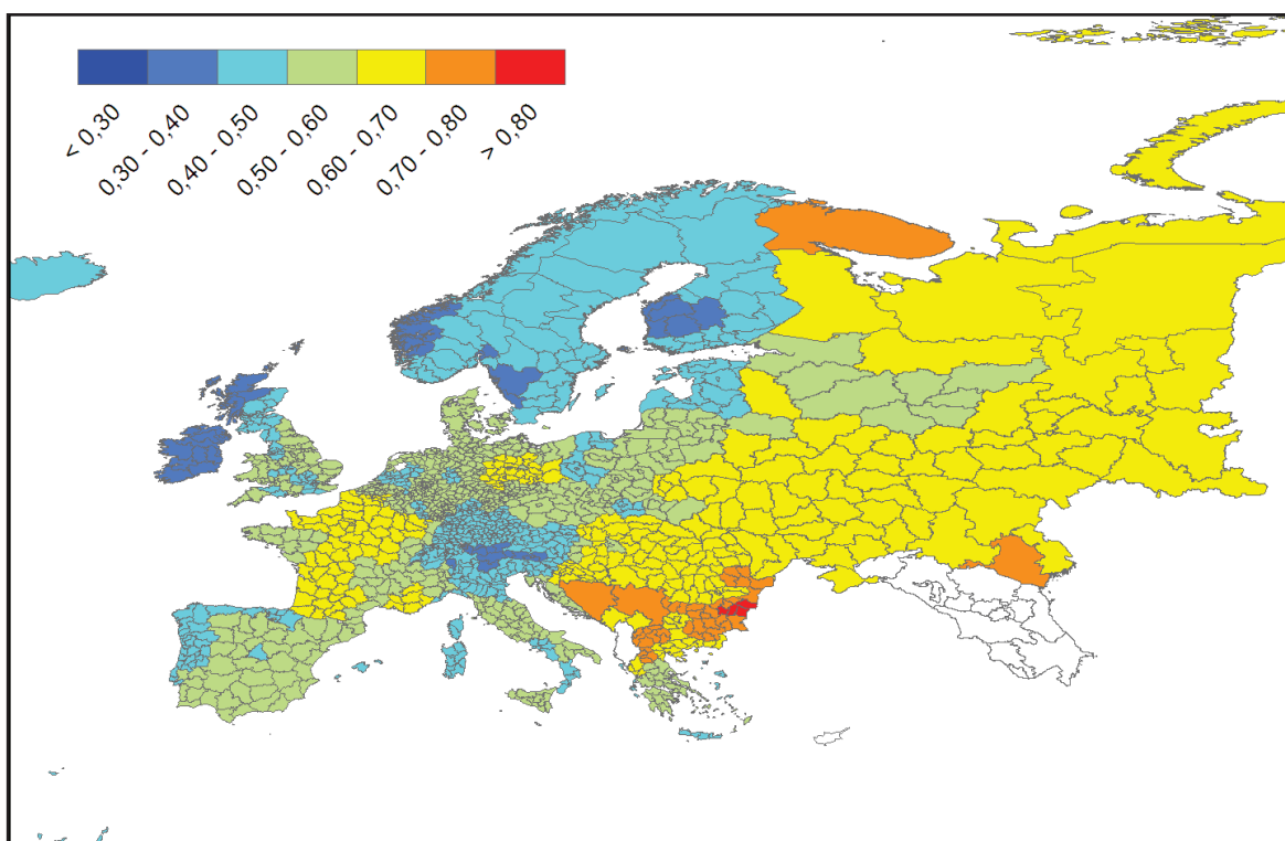
Figure 3.68 Marital status, 1930
