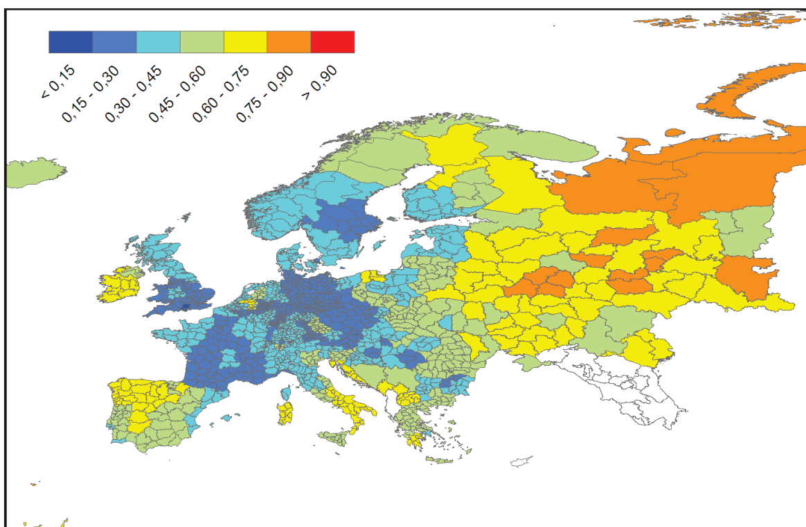
Figure 3.64 Marital fertility, 1930
