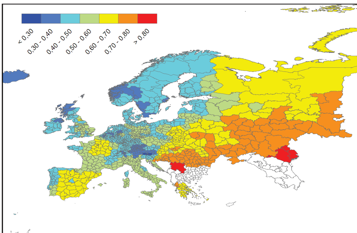
Figure 3.66 Marital status, 1870
