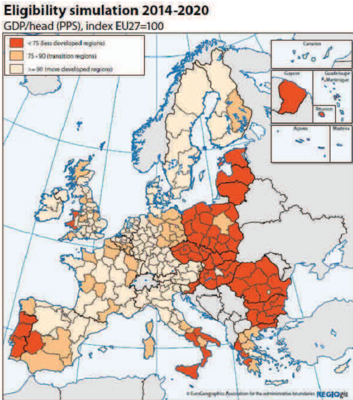
Figure 3.10 Eligibility simulation 2014-2020
