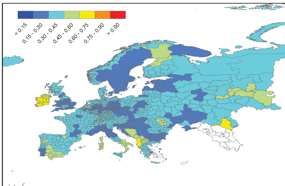
Figure 3.65 Marital fertility, 1960
