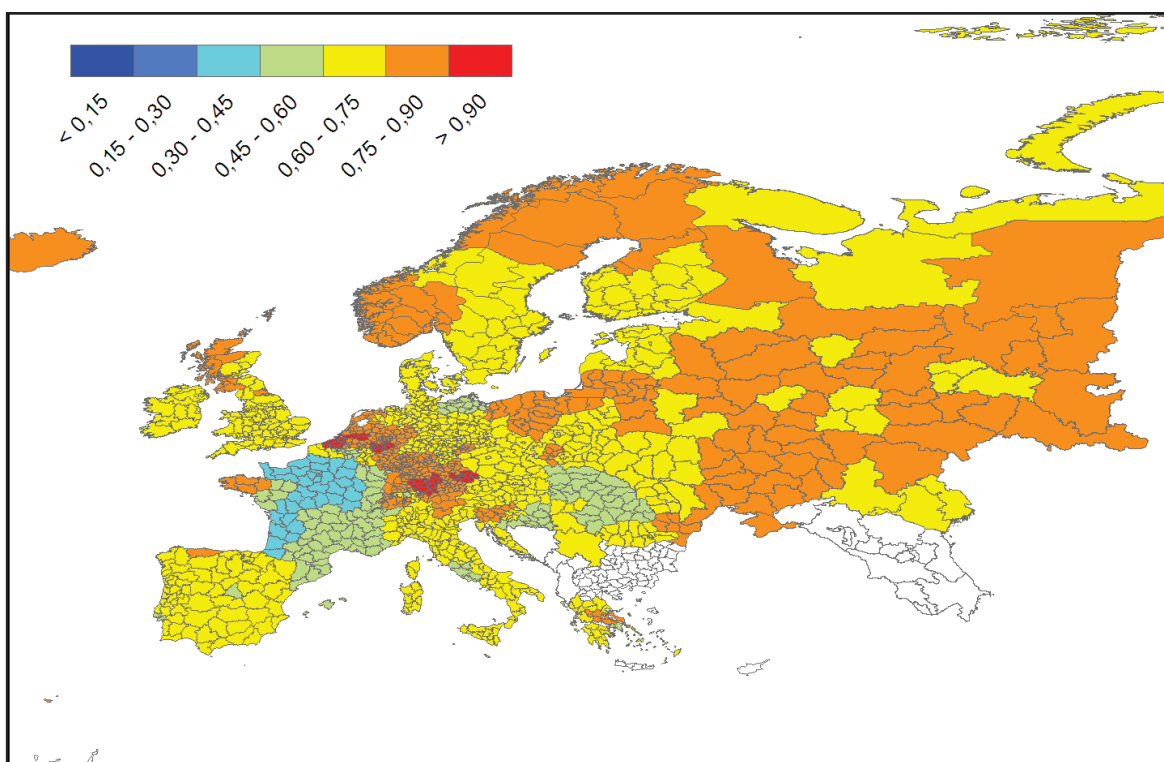
Figure 3.62 Marital fertility, 1870
