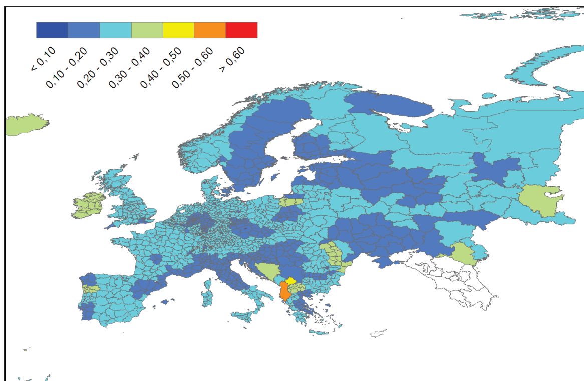
Figure 3.61 Total fertility, 1960
