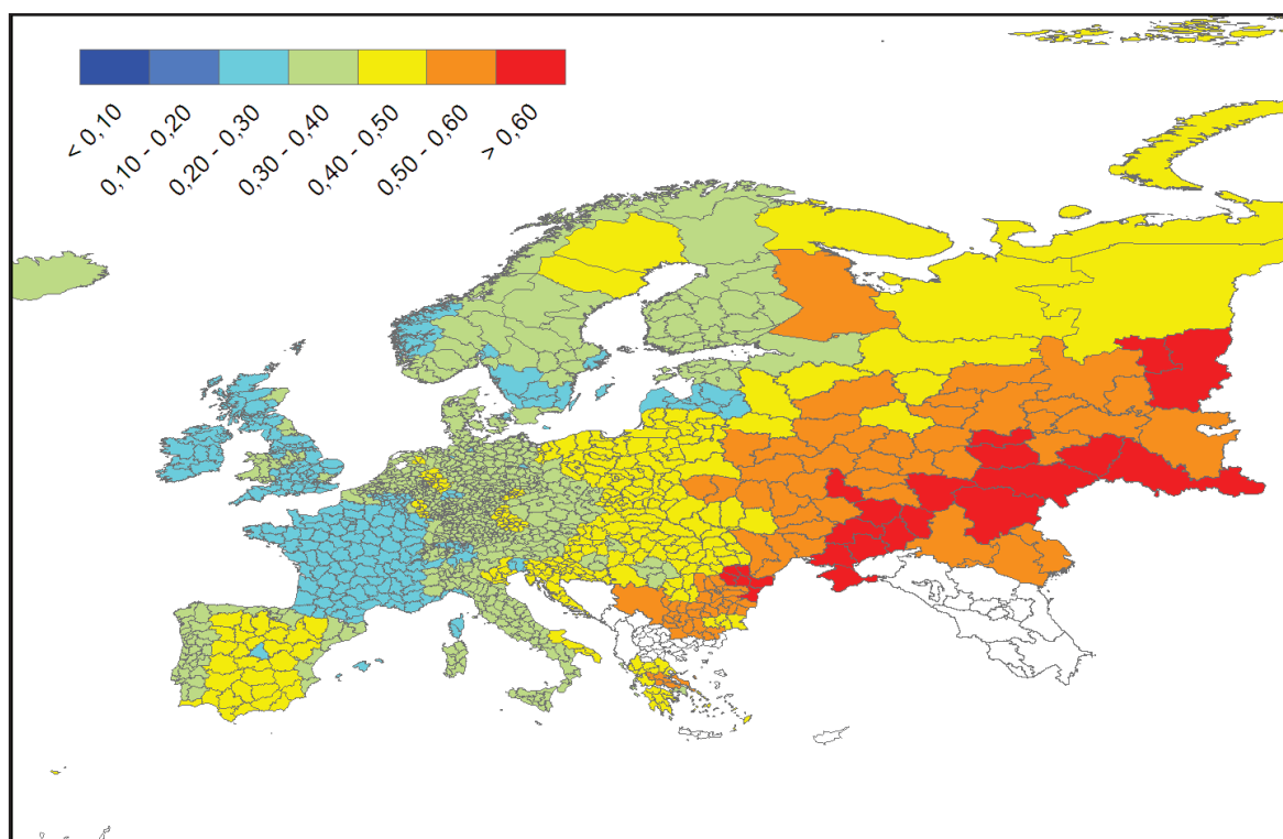
Figure 3.59 Total fertility, 1900
