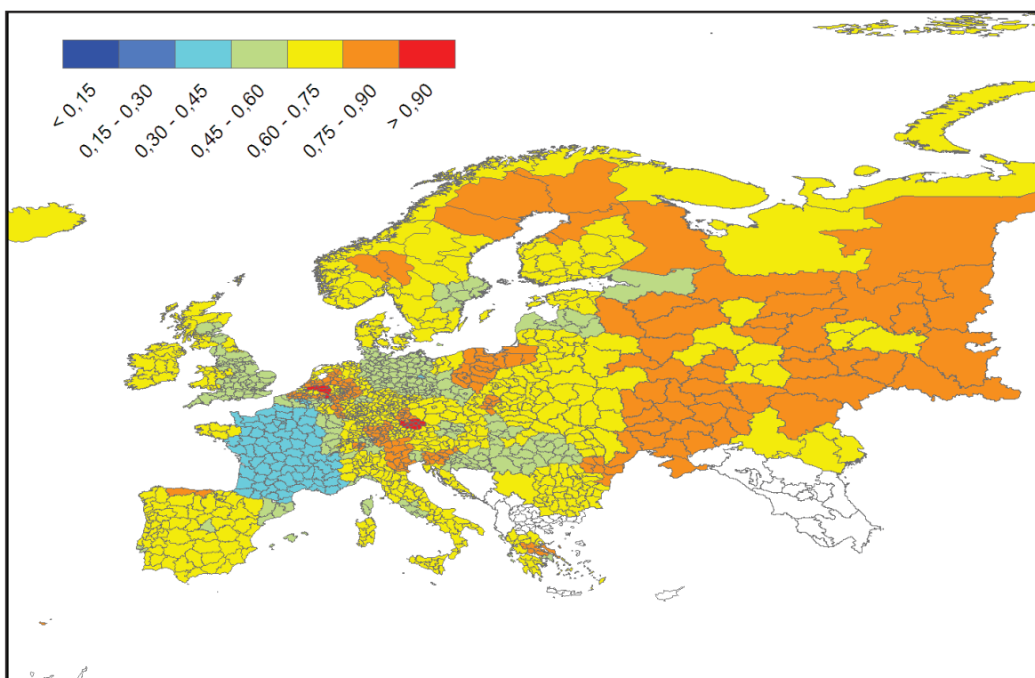
Figure 3.63 Marital fertility, 1900
