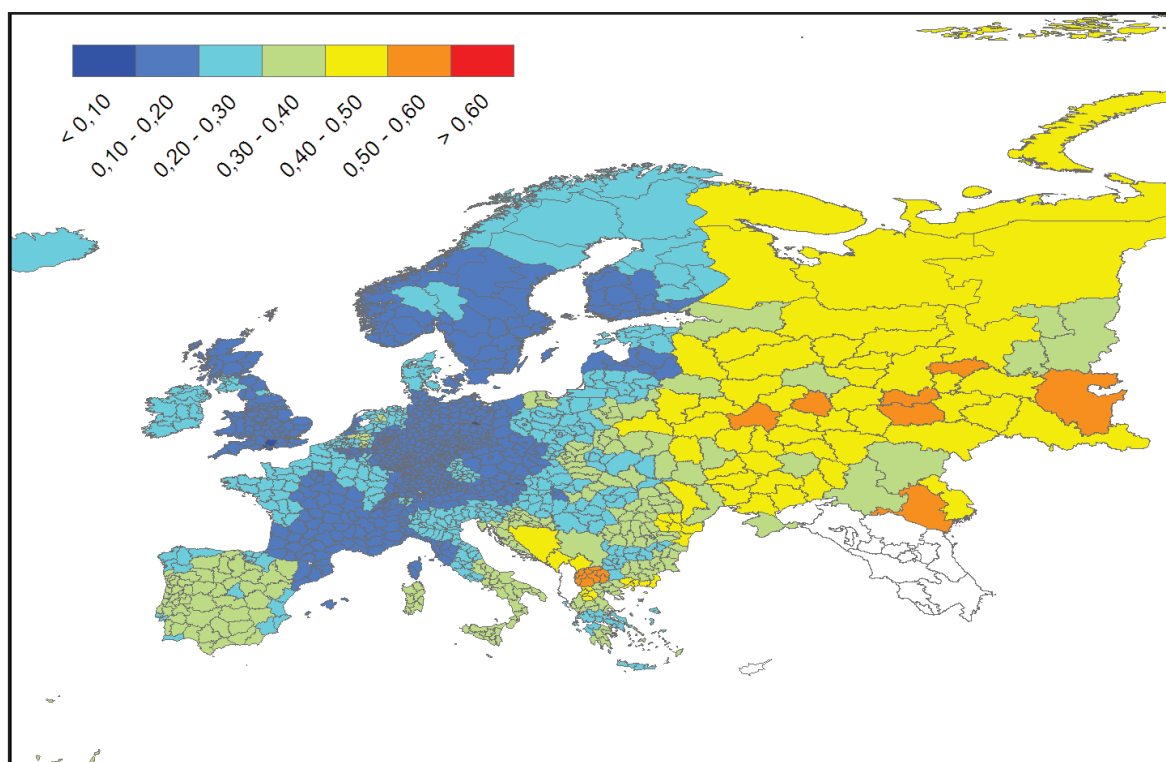
Figure 3.60 Total fertility, 1930
