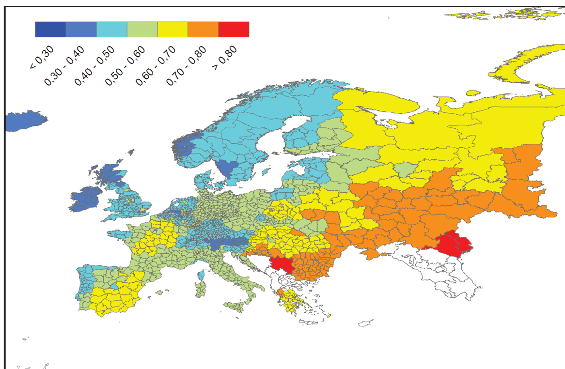
Figure 3.67 Marital status, 1900
