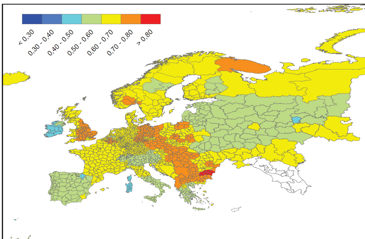
Figure 3.69 Marital status, 1960
