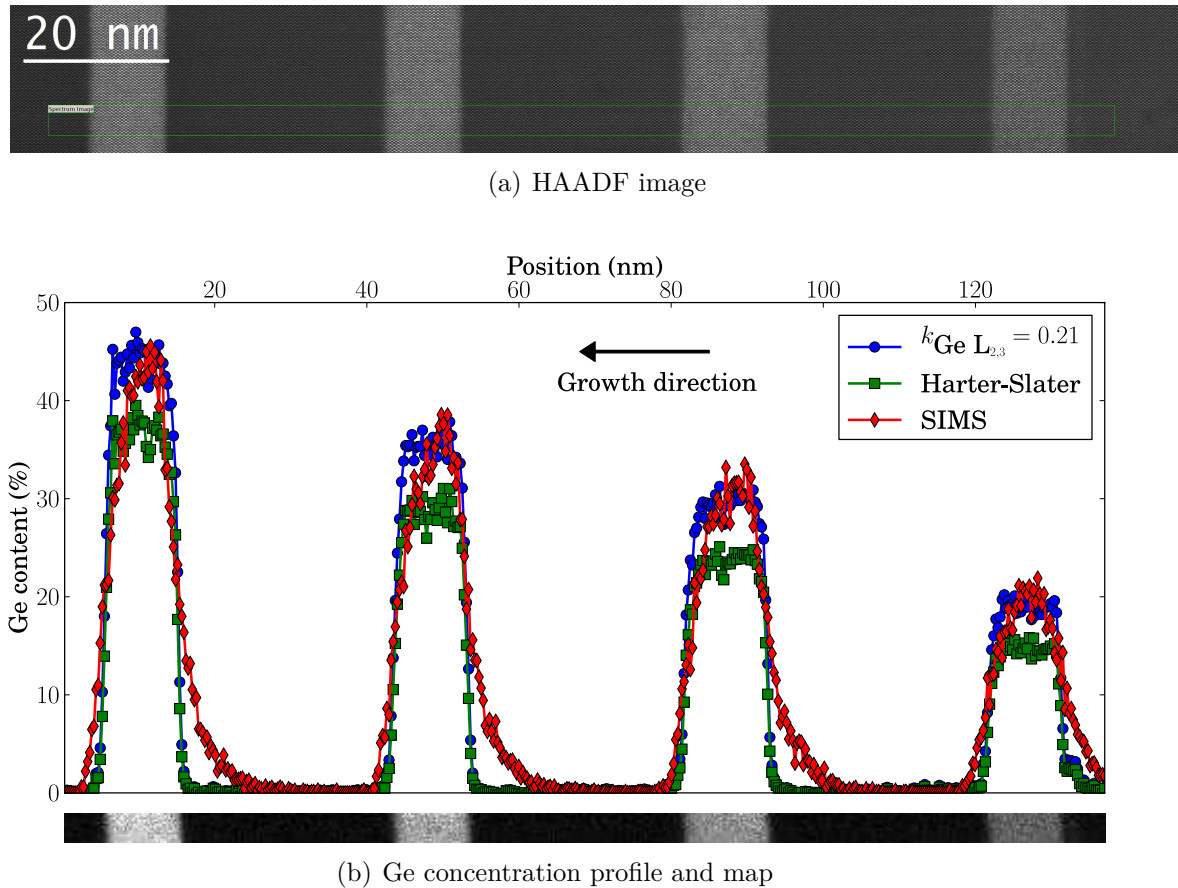
Figure 4.13.: (a) HAADF images of the four SiGe quantum wells indicating the location of the acquired EELS SI (green square) (b) Ge concentration profile and map of four SiGe quantum wells used for the calibration of the k_{\text{Ge } L_{2,3}} factor. The concentration profile obtained by SIMS is plotted in red diamond. The Ge concentration measured by EELS using Hartree-Slater partial cross-section and k_{\text{Ge } L_{2,3}} factor are plotted in green square and blue dots, respectively. The nominal Ge concentration is 45 %, 38 %, 31 % and 20 % from the left to the right.
