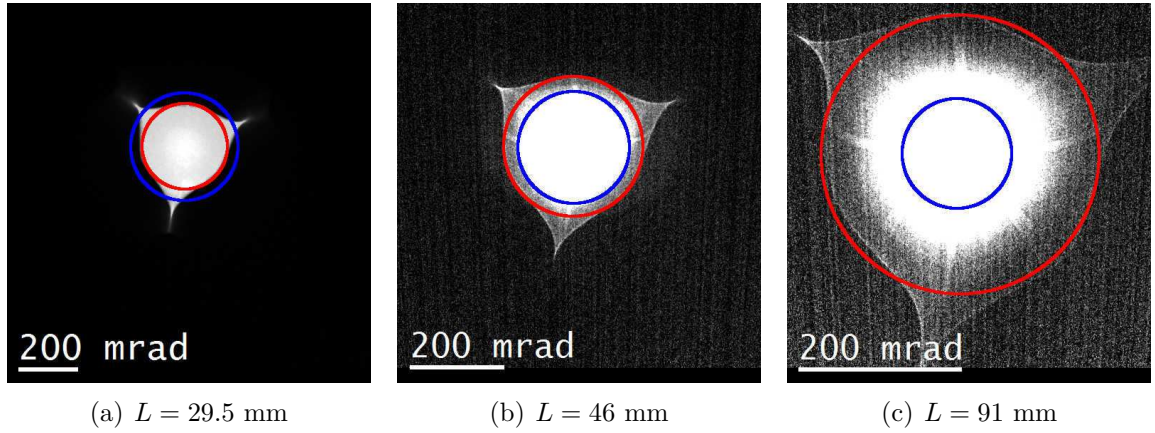
Figure B.1.: Images of the distribution of scattered electrons in the diffraction plane illustrating the dependence of the cut-off of the microscope in STEM mode on the camera length. The images have been acquired using the FEI FluCam camera in diffraction mode for three different camera length: (a) L = 29.5 mm, (b) L = 46 mm and (c) L = 91 mm. The blue and red circles correspond to the inner collection angle of the HAADF detector and the cut-off of the microscope, respectively.
