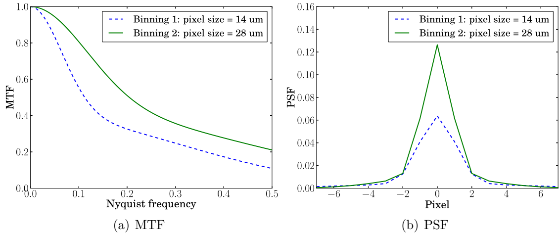
Figure 2.9.: Typical modulation transfer function (MTF) and point spread function of a Gatan Ultrascan CCD camera with two different pixel sizes. The MTF is plotted as a function of the Nyquist frequency, which is defined as the reciprocal value of twice the pixel size.
