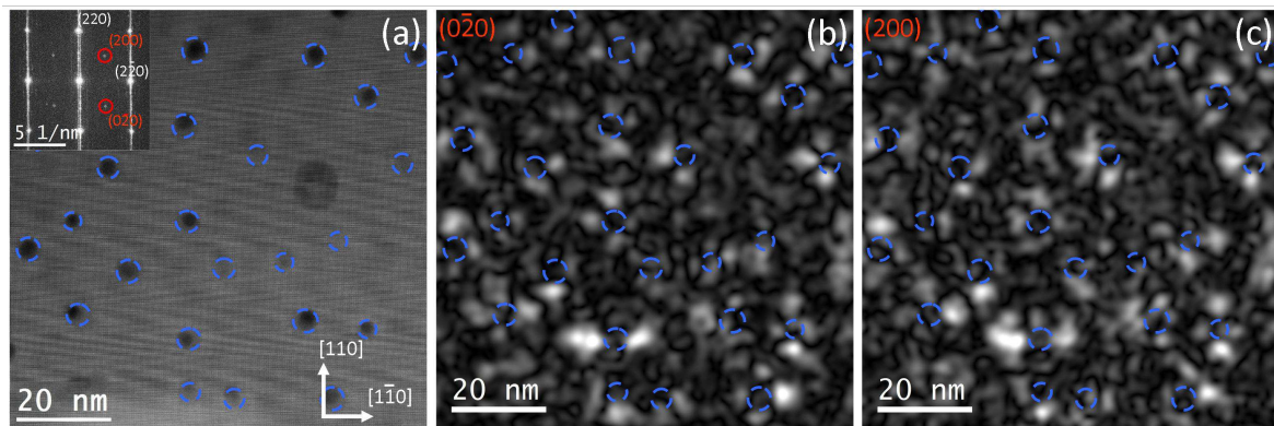
Figure 5.26.: (a) HAADF-HRSTEM image of S2 samples. In the inset of (a) shows the power spectrum of the HAADF images in (a). (b, c) Amplitude of the Fourier component corresponding to the (020) and (200) forbidden Bragg reflections, which are marked by red fill circles in the inset of (a). The blue dashed circle indicated the position of the NCs.
