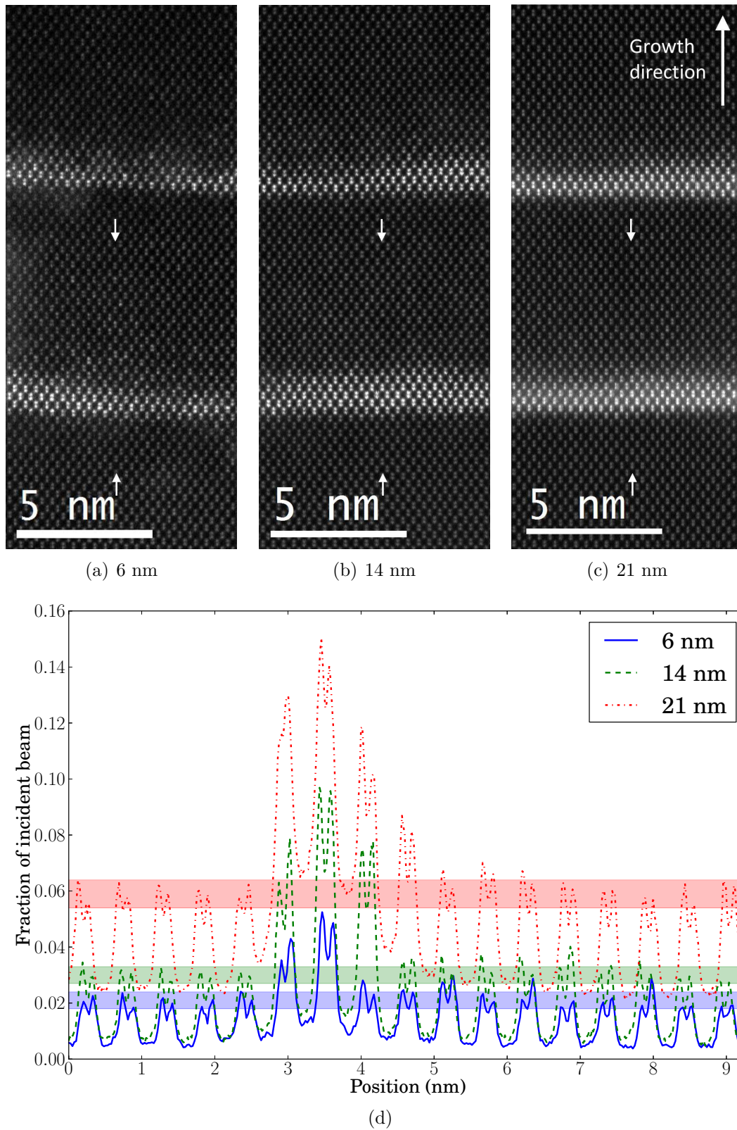
Figure 4.7.: HAADF-STEM images of 4 ML Ge QDs with different thickness: (a) 6 nm, (b) 14 nm and (c) 21 nm. (d) HAADF Intensity profile across the HAADF images of Ge QDs (a-c). The profiles are measured in the area between the two arrows by averaging over narrow width of 1 Å.
