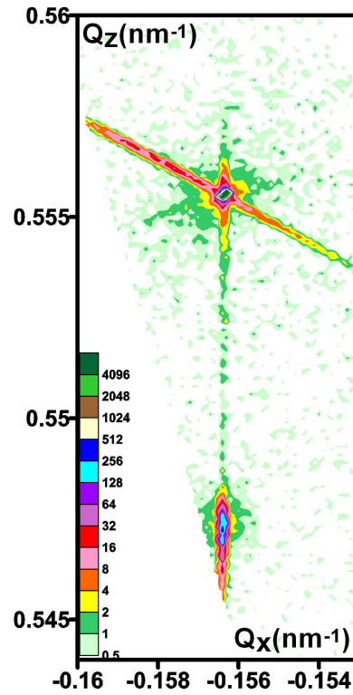
Figure 5.21.: X-ray map around the [1\bar{1}5] Bragg peak of a 250 nm thick \text{Ge}_{0.94}\text{Sn}_{0.06} layer grown on Ge(001).
