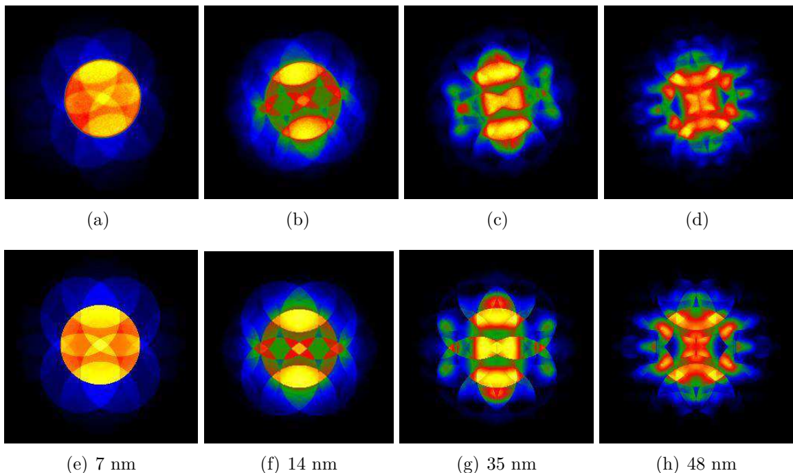
Figure 2.18.: (a-d) Experimental and (e-h) simulated PACBED patterns of Si in [110] -zone axis acquired in STEM mode ( \alpha = 9.2 mrad) at 200 kV for different thicknesses. By comparison of experimental with simulated pattern, the specimen thickness can be determined.
