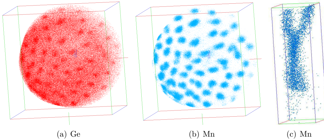
Figure 5.7.: Reconstructed volume of (a) Ge and (b) Mn obtained from APT experiment in top view. The volume in (a-b) are oriented along the growth direction. The position of the GeMn NCs can be recognized by the Mn-rich area in (b). (c) Side view of a junction of two GeMn NCs. Experiment performed by Pierre-Henry Jouneau, Bastien Bonef from CEA INAC and Adeline Grenier from CEA LETI.
