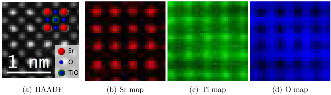
Figure 2.22.: Atomic resolved EELS acquisition of \text{SrTiO}_3 in [001] -zone axis acquired at 200 kV, using 21 mrad convergence angle and 98 mrad collection angle. (a) HAADF images acquired simultaneously and background subtracted map of (b) Sr (c) Ti and (d) O. The current of the 1 Å probe was 140 pA allowing pixel acquisition time of 20 ms with high SNR. The total acquisition time of the EELS data set is 41 s. The specimen thickness t = 27 nm is estimated with the relative specimen thickness t/\lambda = 0.33 .
