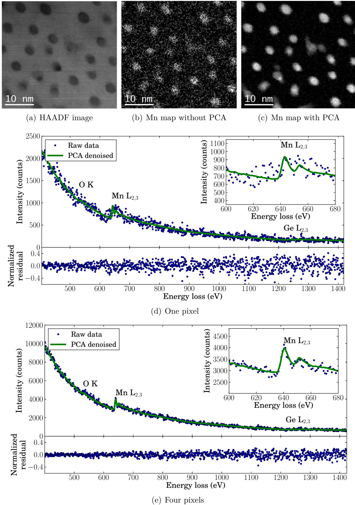
Figure 5.3.: Effect of PCA treatment on the computing of EELS data set. (a) HAADF image acquired simultaneously than the EELS signal. Mn maps obtain from (b) the raw EELS SI and (c) after PCA denoising. Comparison of EELS spectra measured in a GeMn nanocolumns before and after PCA denoising for two cases: (d) signal of one individual pixel and (e) signal summed over 4 pixels. Four components were used for the PCA denoising.
