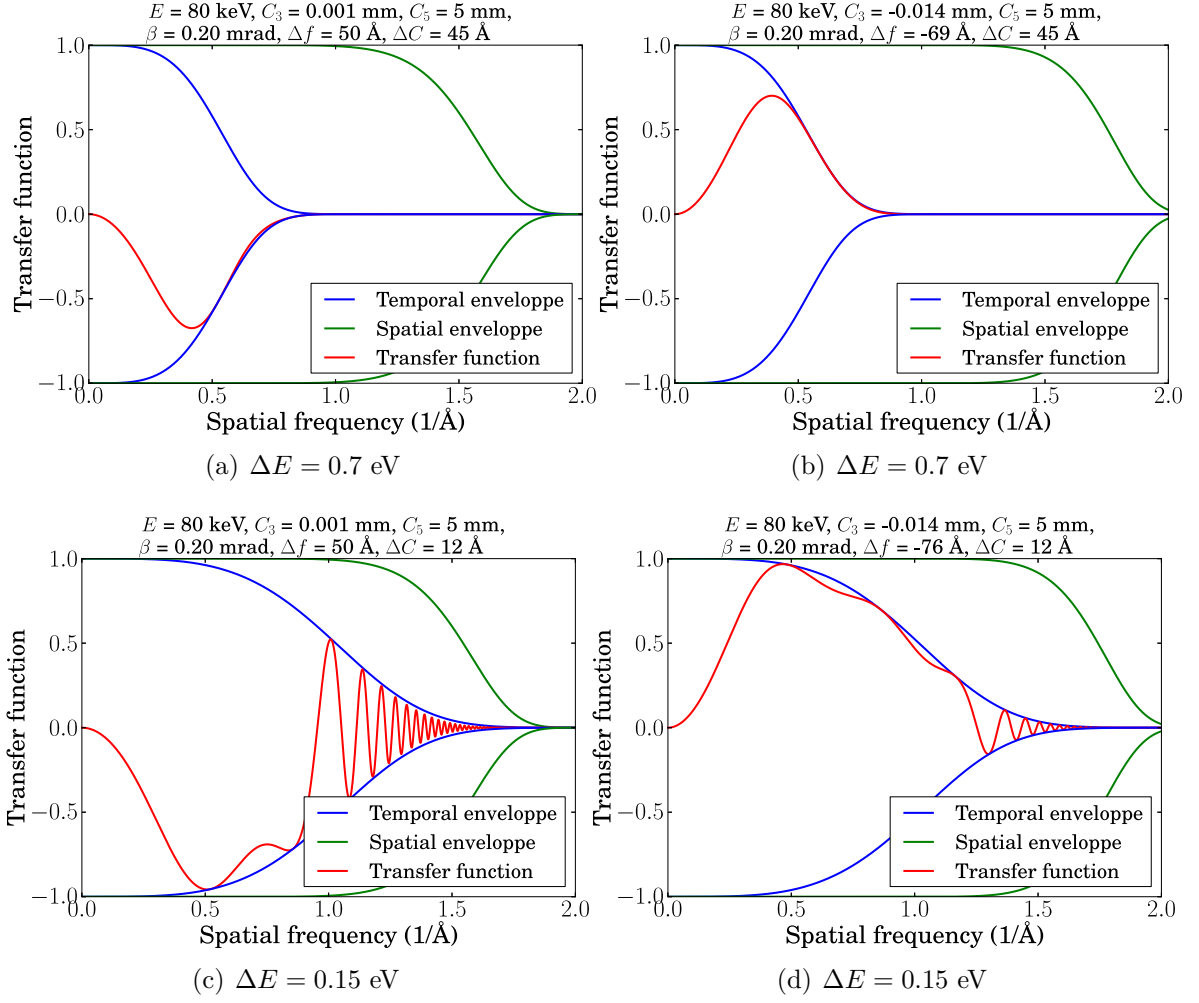
Figure 2.10.: Comparison of PCTF at 80 kV: (a-b) \Delta E = 0.7 eV and (c-d) \Delta E = 0.15 eV. In (b) and (d), the C_3 coefficient has been optimized.
