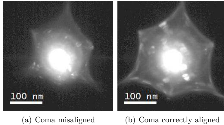
Figure 2.7.: Coma alignment of the image corrector. The shadow in the image correspond the cut-off of the microscope. In (a) the transmitted beam is not centered in the corrector, whereas in (b) the centering is fine. The image intensity is shown on a non linear scale.
