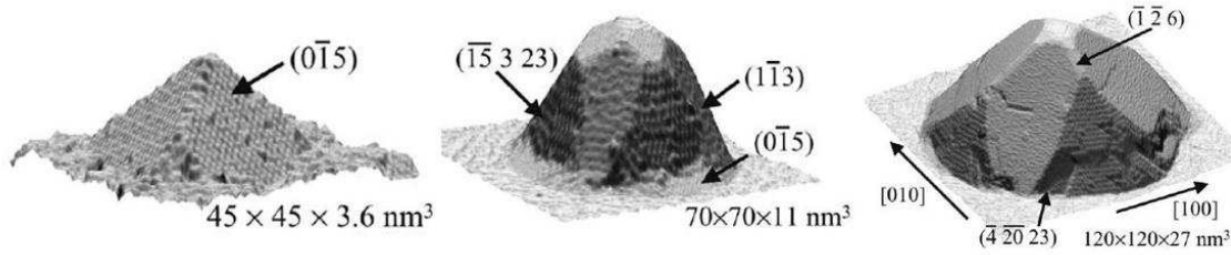
Figure 4.5.: Typical evolution of Ge QDs on Si(001) as observed by scanning tunneling microscopy (STM) topograph of Ge quantum dots on Si(001). The shape of the Ge quantum dots changes with increasing its size. At small size \{105\} faceted pyramids with square base (a) are formed and with increasing the size additional \{113\} and \{102\} facets are created in the dome (b). Plastically deformed super-dome are finally formed with misfit dislocation(c). Note that the figures are stretched along the growth direction to highlight the facets. Taken from [Duja 06].
