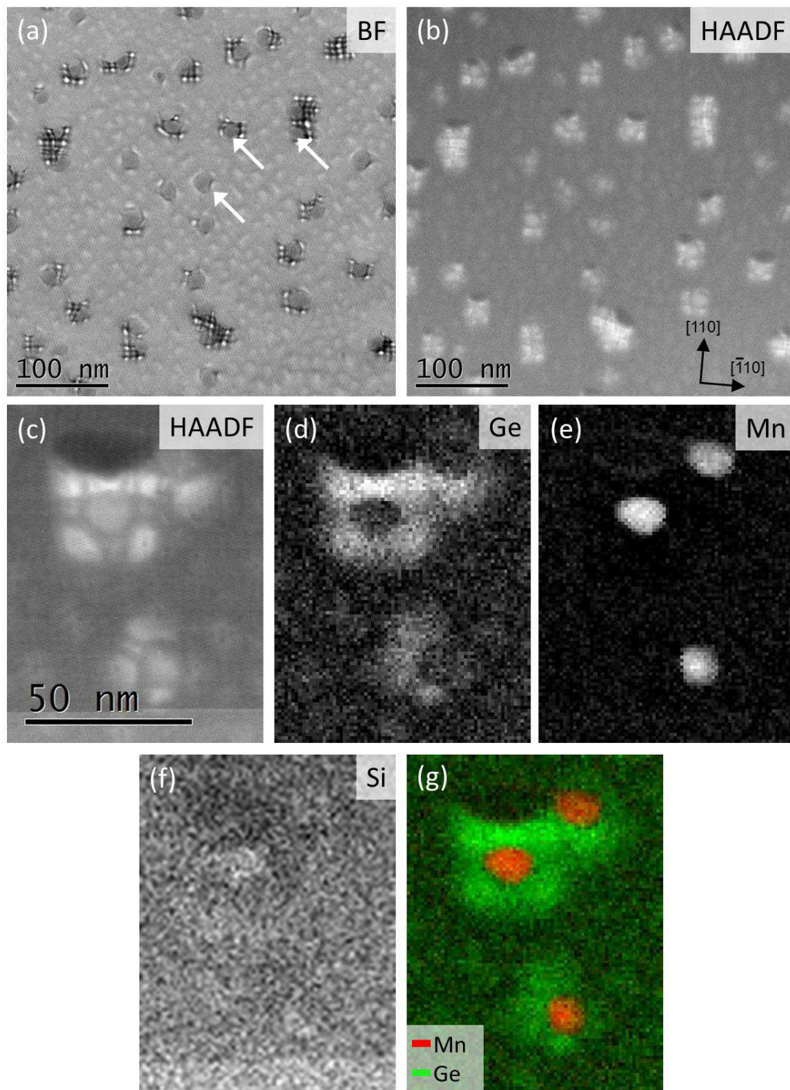
Figure 4.27.: (a) BF- and (b) HAADF-STEM images in the [001] -zone axis of one Ge(Mn) QDs layer grown on Si substrate. (c-f) Plane-view EELS analysis of two Ge(Mn) QDs. (c) HAADF-STEM image acquired simultaneously than the EELS SI. (d) Ge map (e) Mn map and (f) Si map obtained from the EELS SI. (g) Ge (green) versus Mn (red) composite map. PCA denoising was performed with three components.
