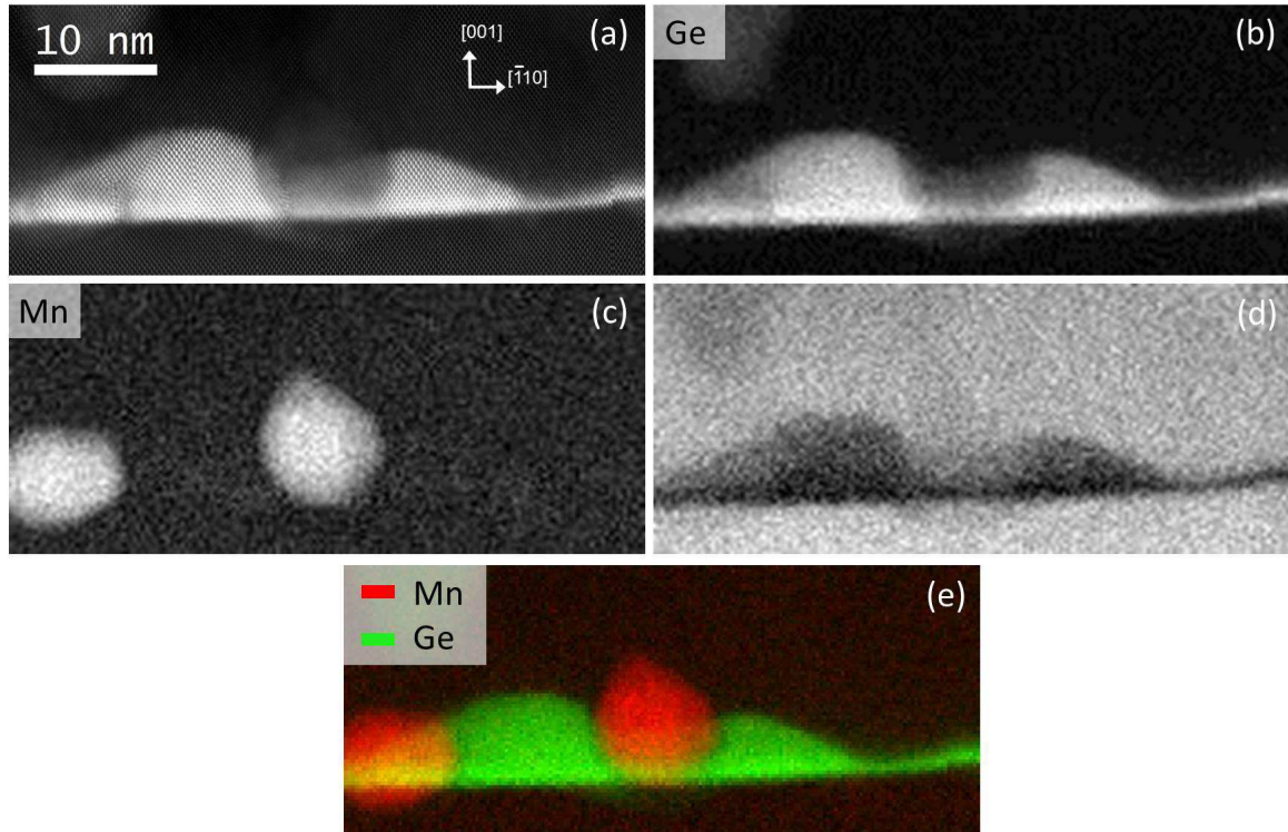
Figure 4.26.: Cross-section EELS analysis a Ge(Mn) QD. (a) HAADF-HRSTEM images in the [110] -zone axis acquired simultaneously than the EELS SI. (b) Ge map, (c) Mn map and (d) Si map obtained from the EELS SI. Ge (green) versus Mn (red) composite map. PCA denoising was performed with five components.
