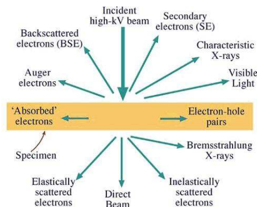
Figure 2.1.: Schematic illustration of the different signals, that can be generated after interaction of a high energy incident electron beam with the specimen in TEM. Taken from [Will 09] .
