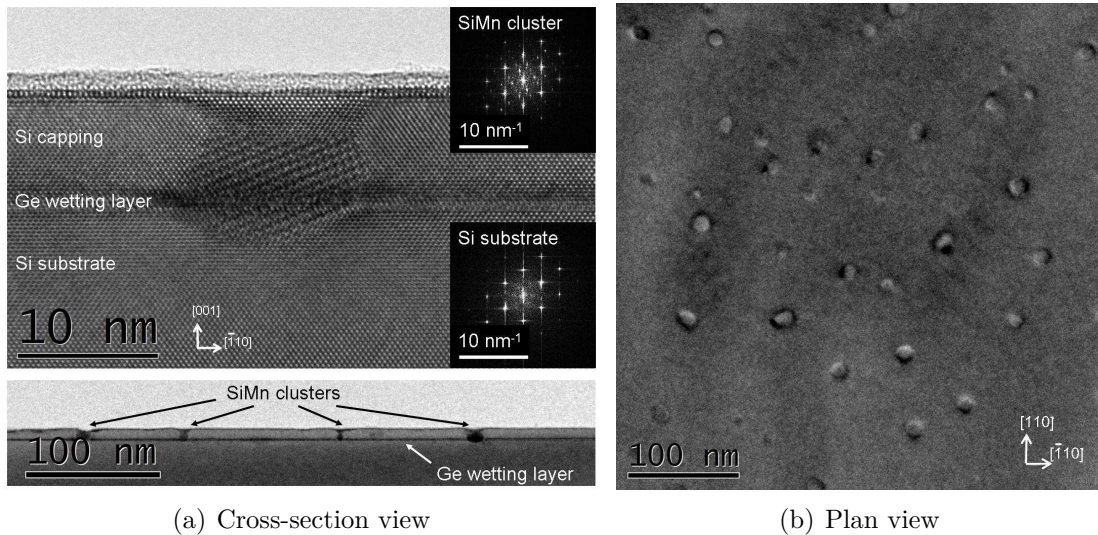
Figure 4.29.: HRTEM observations of an unique GeMn WL. (a) Cross-section view images in [110]-zone axis showing SiMn precipitates, which can be recognized with the Moiré pattern on the top HRTEM image. The dark area on the bottom bright-field TEM image correspond to the Moiré pattern. The FFT of SiMn precipitates and the Si substrate are displayed in the insets. (b) Plan-view bright-field TEM image acquired in the [001]-zone axis shows the in-plane distribution of SiMn precipitates.
