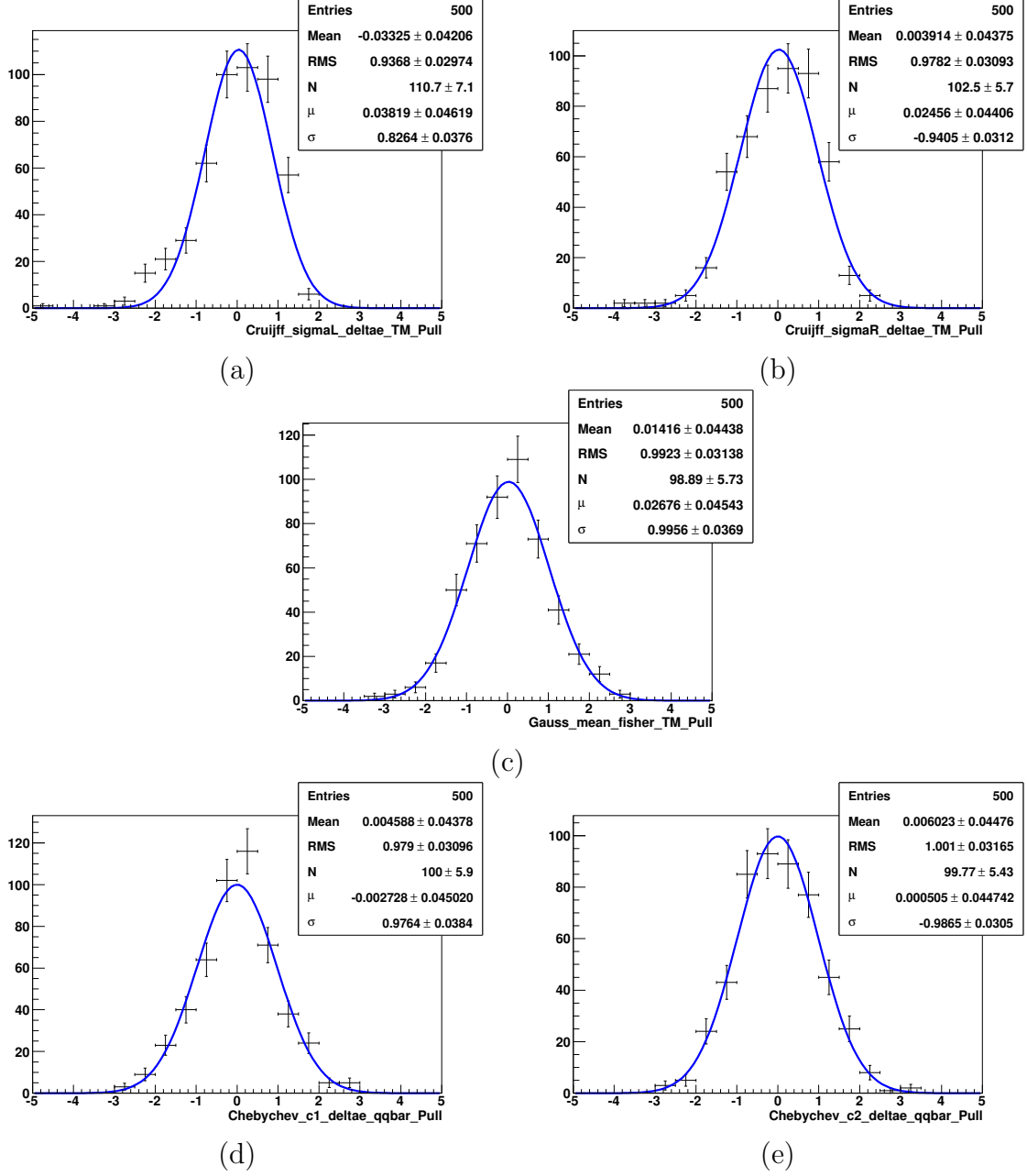
Figure G.3: Pull distributions of signal TM \Delta E Cruijff and the Fisher discriminant Gaussian parameters: \text{Cr}_{\sigma_L} (a), \text{Cr}_{\sigma_R} (b) and G_\mu (c), as well as the continuum background Fisher discriminant Chebychev polynomial parameters: \text{Chebychev}_{c_1} (d), \text{Chebychev}_{c_2} (e) for the pure toy studies with 500 toys.
