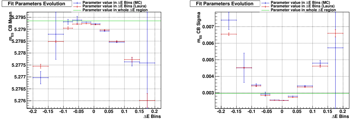
Figure 6.14: m_{\text{ES}} Crystal Ball \mu (left) and \sigma (right) parameters evolution in \Delta E bins. Blue points correspond to MC sample, red points to a toy sample generated using the two-dimensional conditional PDF, and the green horizontal line corresponds to a 1-dimensional Crystal-Ball PDF without m_{\text{ES}}\text{-}\Delta E correlations. The central value of each point is the fitted value of the Crystal Ball parameter, the vertical error bars correspond to the parameter fit error and the horizontal error bars to the size of each \Delta E bin.
