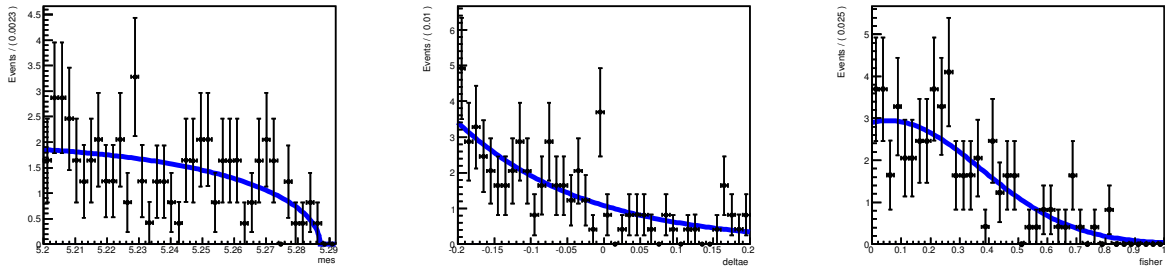
Figure 7.13: PDFs of B^0 \bar{B}^0 generic background category. Conventions are similar to those of Fig. 7.8. Here the m_{\text{ES}} PDF is described by an Argus, the \Delta E PDF by a second order Chebychev polynomial function and the Fisher discriminant PDF is described by a Gaussian function.
