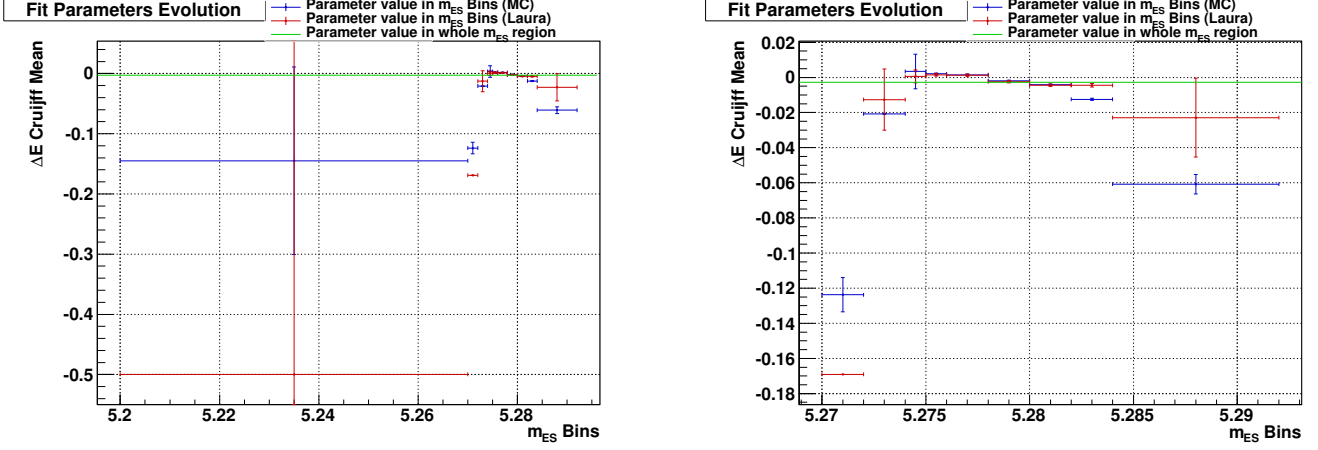
Figure D.1: \Delta E Cruijff \mu parameter evolution in m_{ES} bins, in the whole m_{ES} range (left) and excluding m_{ES} bin0 (right). Blue points correspond to MC sample, red points correspond to generated sample using our two-dimensional conditional PDF, and the green horizontal line corresponds to the uni-dimensional Cruijff initial PDF. The central value of each point corresponds to the fitted value of the Cruijff parameter, the vertical error bars correspond to the parameter fit error given by MINUIT and the horizontal error bars define the size of each \Delta E bin.
