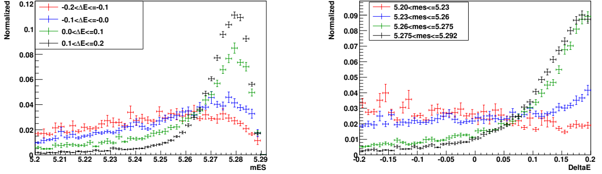
Figure 7.16: m_{\text{ES}} (left) and \Delta E (right) distributions of B^+ \rightarrow K^{*+}(\rightarrow K_s^0 \pi^+) \gamma + B^+ \rightarrow X_{su}(\rightarrow K_s^0 \pi^+) \gamma events in \Delta E and m_{\text{ES}} bins, respectively
