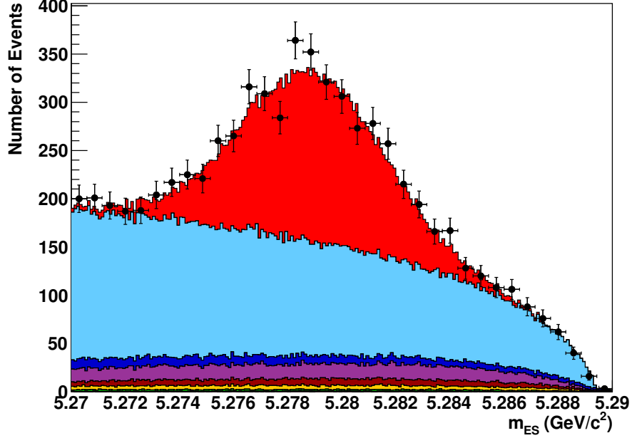
Figure F.2: m_{\text{ES}} fit projection in the signal region, where the following cuts have been applied in order to enrich the data sample in signal events: -0.15 \leq \Delta E \leq 0.10 \text{ GeV}/c and m_{\text{ES}} > 5.27 \text{ GeV}/c^2 . Conventions are identical to those in Fig. F.1
