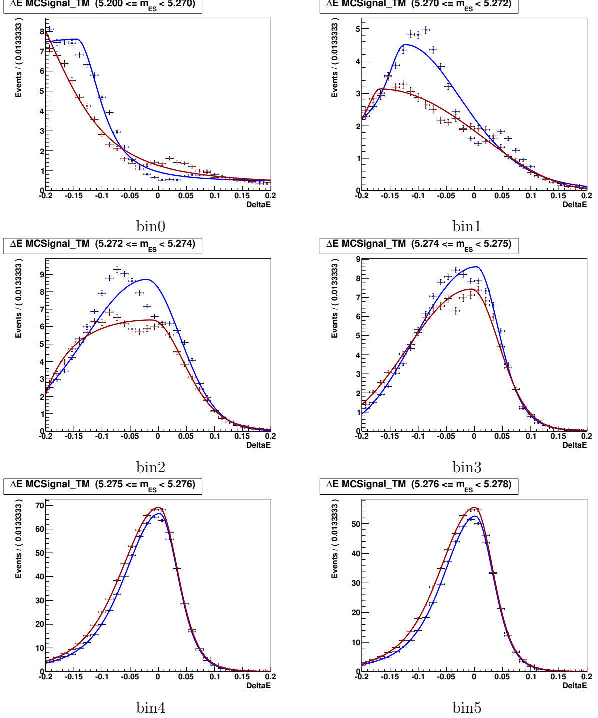
Figure D.8: \Delta E Cruijff fit projection in m_{\text{ES}} bins 0 to 5. Blue curve correspond to MC sample, red curve correspond to generated sample using our two-dimensional conditional PDF.
