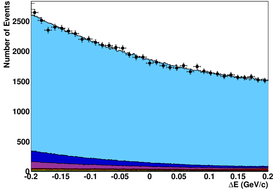
Figure F.6: \Delta E fit projection in m_{\text{ES}} bin 0.
