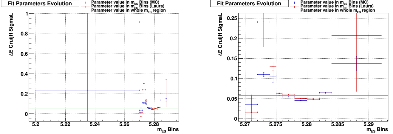
Figure D.2: \Delta E Cruijff \sigma_l parameter evolution in m_{ES} bins, in the whole m_{ES} range (left) and excluding m_{ES} bin0 (right). Conventions are identical as those used in Fig. D.1.
