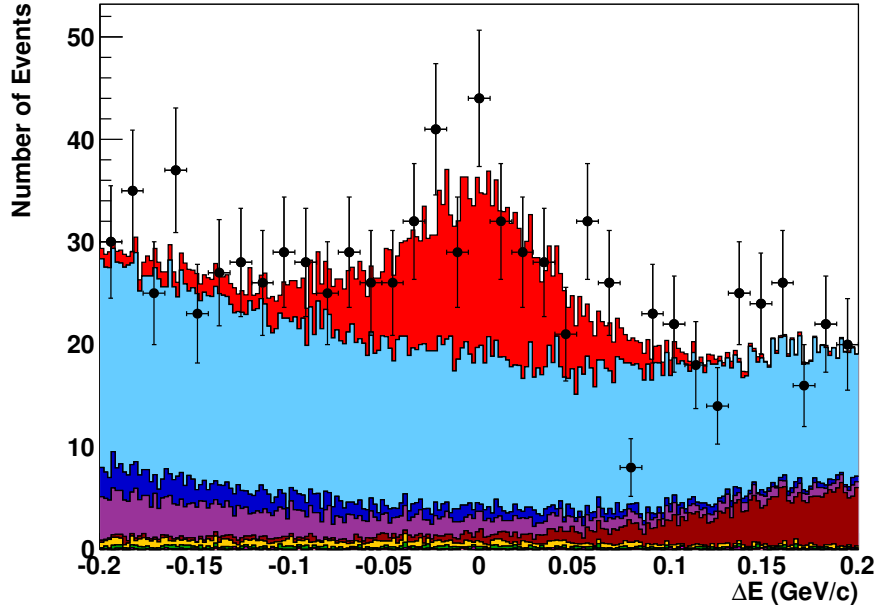
Figure F.10: \Delta E fit projection in m_{\text{ES}} bin 4.
