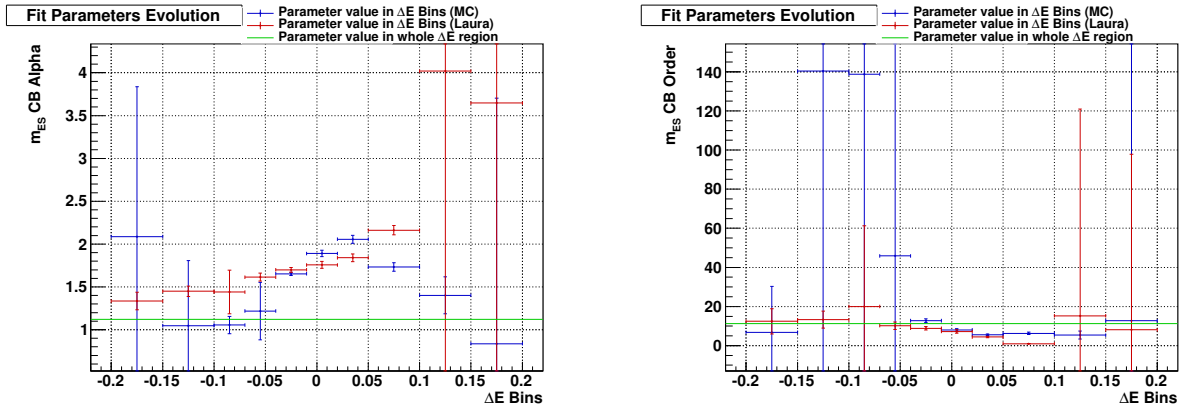
Figure 6.15: m_{\text{ES}} Crystal Ball \alpha (left) and n (right) parameters evolution in \Delta E bins. Conventions are identical as those of Fig. 6.14.
