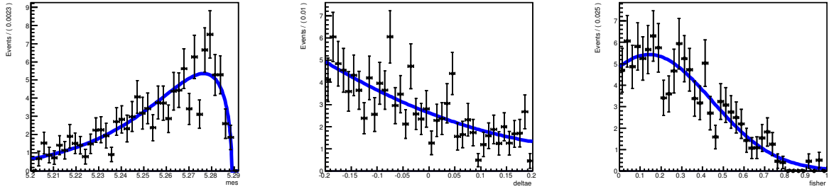
Figure 7.9: PDFs of B^+ \rightarrow X_{su}(\rightarrow K\pi)\gamma B -background category. Conventions are similar to those of Fig. 7.8. Here the m_{\text{ES}} PDF is described by an Argus, the \Delta E PDF by a second order Chebychev polynomial and the Fisher discriminant by a Gaussian function.
