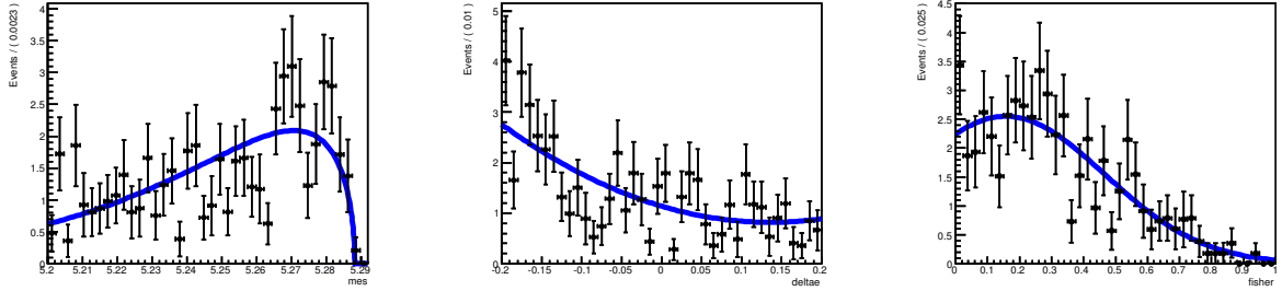
Figure 7.12: PDFs of B^0 \rightarrow X_{sd}(\rightarrow K\pi)\gamma + B^+ \rightarrow X_{su}(\rightarrow K\pi)\gamma background category. Conventions are similar to those of Fig. 7.8. Here the m_{\text{ES}} PDF is described by a Crystal Ball function, the \Delta E PDF by a Cruijff function and the Fisher discriminant PDF is described by a Gaussian function.
