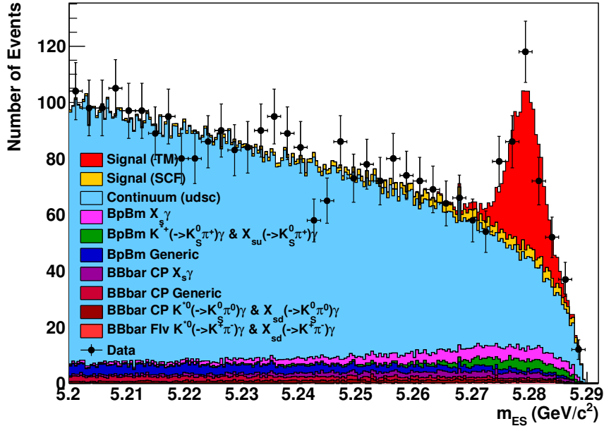
Figure 7.21: m_{\text{ES}} fit projection. Black points describe data events and the full colored histograms describe the contribution of each event species in the model.
