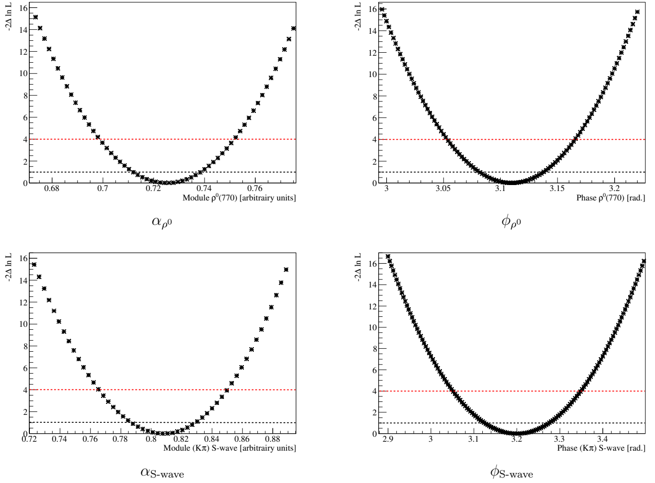
Figure 6.45: One-dimensional scans of -2\Delta\ln\mathcal{L} as a function of the magnitudes of \rho^0(770) and (K\pi) S-wave and the phase of \rho^0(770) . The horizontal dashed lines mark the one- and two-standard deviation levels.
