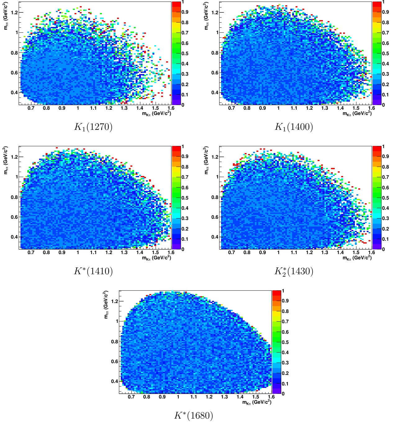
Figure 6.38: Two-dimensional ( m_{K\pi} , m_{\pi\pi} ) efficiency maps for each resonance contributing to the signal. In the upper right side of each map, some bins present efficiency close to one. This is due to the very low density of events in these bins, and to event migration.
