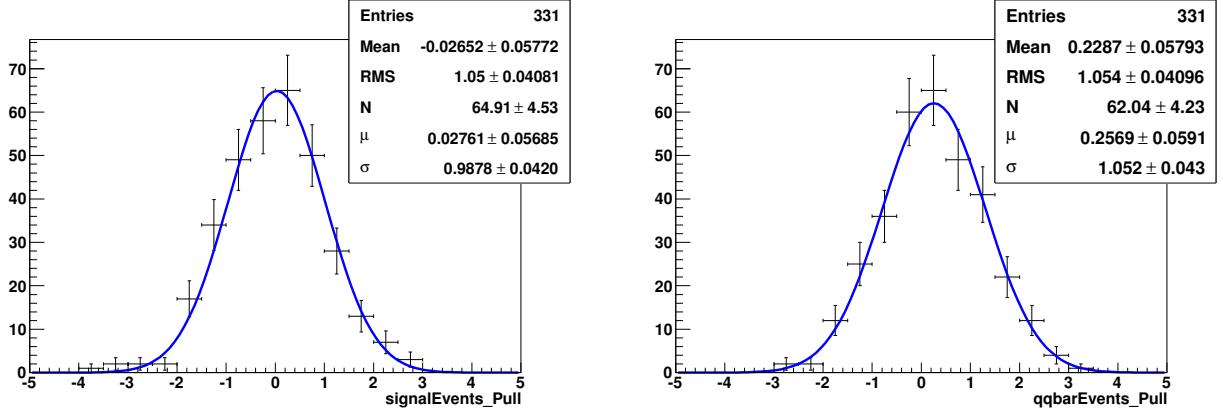
Figure 6.29: Signal-TM (left) and continuum udsc (right) yield pull distributions for the embedded toy studies with 331 toys, respectively.
