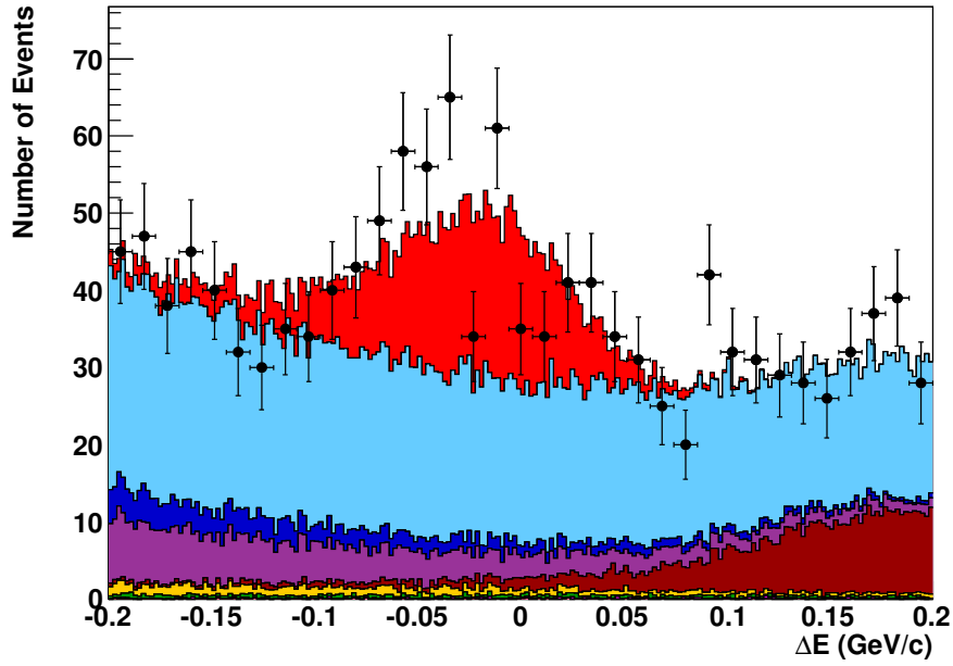
Figure F.14: \Delta E fit projection in m_{\text{ES}} bin 8.
