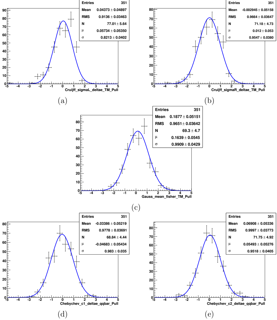
Figure G.7: Pull distributions of signal TM \Delta E Cruijff and the Fisher discriminant Gaussian parameters: Cr_{\sigma_L} (a), Cr_{\sigma_R} (b) and G_\mu (c), as well as the continuum background Fisher discriminant Chebychev polynomial parameters: Chebychev_{c1} (d), Chebychev_{c2} (e) for the embedded toy studies with 351 toys.
