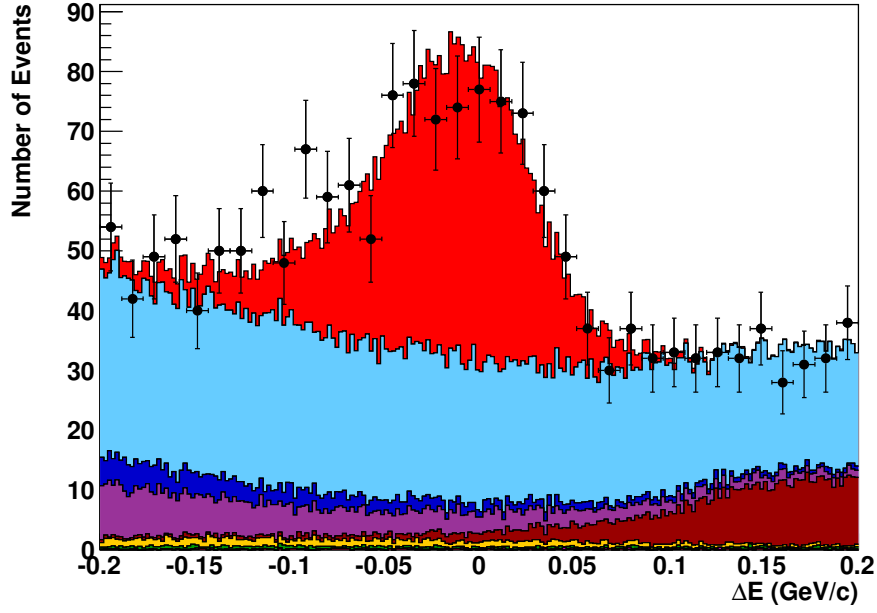
Figure F.13: \Delta E fit projection in m_{\text{ES}} bin 7.
