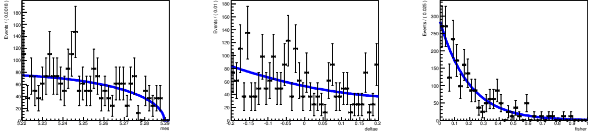
Figure 7.8: Probability density functions for the fit variables m_{\text{ES}} (left), \Delta E (center) and the Fisher discriminant (right) of continuum ( udsc ) background category. The blue curves represent the PDF distributions, and the black points correspond to MC events. Here the m_{\text{ES}} PDF is described by an Argus, the \Delta E PDF by a second order Chebychev polynomial and the Fisher discriminant by an exponential.
