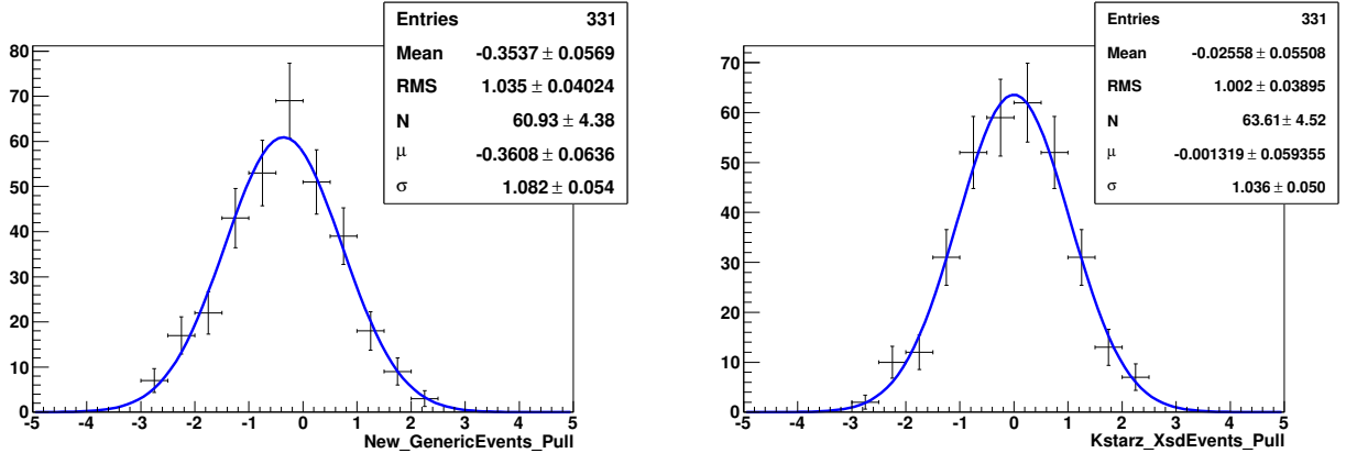
Figure 6.30: Generic B background (left) and B^0 \rightarrow K^{*0}(\rightarrow K\pi)\gamma + B^0 \rightarrow X_{sd}(\rightarrow K\pi)\gamma (right) yield pull distributions for the embedded toy studies with 331 toys, respectively.
