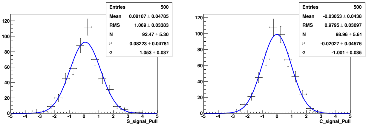
Figure 7.19: Signal \mathcal{S} (left) and \mathcal{C} (right) pull distributions for the pure toy studies with 500 toys.
