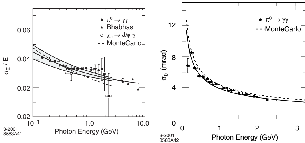
Figure 4.8: Photon energy (left) and angular (right) resolutions achieved by the electromagnetic calorimeter [? ].
