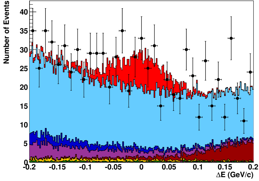
Figure F.9: \Delta E fit projection in m_{\text{ES}} bin 3.
