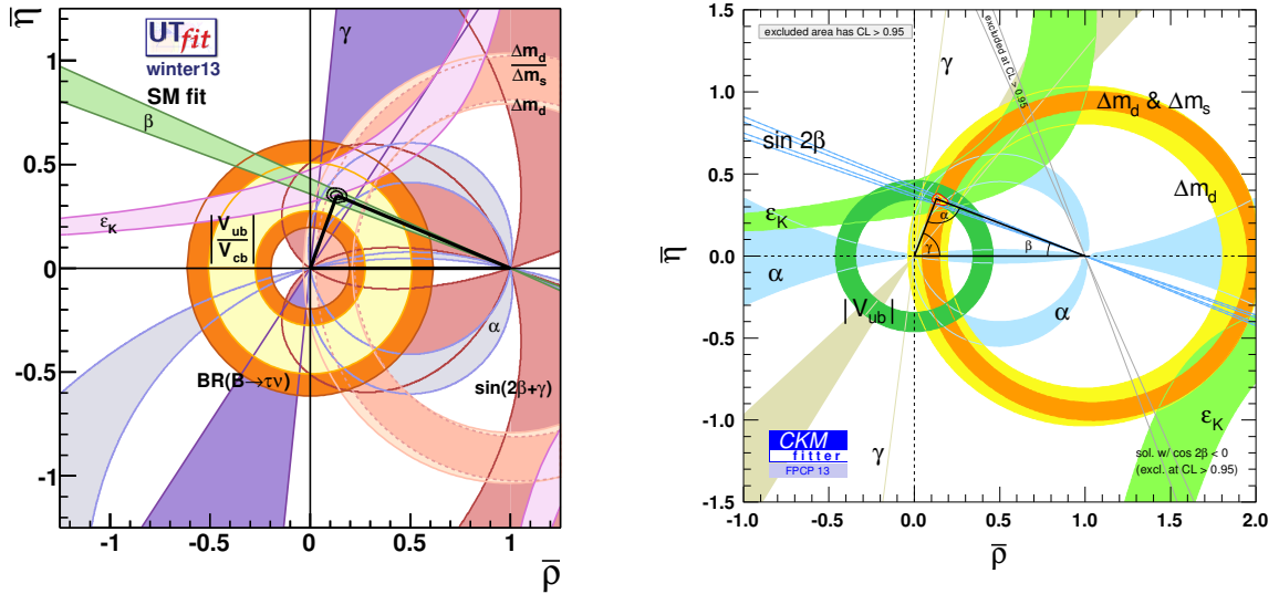
Figure 1.2: Pictorial representation of the current experimental constraints on the sides and angles of the unitarity triangle, by the CKMfitter group [?] (right), updated with the results available in spring 2013, and by the UTFit group [?] (left) updated with the results available in winter 2013. The bands representing each experimental measurement or bound are seen to be in very good agreement with each other, all of them overlapping around the apex of the triangle drawn.
