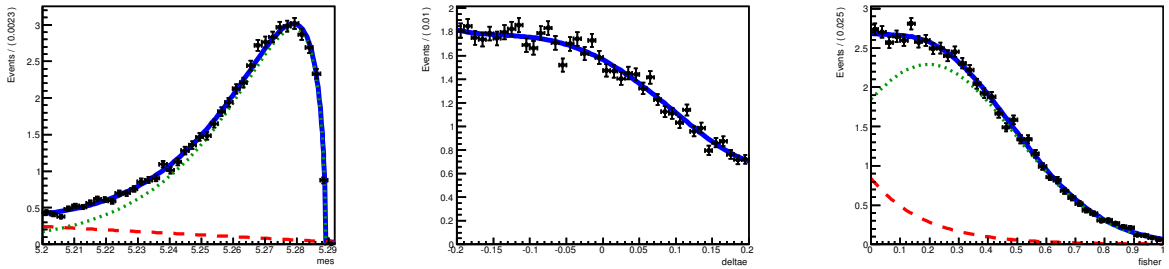
Figure 7.5: Probability density functions for the fit variables m_{\text{ES}} (left), \Delta E (center) and the Fisher discriminant (right) of signal SCF events. Here the m_{\text{ES}} PDF is described by the sum of a first order Chebychev polynomial (red dashed line) and an Argus function (green dotted line), the \Delta E PDF by a fourth order Chebychev polynomial and the Fisher discriminant PDF by the sum of a Gaussian (green dotted line) and an exponential (red dashed line). The blue curves represent the PDF distributions, and the black points correspond to MC events.
