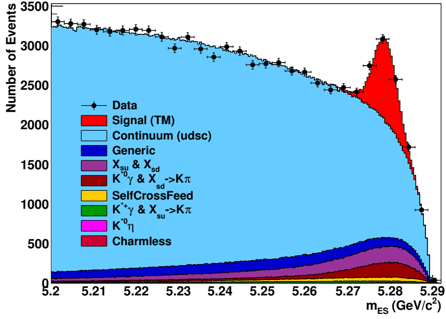
Figure F.1: m_{\text{ES}} fit projection in the whole fit region.
