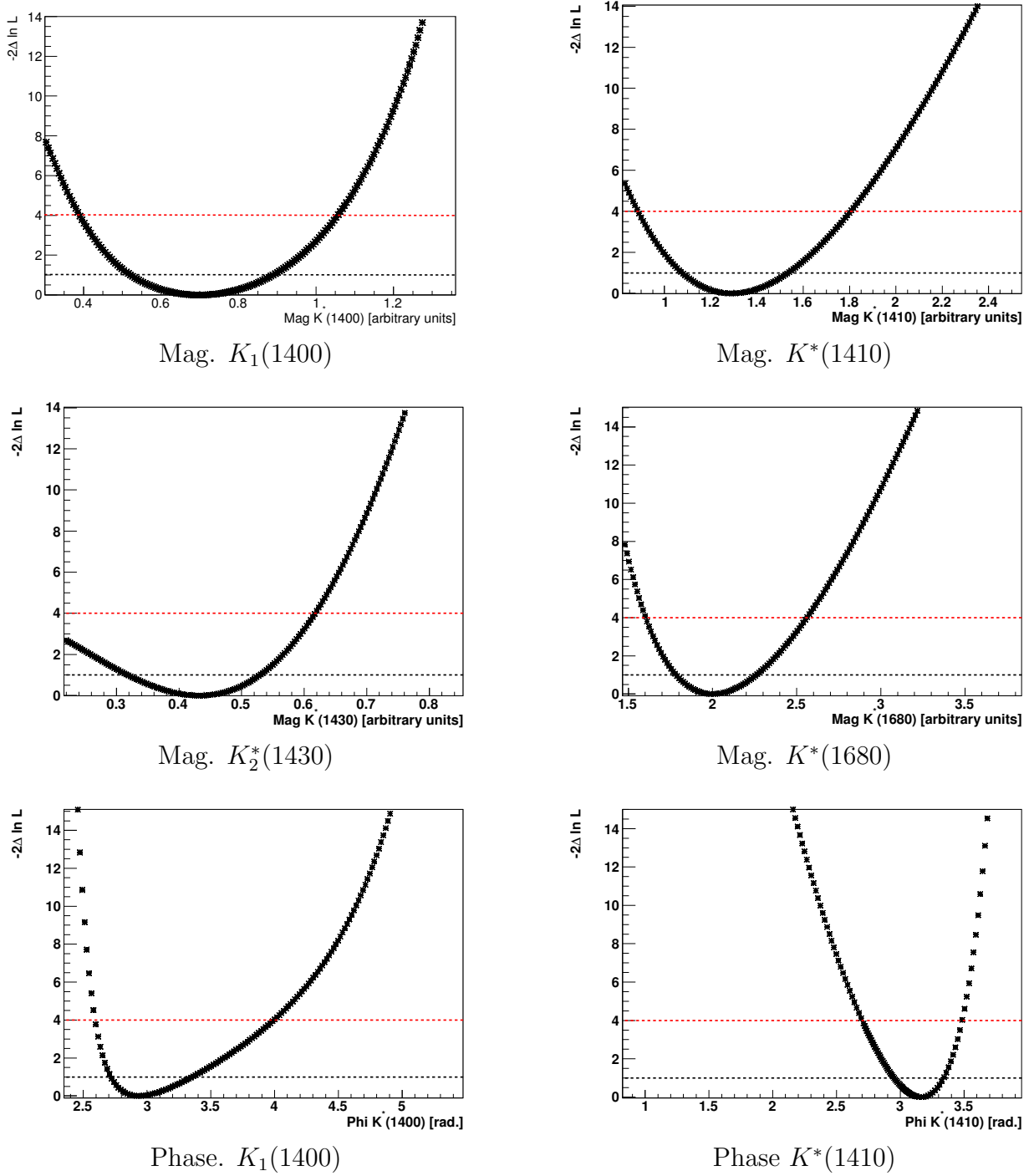
Figure 6.37: One-dimensional scans of -2\Delta\ln\mathcal{L} as a function of magnitudes (top and middle) and phases (bottom). The horizontal dashed lines mark the one- and two-standard deviation levels.
