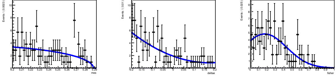
Figure 7.11: PDFs of B^+ B^- generic B -background category. Conventions are similar to those of Fig. 7.8. Here the m_{\text{ES}} PDF is described by an Argus, the \Delta E PDF by a second order Chebychev polynomial function and the Fisher discriminant by a Gaussian function.
