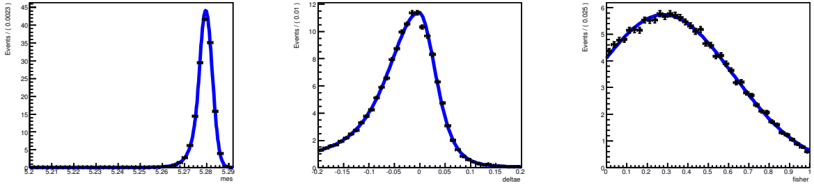
Figure 7.4: Probability density functions for the fit variables m_{\text{ES}} (left), \Delta E (center) and the Fisher discriminant (right) of signal-TM events. Here the m_{\text{ES}} PDF is described by a Crystal Ball function, the \Delta E PDF by a Cruijff function and the Fisher discriminant PDF by a Gaussian. The blue curves represent the PDF distributions, and the black points correspond to MC events.
