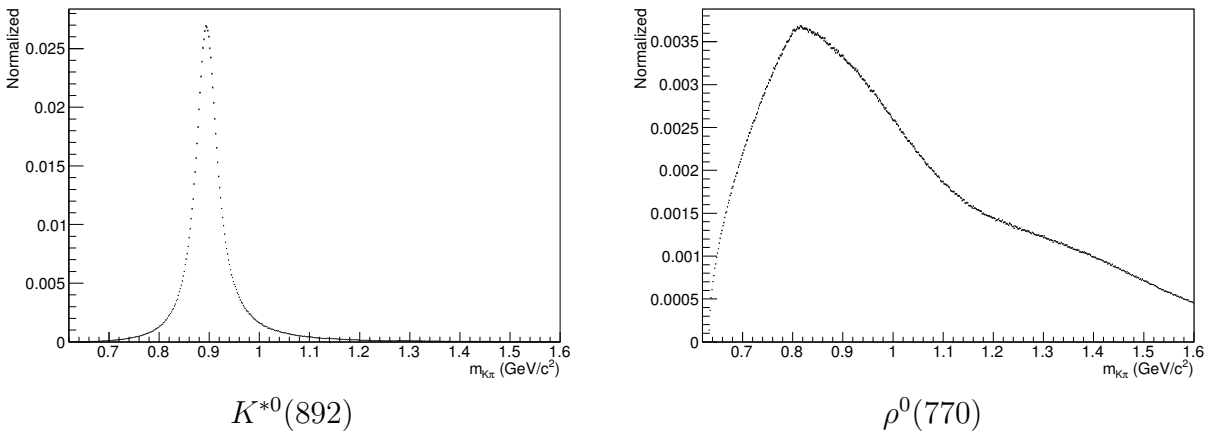
Figure 6.42: Two-dimensional histogram projections used to describe the K^{*0}(892) and the \rho^0(770) resonance modules in the m_{K\pi} fit model. The histograms were generated using EvtGen [?] at the generator level.
