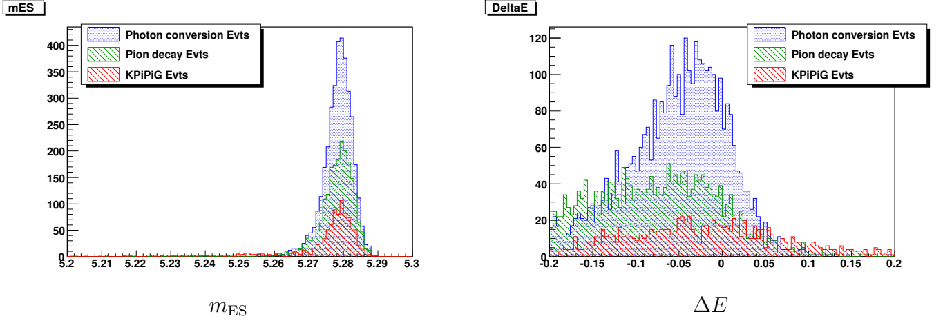
Figure 6.9: Distributions of TM events, wrongly assigned to the SCF category, in the two kinematical variables entering the final fit ( m_{ES} and \Delta E ). Photon conversions are presented in blue, the pion decays in green, and the kaon/pion swap in red.
