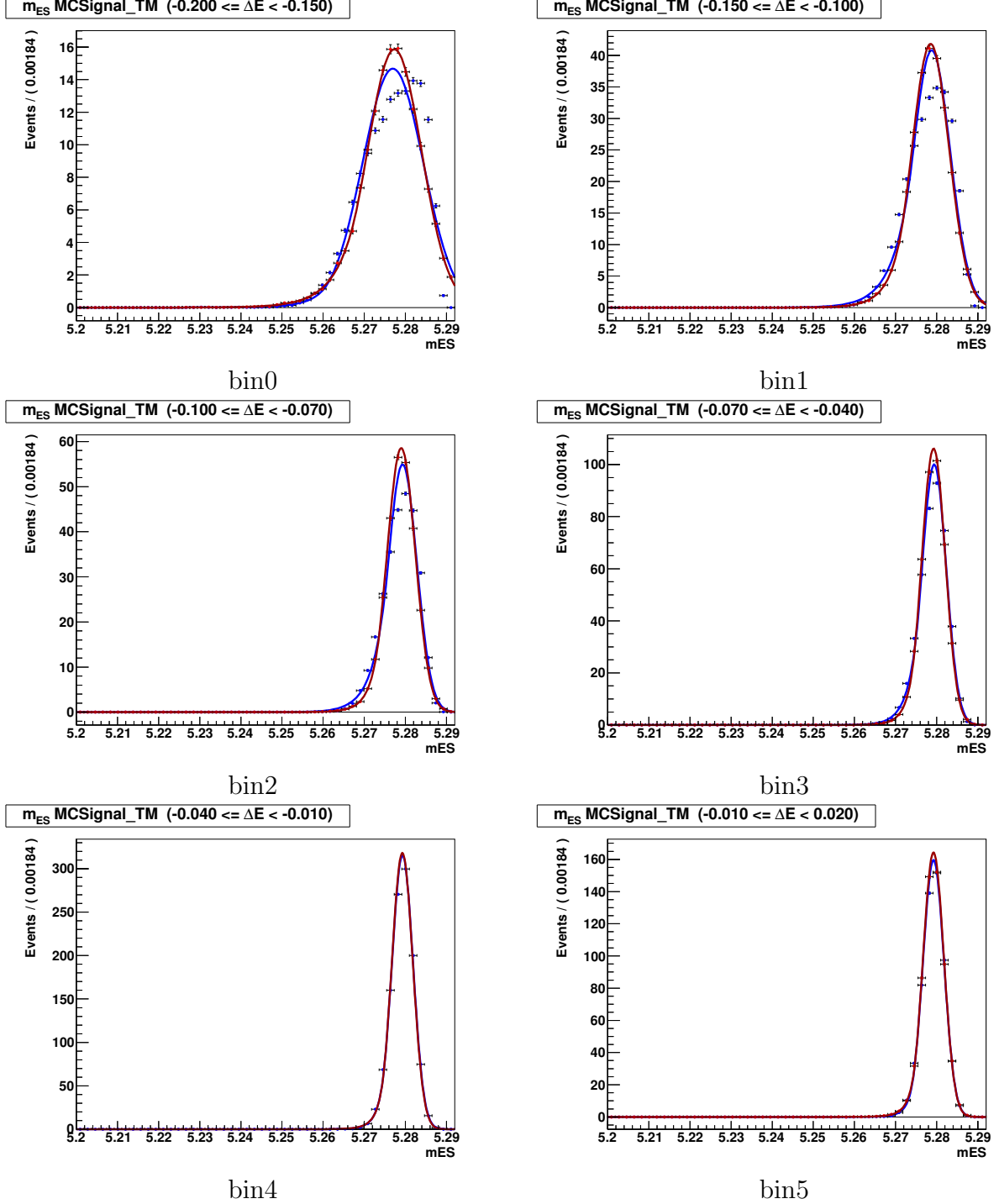
Figure D.6: m_{\text{ES}} Crystal Ball fit projection in \Delta E bins 0 to 5. Blue curve correspond to MC sample, red curve correspond to generated sample using our two-dimensional conditional PDF.
