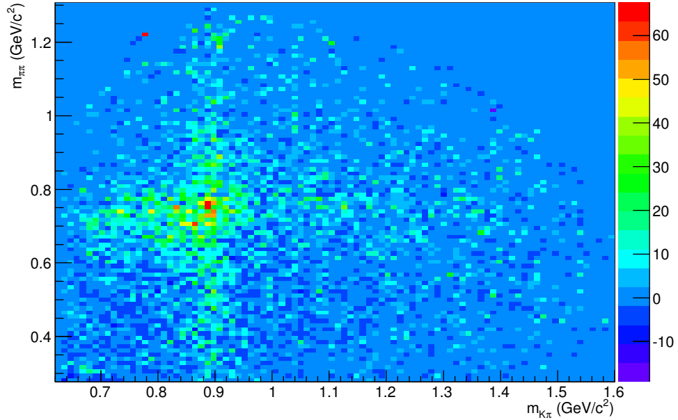
Figure 6.40: Signal-TM two-dimensional (m_{K\pi}, m_{\pi\pi}) sPlot distribution, before application of the efficiency correction.
