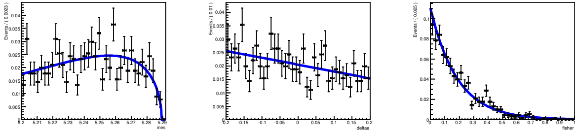
Figure 7.15: PDFs of B^0 \rightarrow K^{*0}(\rightarrow K^\pm \pi^\mp) \gamma + B^0 \rightarrow X_{sd}(\rightarrow K^\pm \pi^\mp) \gamma background category. Conventions are similar to those of Fig. 7.8. Here the m_{\text{ES}} PDF is described by an Argus, the \Delta E PDF is described by a first order Chebychev polynomial function and the Fisher discriminant PDF is described by an exponential.
