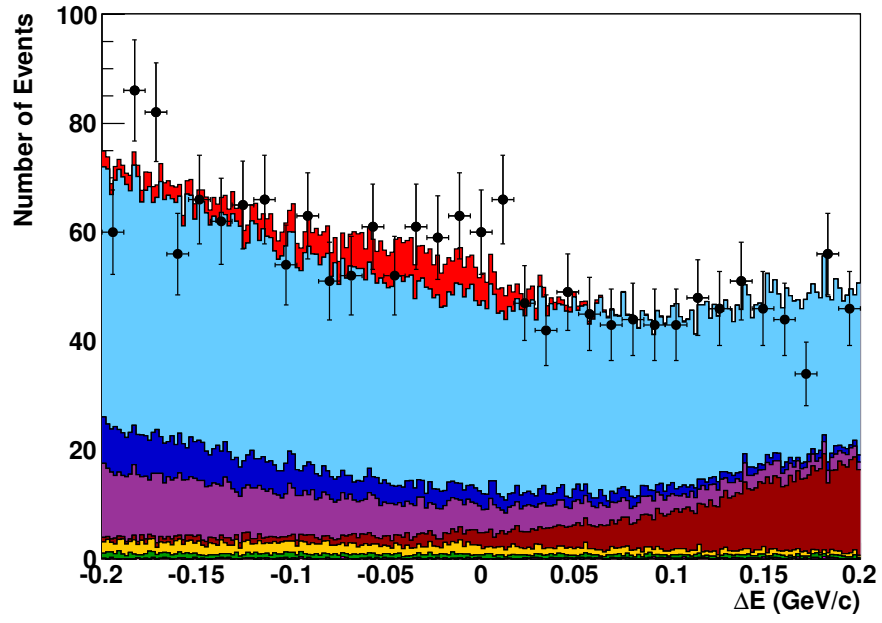
Figure F.15: \Delta E fit projection in m_{\text{ES}} bin 9.
