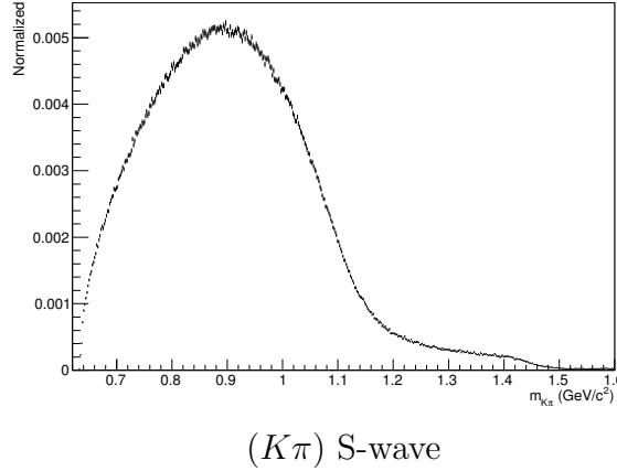
Figure 6.43: Two-dimensional histogram projection used to describe the 0^+ ( K\pi ) S-wave component in the m_{K\pi} fit model. The histogram was generated using an accept-reject method base on the LASS parametrization applied to a phase-space distribution generated using EvtGen [?] at the generator level.
