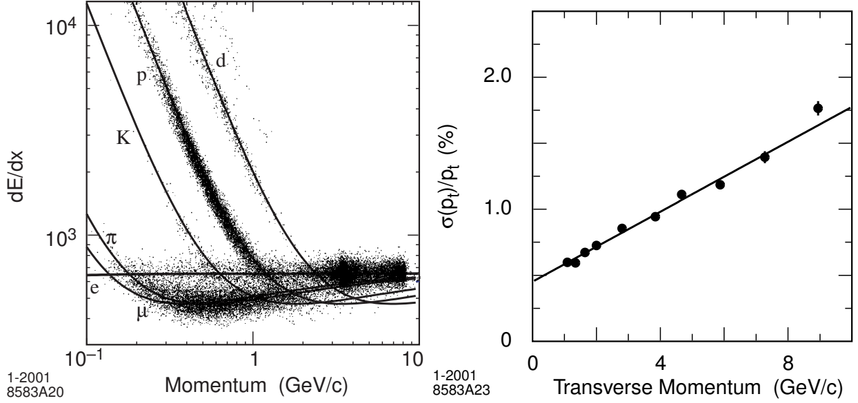
Figure 4.4: On the left, DCH dE/dx measurements and the Bethe-Bloch predictions [? ]. On the right, the resolution on p_t as calculated from cosmic ray events that fall within the acceptance of the SVT and the DCH [? ].
