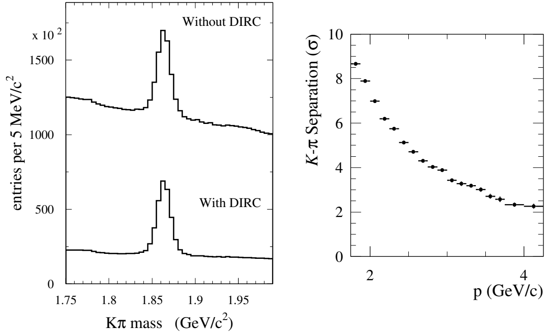
Figure 4.6: Plots illustrating the DIRC capabilities for kaon-pion separation [? ]. On the left, the reconstructed \bar{D}^0 mass with and without the PID information provided by the DIRC. On the right, the separation of kaons and pions achieved by the DIRC in standard deviations.
