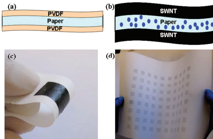
Figure I. 7 (a) Scheme of paper treatment with PVdF, used to block the micro-sized pores and avoid short circuiting because of SWCNT penetration, (b) paper supercapacitor structure with SWCNT film printed on both sides of the treated paper, by means of rod-coating or ink-jet printing, (c) photo of a rod-coated supercapacitor on paper, (d) photo of an ink-jet printed supercapacitor on paper. Reprinted with permission from “Printed energy storage devices by integration of electrodes and separators into single sheets of paper” by L. Hu, H. Wu, Y. Cui, 2010. Applied Physics Letters , 96, 183502-183502-3. Copyright 2012 by American Institute of Physics.
