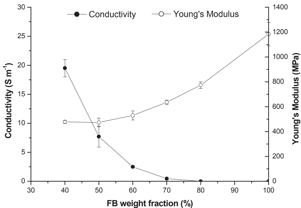
Figure III. 16 CB/FB composite paper conductivity and Young's Modulus values as a function of the FB content.
