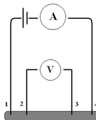
Figure II. 4 Four-probe configuration.
