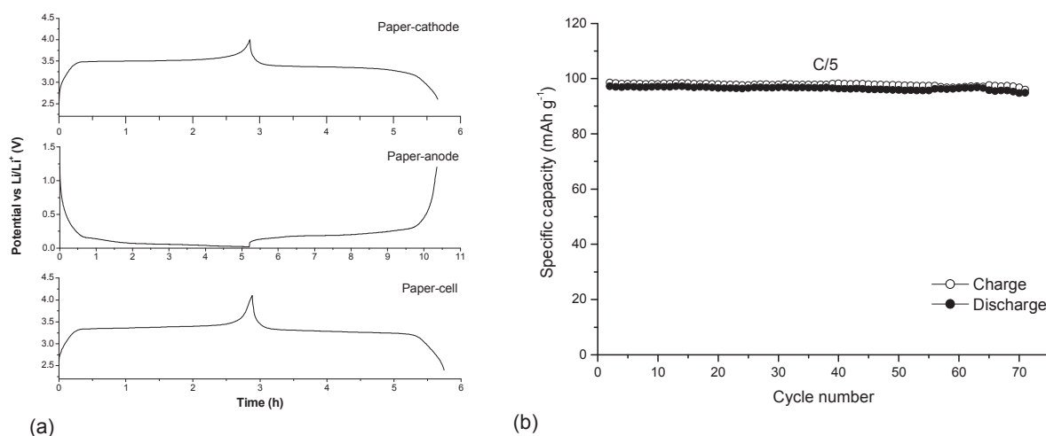
Figure III. 22 Electrochemical performances of the paper-electrodes and the paper-cell at ambient temperature. (a) Charge/discharge potential profiles of the paper-electrodes (LiFePO 4 /CB/FB cathode, 100 th cycle, and GP/FB anode, 50 th cycle) half cells and the paper-cell (2 nd cycle), obtained by sandwiching three layers of paper separator between the two electrodes. The applied current for both the cathode and the cell was 0.1 mA and for the anode was 0.2 mA. (b) Paper-cell specific charge/discharge capacity at C/5 current rate.
