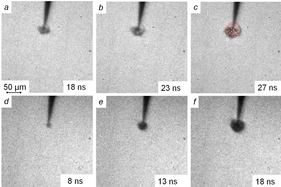
Figure 4.3 Initiation and development of slow ‘bush-like’ mode at a) – c) 4 kV, d) – f) 9 kV on the \text{\O}2\ \mu\text{m} pin electrode. Deionized water. Camera gate is 2 ns
