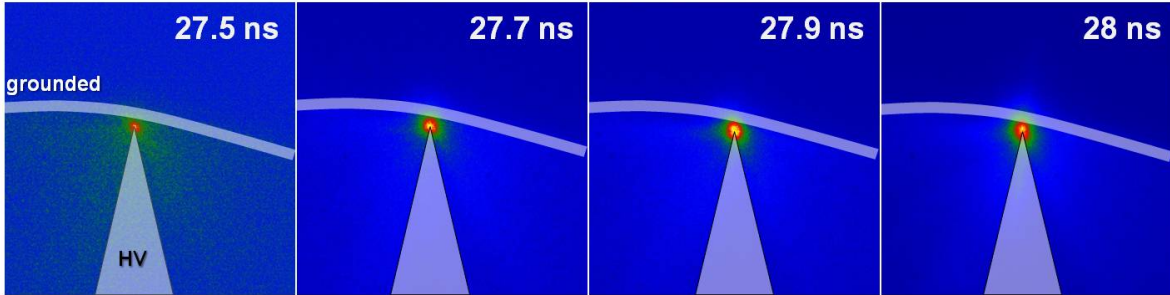
Figure 3.9 Formation of spark discharge in air. Discharge gap was about 100 \mu\text{m} and voltage amplitude on the tip was 13 \text{ kV} . Time on emission images corresponds to specified delay of iCCD camera exposure gate ( \tau_g ) in respect to triggering signal.
