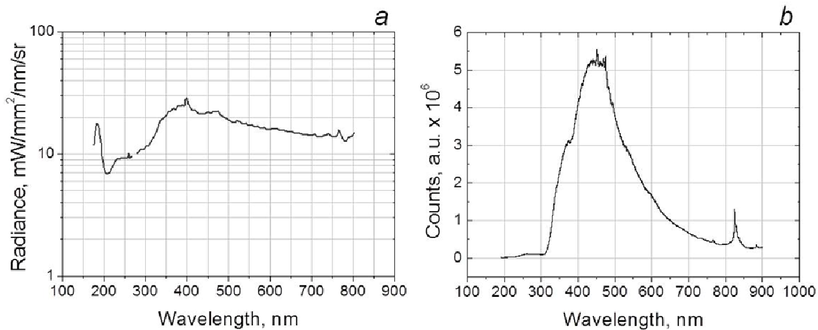
Figure 3.11 a) Radiance of EQ-99 calibration lamp, b) Calibration spectrum of Andor Shamrock R-303i spectrometer equipped with 600 \text{mm}^{-1} grating.
