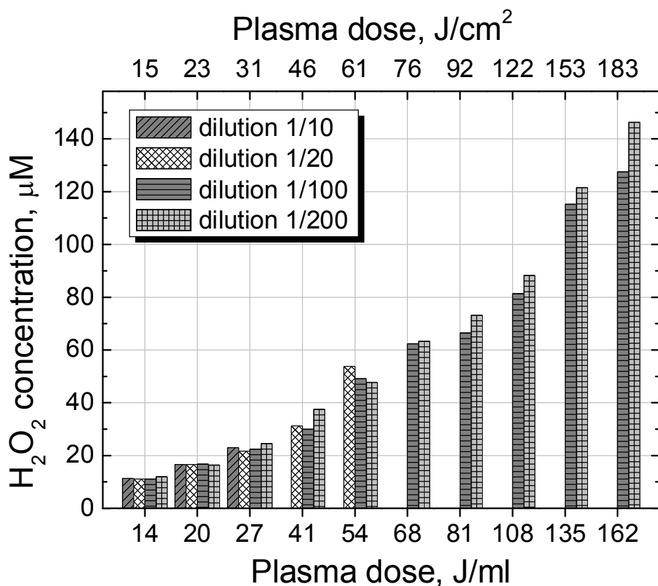
Figure 3 Production of H_2O_2 in 2 ml of PBS Mg^{2+}Ca^{2+} treated by DBD plasma at 150 Hz. Plasma doses in Joule per milliliter and square centimeter are given. Several dilutions were used in order to avoid saturation of the fluorescent signal.
