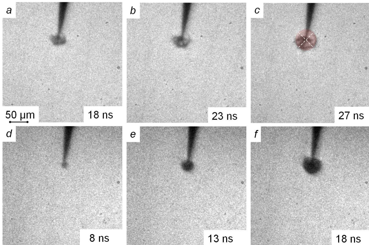
Figure 4.3 Initiation and development of slow ‘bush-like’ mode at a) – c) 4 kV, d) – f) 9 kV on the \text{Ø}2 \mu\text{m} pin electrode. Deionized water. Camera gate is 2 ns
