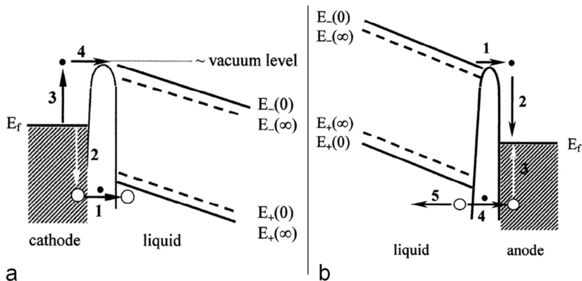
Figure 2.6 a) Generation of Auger electron from the cathode by neutralization of positive ion b) Generation of positive hole in Auger process of neutralization of negative ion or electron. Taken from (Lewis 2003)
