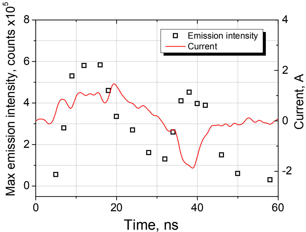
Figure 4.27 Evolution of plasma emission intensity and transient current of tree-like discharge in deionized water at 15 kV.
