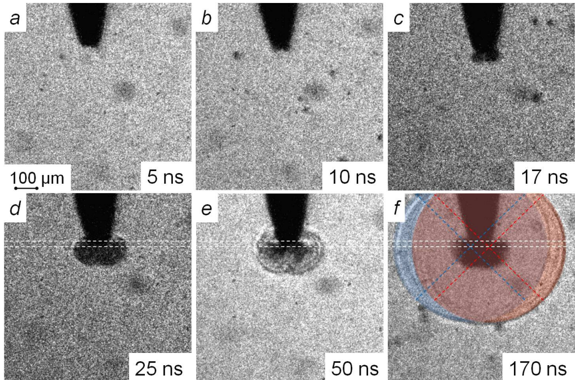
Figure 4.4 Initiation and development of slow ‘bush-like’ mode at 19 kV on \text{\O}60 \mu\text{m} tip. Deionized water. Camera gate is 2 ns.
