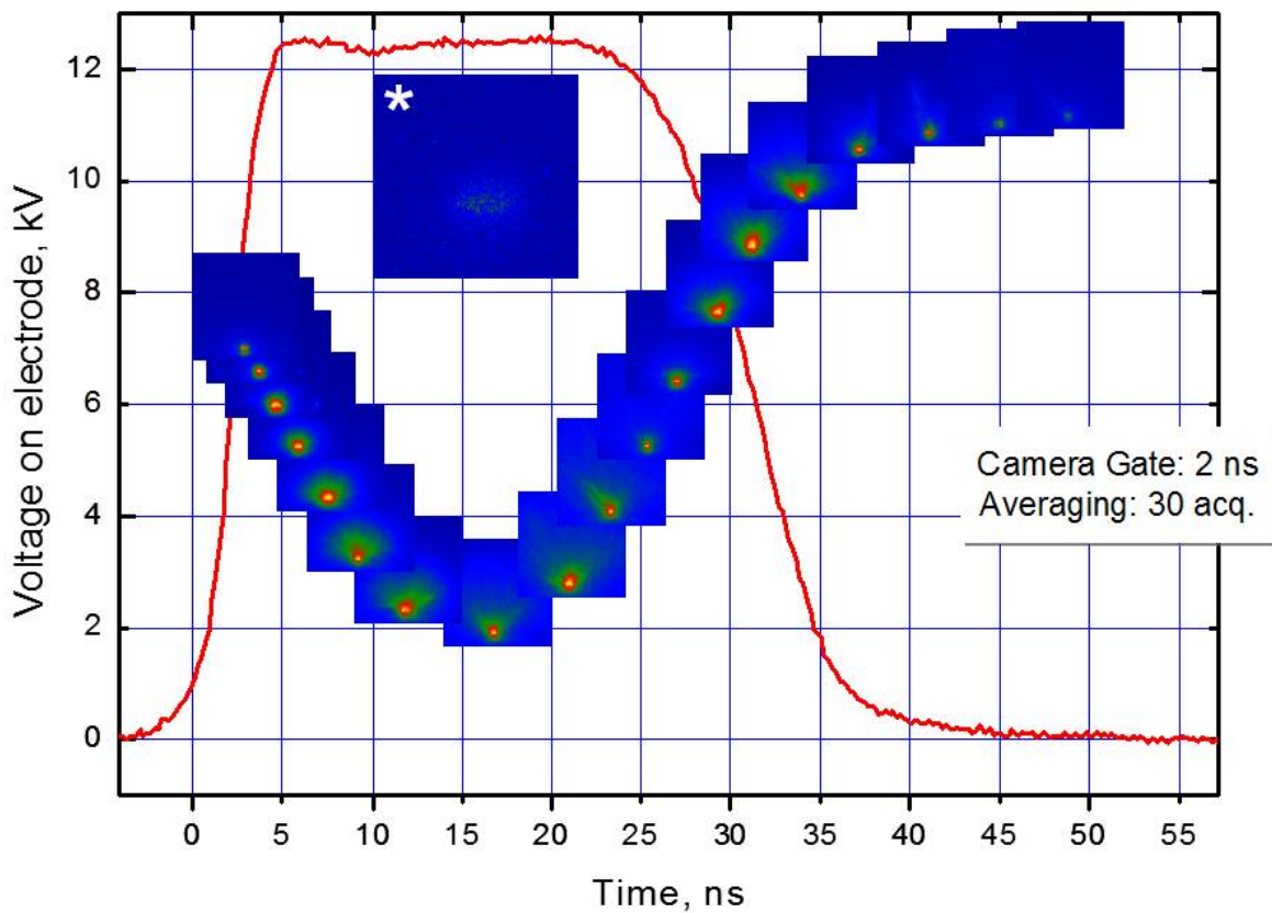
Figure 4.25 Time-resolved evolution of plasma emission averaged over 30 shots. iCCD camera gate is 2 ns. (*) Averaged optical emission from bush-like discharge in single shot. iCCD camera gate is 40 ns..
