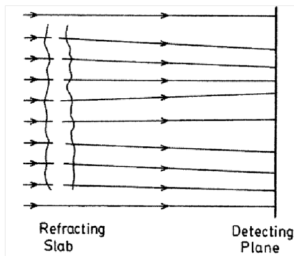
Figure 3.5 Principle of shadowgraph imaging (taken from (Hutchinson 2002)).
