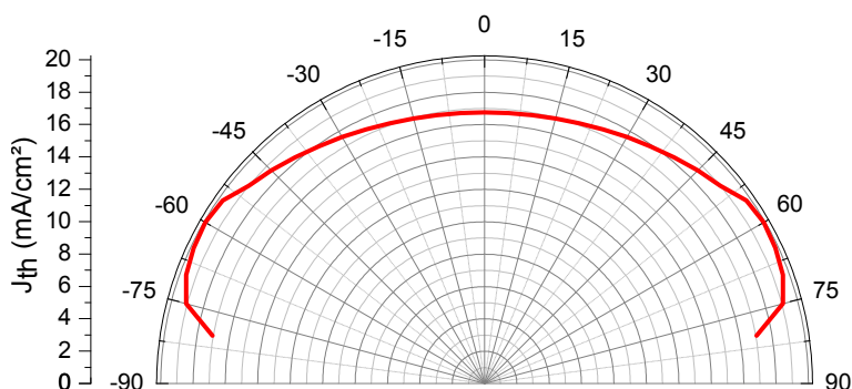
Figure 4.6.8: Angular diagram of the theoretical short circuit current (in mA/cm 2 ) for the 1D 25 nm-thick GaAs structure in function of the incident light angle (in degree).
