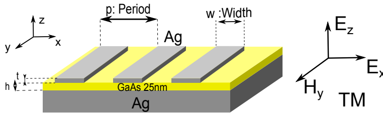
Figure B.1.1: 1D MSM nano-cavity array structure of Chapter 4. It is composed of a 25 nm-thick GaAs layer, a silver mirror and a metallic array of one dimensional (i.e. infinite along their length and the y axis) silver wires array. The definition of transverse magnetic (TM) mode is displayed.
