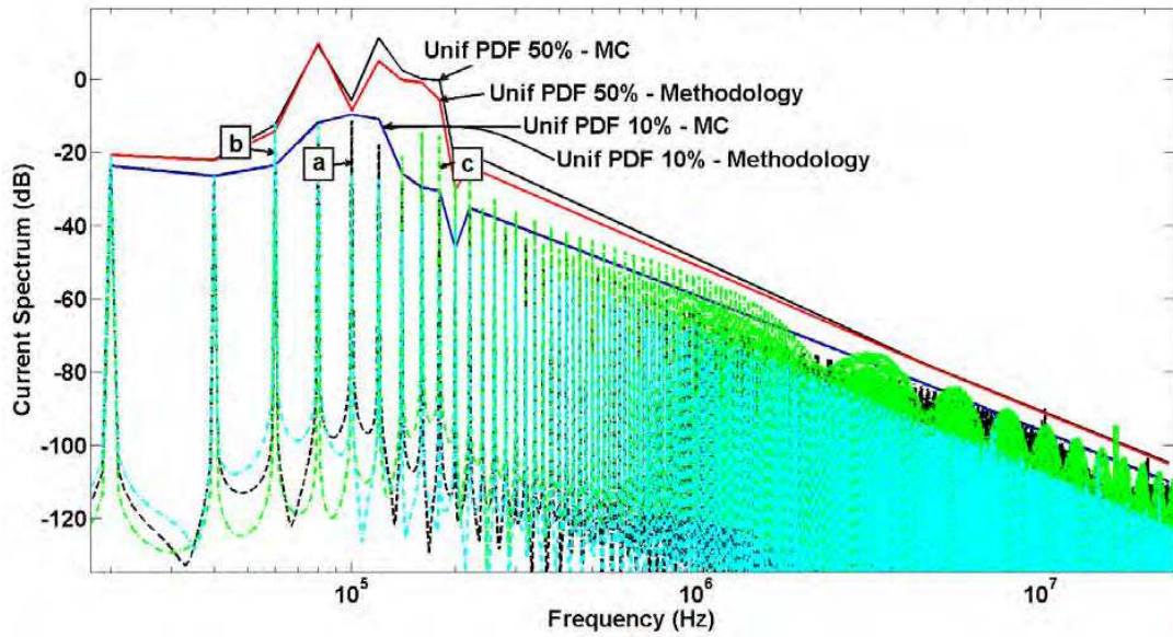
Figure 5 - 10 - Confidence Intervals of the Output Current in dB C and L following: A Uniform PDF, 10% and 50% around average Confidence level of 0.01%; Deterministic plots: \mathbf{a} - C_o and L_o ; \mathbf{b} - 1.4C_o and 1.4L_o ; \mathbf{c} - 0.6C_o and 0.6L_o ; C_o = 25.33 \text{ nF} and L_o = 100 \text{ nH}
