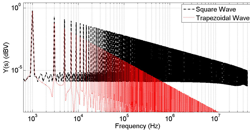
Figure 1 - 17 - Comparison of Square and Trapezoidal Wave Spectra
