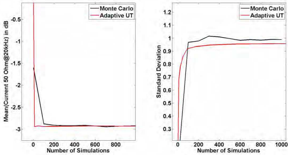
Figure 5 - 35 - Results for Model 3, DC-DC Converter, 10% interval
