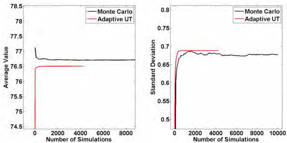
Figure 5 - 32 -- Results for Model 2, 20% interval
