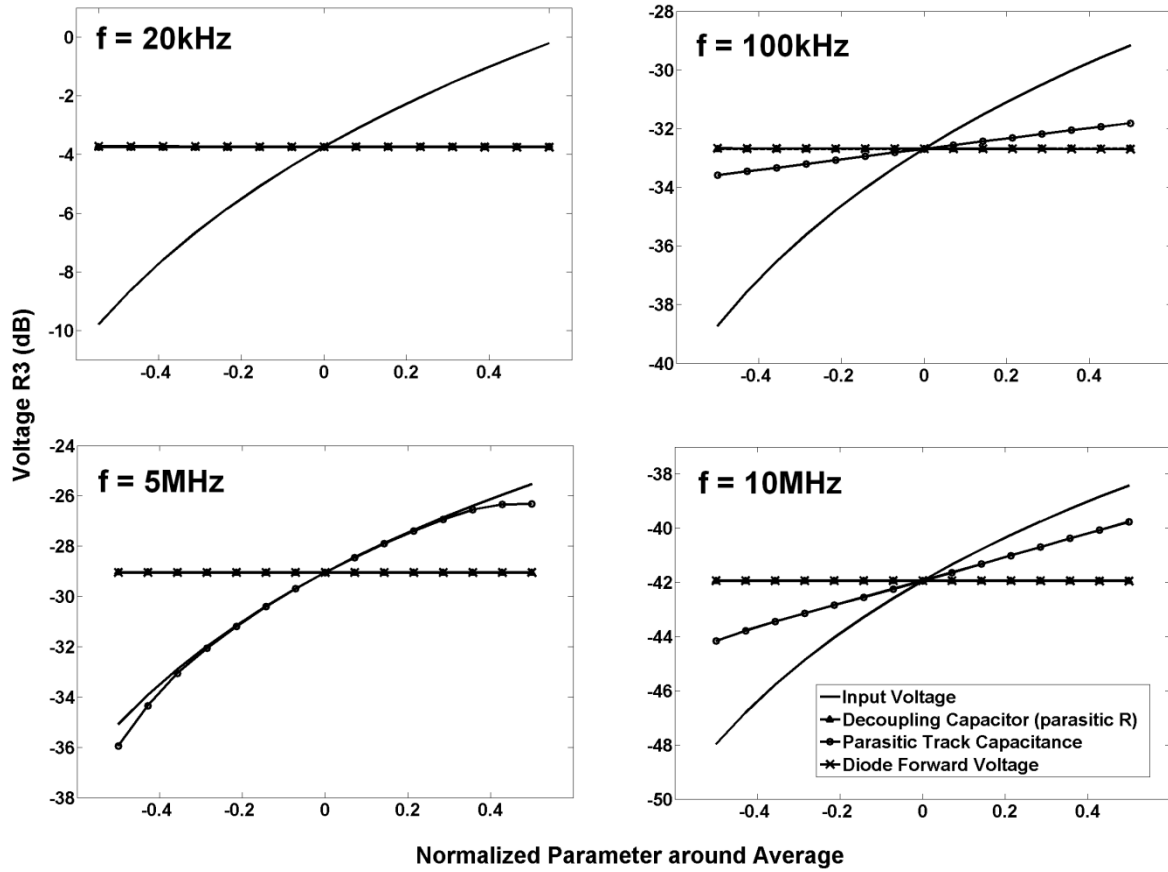
Figure 5 - 13 - Sensitivity Analysis of 4 parameters
