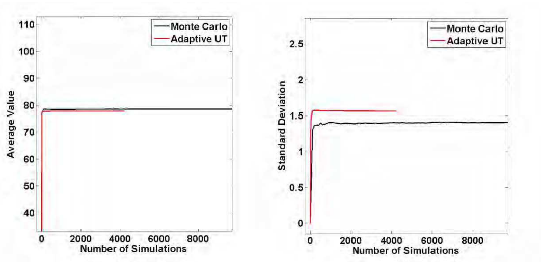
Figure 5 - 33 - Results for Model 2, 40% interval
