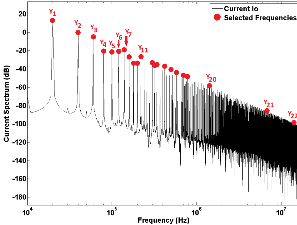
Figure 5 - 3 - Output Current I_o vs. Frequency Selected frequencies highlighted in red (Output reduction)
