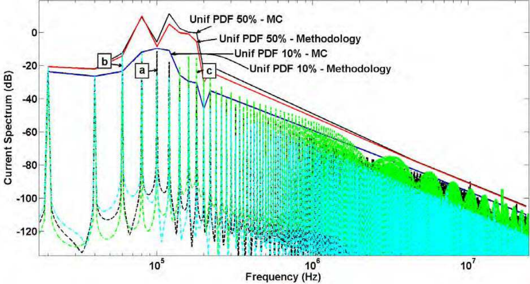
Figure 5 - 10 - Confidence Intervals of the Output Current in dB C and L following: A Uniform PDF, 10% and 50% around average Confidence level of 0.01%; Deterministic plots: a - C_o and L_o ; b - 1.4C_o and 1.4L_o ; c - 0.6C_o and 0.6L_o ; C_o = 25.33 \text{ nF} and L_o = 100 \text{ nH}
