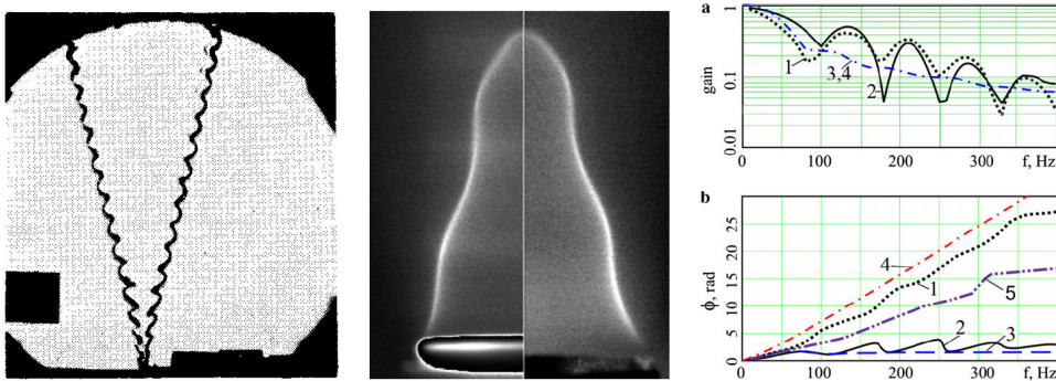
Figure 1.7: (left) Image of a V-flame which rim is undergoing a transverse motion. Reproduced from Petersen and Emmons (1961) . (center) Comparison between shapes taken by conical flames with a longitudinal rim perturbation and an acoustic flow modulation. Reproduced from Kornilov et al. (2007) . (right) Comparison of different FTFs: 1-Experimental FTF of an acoustically perturbed flame. 2-Experimental FTF of a flame with a longitudinal rim excitation. 3-Theoretical FTF from Ducruix et al. (2000) . 4-Theoretical FTF from Schuller et al. (2003a) . 5-Experimental FTF of a flame with a transverse rim excitation. Reproduced from Kornilov et al. (2007) .
