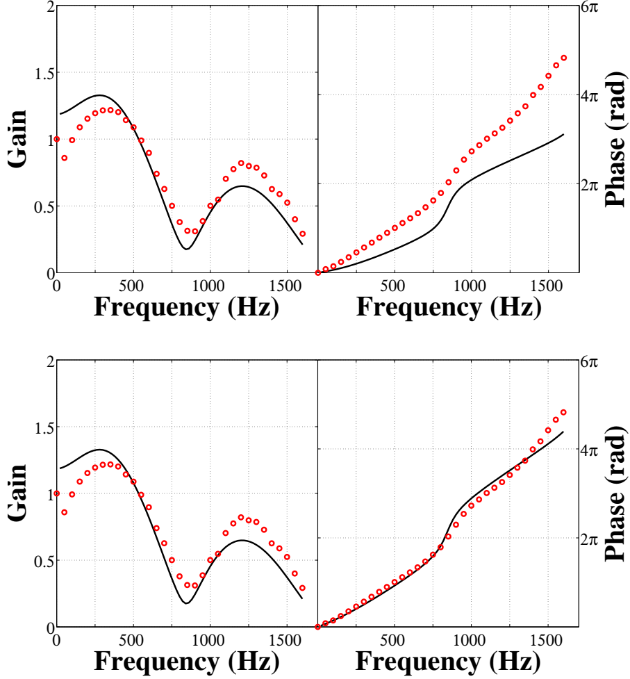
Figure 6.19: Comparisons between FTF measurements (red circles) and different FTF models (black lines). (top) F_A(\omega_*^c, \alpha) + F_B(\omega_*^c, \alpha, \Psi_f, \delta_*, Ze) . (bottom) [F_A(\omega_*^c, \alpha) + F_B(\omega_*^c, \alpha, \Psi_f, \delta_*, Ze)] \exp(i\omega\tau_s) .
