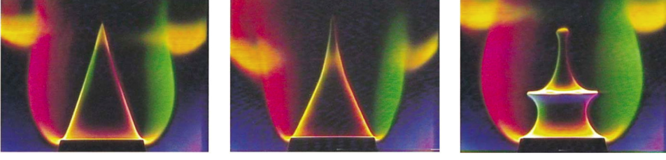
Figure 1.1: Three color Schlieren images of \text{CH}_4/\text{air} conical flames. (left) Steady flame for v_0 = 0.96 \text{ m.s}^{-1} and \phi = 0.95 . (center) Perturbed flame at f = 25 \text{ Hz} . (right) Perturbed flame at f = 75 \text{ Hz} . Reproduced from Ducruix et al. (2000) .
