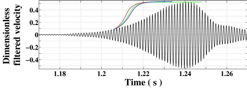
Figure B.10: Filtered dimensionless velocity measurements as a function of time. Colored lines represents the instability amplitude time evolution determined from the results of the nonlinear stability analysis: (red line) The flame frequency response and the inlet and outlet reflection coefficients are taken as F(\omega_r) and R(\omega_r) . (green line) F(\omega) and R(\omega_r) . (blue line) F(\omega) and R(\omega) .
