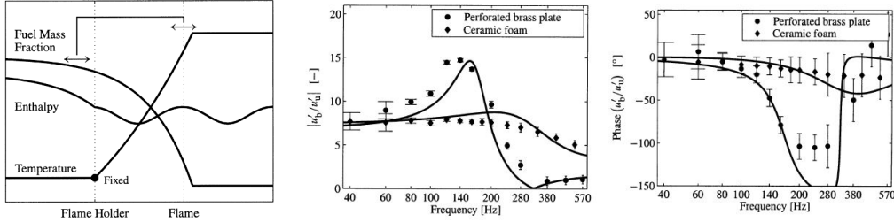
Figure 1.8: (left) Scheme of the resonant coupling that can occur between the flame holder and the flame front involving enthalpy fluctuation and flame front motion. (center and right) Velocity Transfer Function gain and phase for two different burner materials. Experimental data are plotted with circles while the theoretical model is plotted with lines. All the figures are reproduced from [Schreel et al. (2002)]. A \exp(i\omega t) -convention was adopted in this article.
