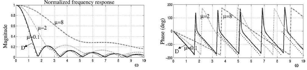
Figure 1.6: Exothermicity effects on the FTF gain (left) and phase lag (right) of a ducted V-flame. The different curves are a function of the parameter \mu = \rho_u/\rho_b - 1 . Reproduced from Mehta et al. (2005) . The FTF phase decreases at low frequencies because the “ \exp(i\omega t) ” convention was adopted in this article.
