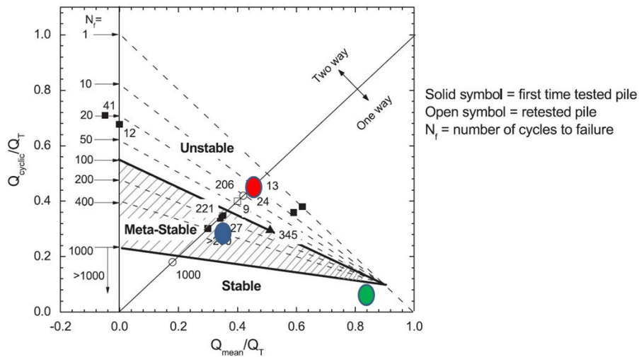
Figure 54: Loading cycles [110] [62]
