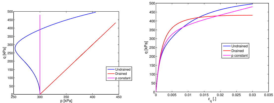
Figure 8: p' - q and \epsilon_q - q
