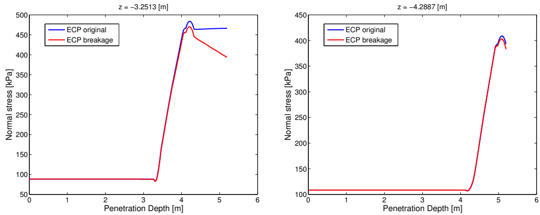
Figure 38: Interface normal stress evolution during installation considering or not the breakage mechanism
