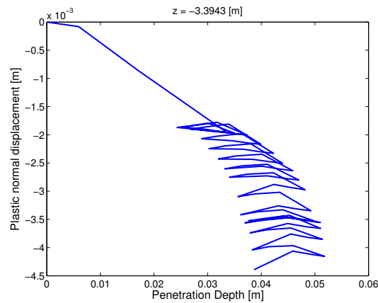
Figure 70: u_n^p - Plastic normal displacement
