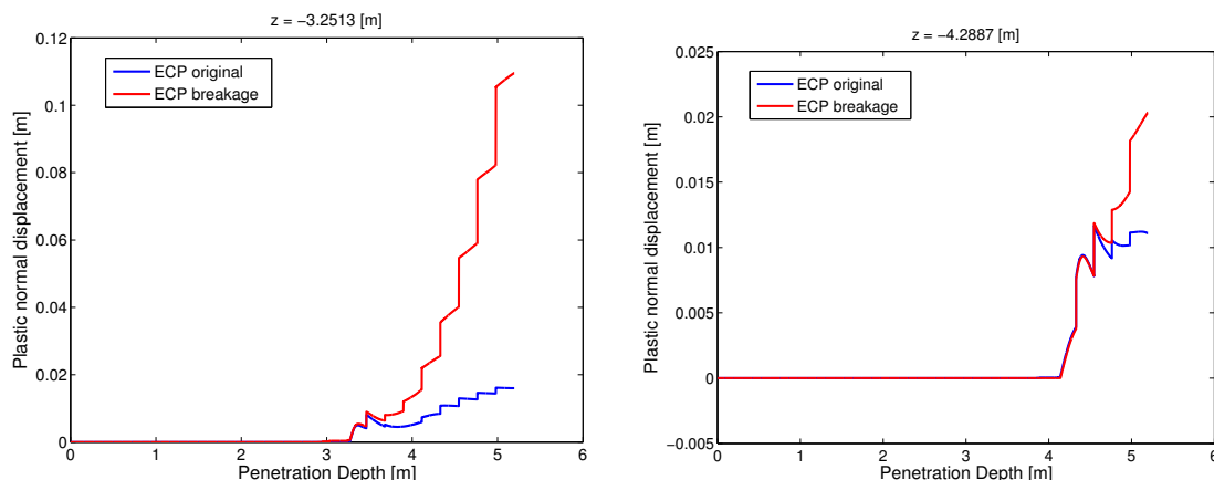
Figure 40: u_n^p evolution during installation considering or not the breakage mechanism
