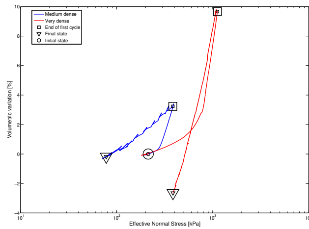
Figure 31: \sigma'_n - \dot{J}
