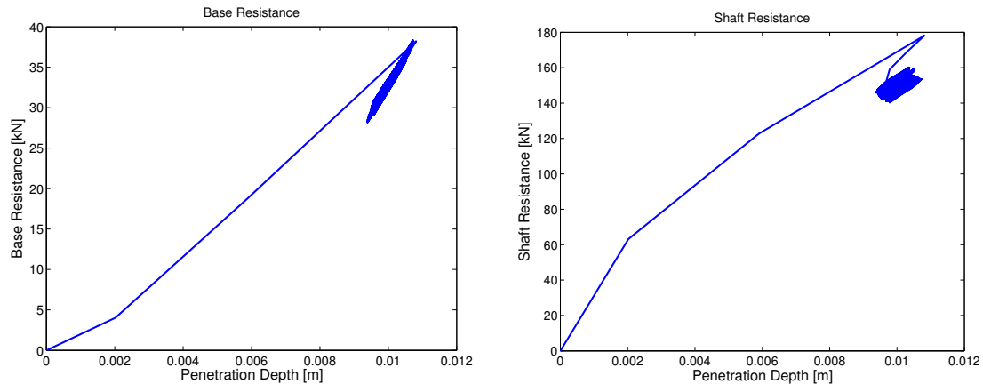
Figure 55: Base and Shaft resistances - Medium initial loading
