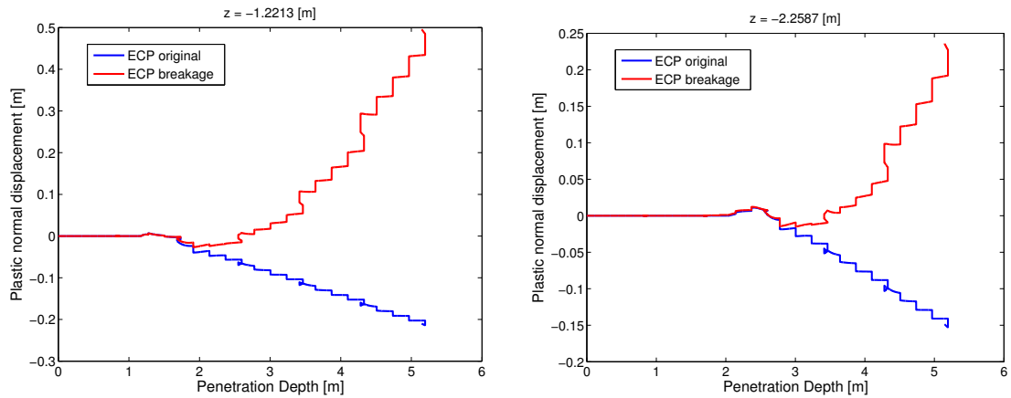
Figure 43: u_n^p evolution during installation considering or not the breakage mechanism
