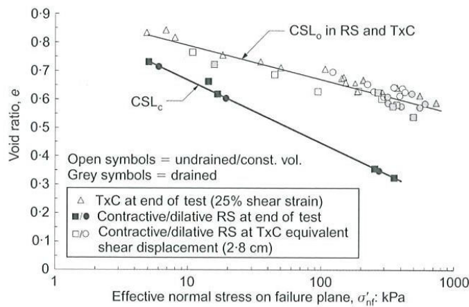
Critical state lines of original ( CSL_0 ) and crushed ( CSL_c ) IR sand from TxC and RS tests
