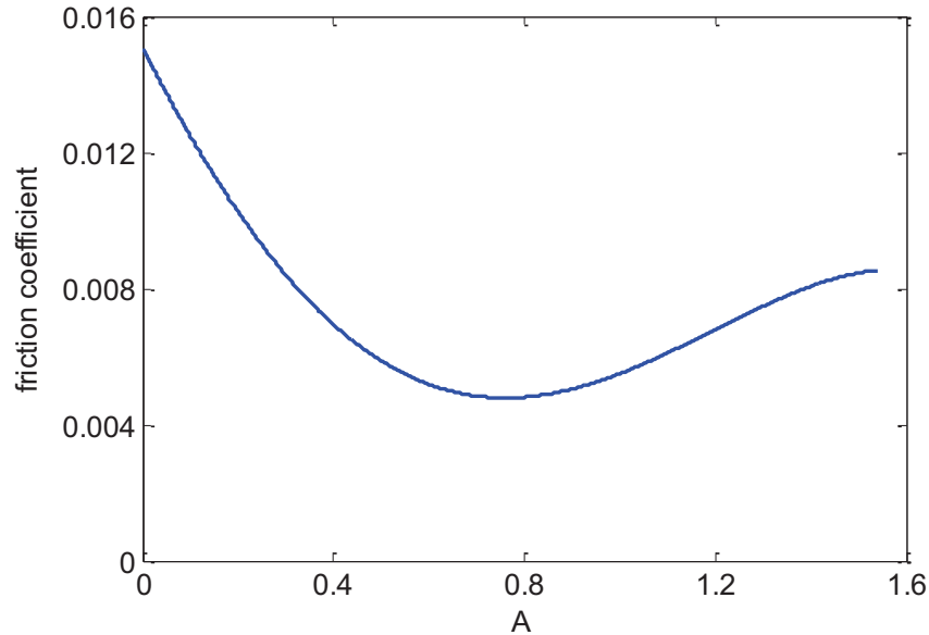
Figure 43. Friction coefficient as a function of A .
