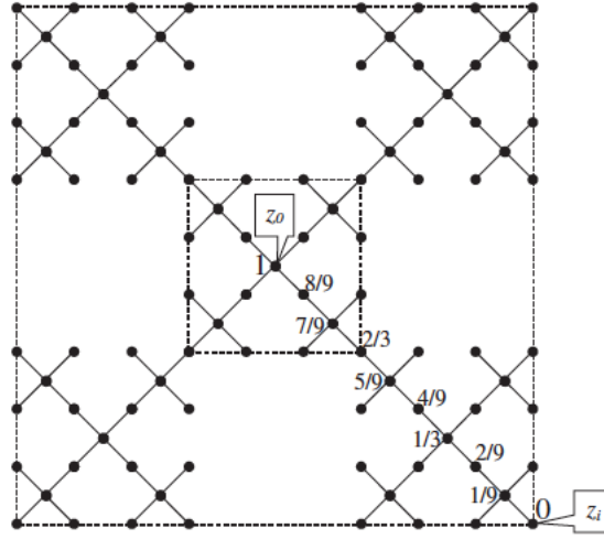
Figure 5.2: the function f on the diagonal z_0 z_i
