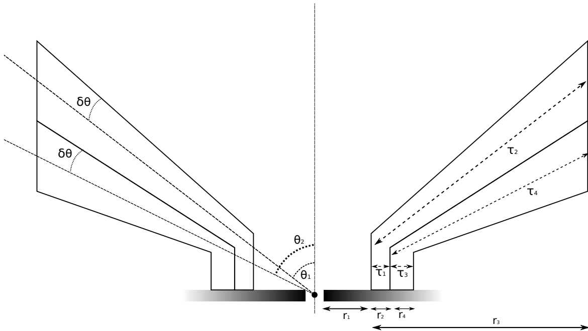
Figure 8.9: A two-phased medium where the cool WHIM outflow is composed of dust.
