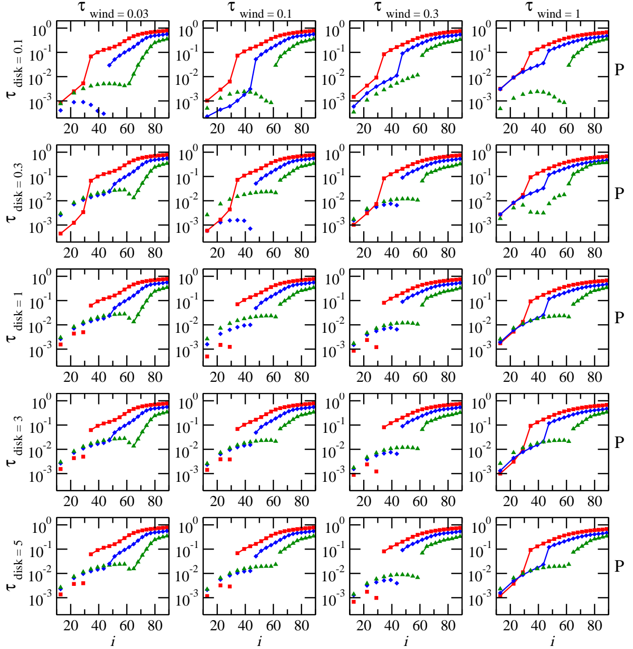
Figure 4.24: Resulting percentage of polarization, P , as a function of viewing angle, i , for a complex AGN model (see text). The half-opening angle of the equatorial scattering disk is set to 10^\circ . Legend: The different curves denote common half-opening angles of the torus and the polar winds of 30^\circ (red squares), 45^\circ (blue diamonds), and 60^\circ (green triangles with points to the top), see Fig. 4.23. The isolated symbols indicate a polarization position angle \psi = 90^\circ (parallel), connected symbols stand for \psi = 0^\circ (perpendicular). From left to right: increasing the polar outflow optical depth from 0.03 to 1; From top to bottom: increasing the optical depth of the equatorial disk from 0.1 to 5.
