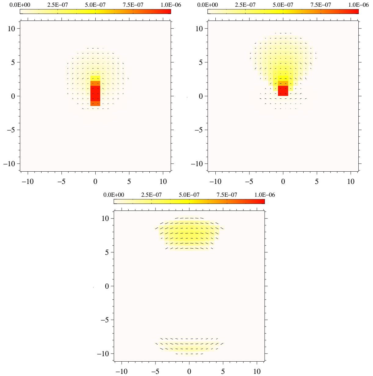
Figure 4.18: Modeling the polarized flux, PF/F_* , of electron-filled, polar outflow combined with an optically thick, dusty torus; PF/F_* color-coded and integrated over all wavelengths. Top-left: face-on image; top-right: image at i \sim 45^\circ ; bottom: edge-on image.
