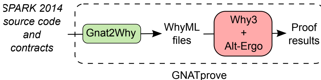
Figure 1.1: Deductive verification in SPARK 2014
