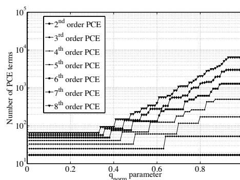
(b) 8-variate
