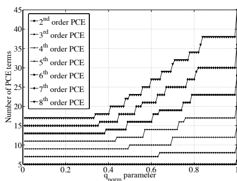
(a) 2-variate
