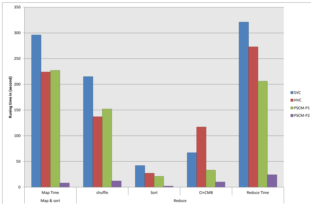
Figure 4.5: Time breakdown SCM \times 500 .
