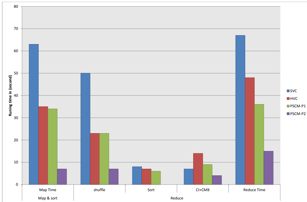
Figure 4.4: Time breakdown SCM \times 100 .
