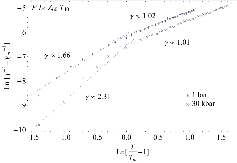
Fig. 3.43: Plots of \text{Ln}(\chi^{-1} - \chi_m^{-1}) versus \text{Ln}(T/T_m - 1) in the paraelectric regions for PL_5Z_{60}T_{40} under 1 bar and 30 kbar. Linearly fitting the data yields \gamma \simeq 1 in both cases for high enough temperatures. As the temperature is lowered slopes increase, \gamma \simeq 1.66 and \gamma \simeq 2.31 for 1 bar and 30 kbar respectively.
