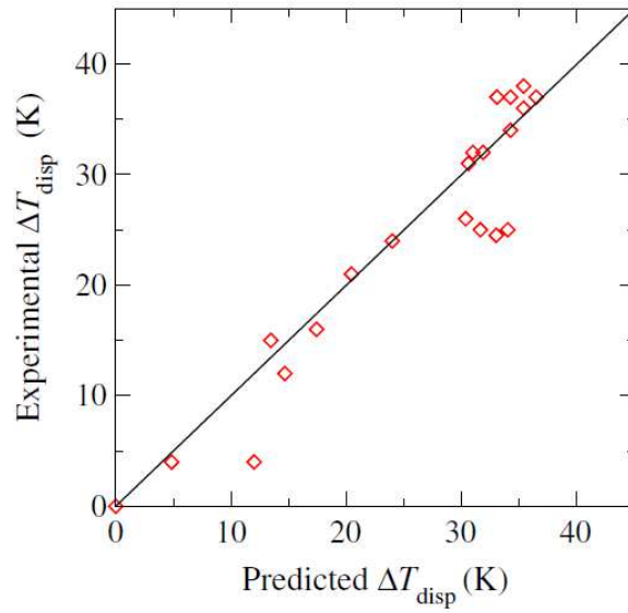
Fig. 1.17: Comparison of the \Delta T_{\text{disp}} results of the Landau theory fit with experimental \Delta T_{\text{disp}} . Data points are close to the y = x line, indicating that the Landau theory of the relaxor-to-ferroelectric transition encapsulated by Eq.1.28 and 1.29 quantitatively captures the trend of the experimental \Delta T_{\text{disp}} data, and attesting that local effects govern the magnitude of the dispersion in Pb-based relaxor ferroelectrics. (After Grinberg et al. [134])
