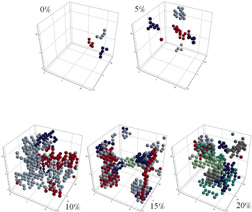
Fig. 3.38: Biggest clusters of local modes for \text{PZ}_{60}\text{T}_{40} system, just above T_C , and for \text{PL}_5\text{Z}_{60}\text{T}_{40} , \text{PL}_{10}\text{Z}_{60}\text{T}_{40} , \text{PL}_{15}\text{Z}_{60}\text{T}_{40} and \text{PL}_{20}\text{Z}_{60}\text{T}_{40} systems, for temperatures just above their T_m .
