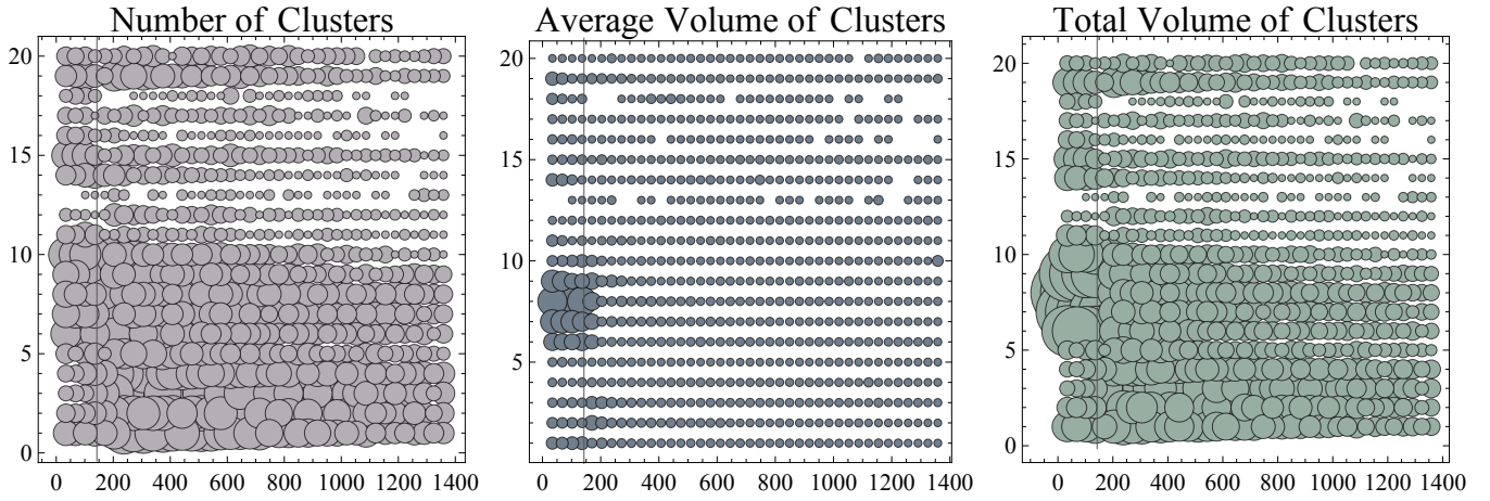
Fig. 3.37: \text{PL}_{20}\text{Z}_{60}\text{T}_{40} : Temperature evolution of the number of clusters ( N_{Cl} ), their average volume ( V_{Cl}^{av} ) and their total volume ( V_{Cl}^{tot} ) per face. The y axis refers to the face label, the x axis denotes temperature. (i) In this case, disorder extends over a wide temperature range. (ii) The ground state is strongly mixed, resulting in a triclinic average symmetry (section 3.1.5).
