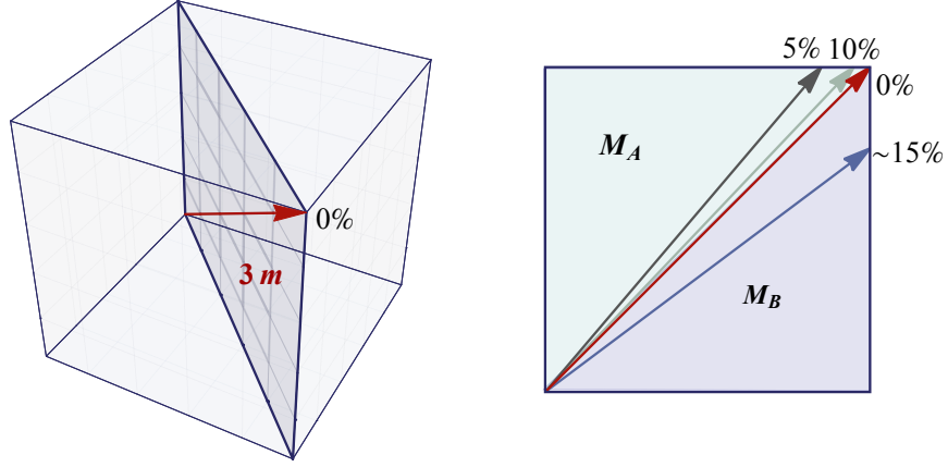
Fig. 3.25: Schematic representation of the influence of the lanthanum substitution on the low temperature structural properties of \text{PL}_x\text{Z}_{60}\text{T}_{40} for increasing lanthanum content x = 0, 5, 10, 15\% .
