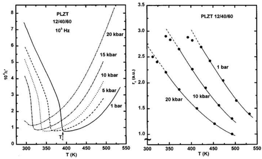
Fig. 1.43: Left panel: Temperature dependence of the reciprocal of \epsilon'(T) of PLZT 12/40/60 measured at 10^5 Hz and different pressures. The location of the structural phase transition is denoted by T_C for the 1-bar response. Right panel: Variation of the correlation radius (in arbitrary units) for polarization fluctuations with temperature for PLZT 12/40/60 (After Samara [104]).
