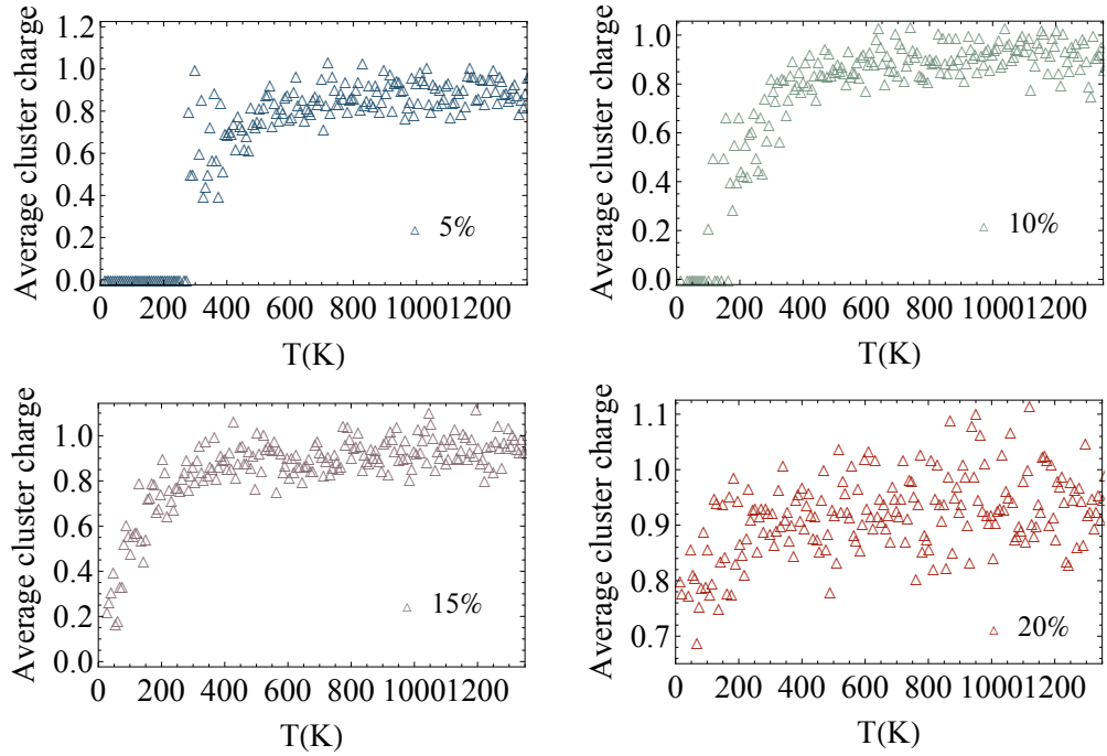
Fig. 3.59: Temperature evolution of the average charge of \{|Q| = 1\} -obtained clusters for \text{PL}_5\text{Z}_{60}\text{T}_{40} , \text{PL}_{10}\text{Z}_{60}\text{T}_{40} , \text{PL}_{15}\text{Z}_{60}\text{T}_{40} and \text{PL}_{20}\text{Z}_{60}\text{T}_{40} systems.
