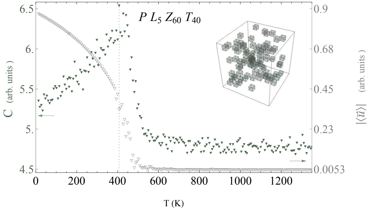
Fig. 3.2: Temperature evolutions of the specific heat (filled symbols) and the scaled polarization (open symbols) in PL_5Z_{60}T_{40} system. The inset shows the distribution of the quenched (lanthanum containing) unit cells inside the supercell. Dotted vertical line corresponds to T_C .
