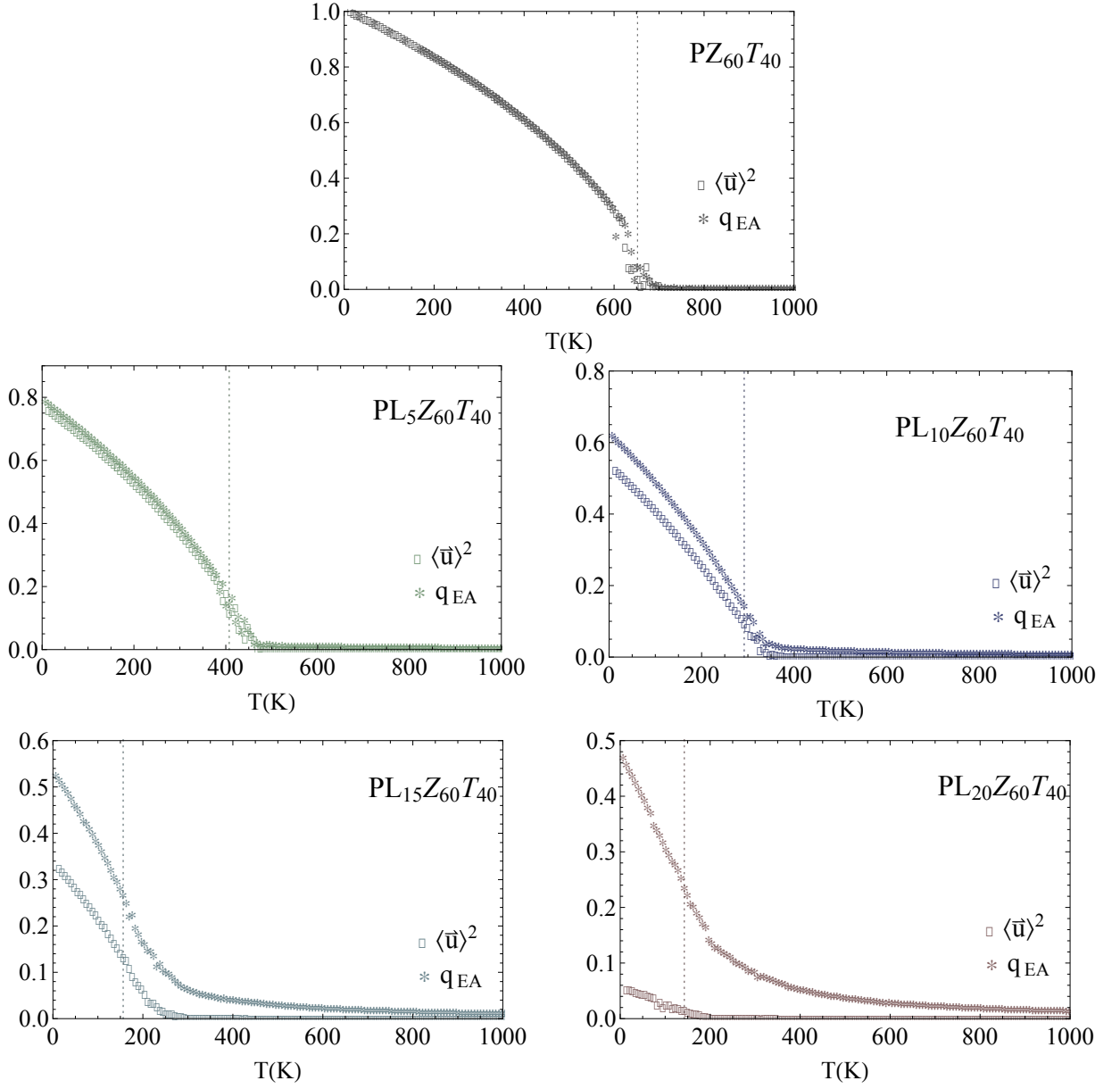
Fig. 3.26: Temperature evolutions of the Edwards-Anderson parameter q_{EA} and squared polarization \langle \vec{u} \rangle^2 , for PZT, PL 5 ZT, PL 10 ZT, PL 15 ZT and PL 20 ZT systems. Dotted vertical lines correspond to T_C ( i.e. , the temperature at which the specific heat peaks).
