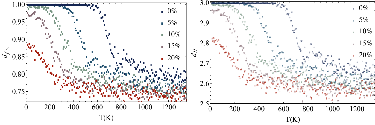
Fig. 3.54: Temperature evolution of the free volume d_{f.v} (left figure) and of its fractal dimension (right figure) for the pure system PZT and different \text{PL}_x\text{ZT} systems.
