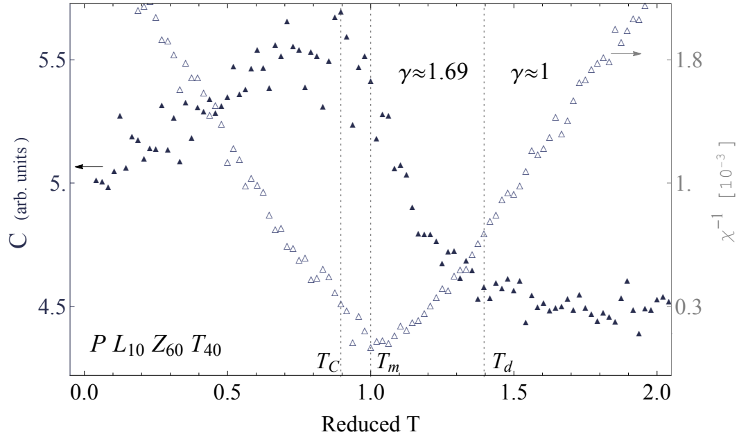
Fig. 3.14: Temperature evolution of the inverse dielectric susceptibility and the specific heat for PL_{10}Z_{60}T_{40} . T_C \simeq 292 K corresponding to the maximum of the specific heat and T_m \simeq 326 K corresponding to that of the dielectric susceptibility, are indicated by vertical dashed lines. The reduced temperature refers to T/T_m . The onset of deviation from the Curie-Weiss law at T_d \simeq 455 K is indicated by a vertical dashed line.
