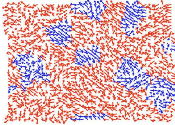
Fig. 1.21: Snapshot of local mode polarizations of PSN at T = 600 K ( \approx T_c ). Highly correlated regions are chemically ordered whereas the disordered matrix is chemically disordered. (After Burton et al. [146])
