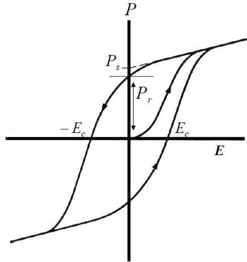
Fig. 1.2: Hysteresis dependence of the polarization of a typical ferroelectric crystal on electric field, P_S is the spontaneous polarization, P_r the remanent polarization and E_c the coercive field (figure after [37]).
