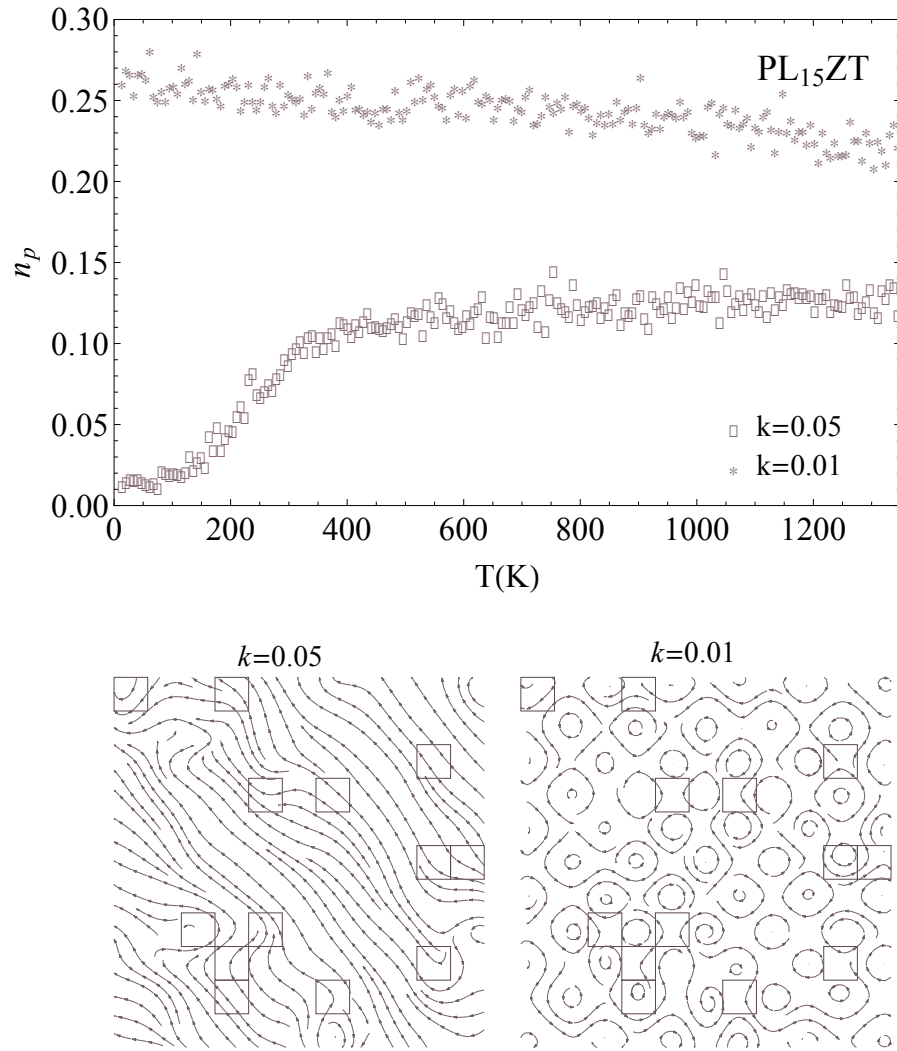
Fig. 3.61: Temperature evolution of the density of pairs of hedgehogs n_p in PL 15 ZT for k=0.01 and k=0.05 . Lower panels depict the integral curves of the order parameter field within a (x, y) plane for T=17 K. Squares indicate the spatial distribution of the quenched cells.
