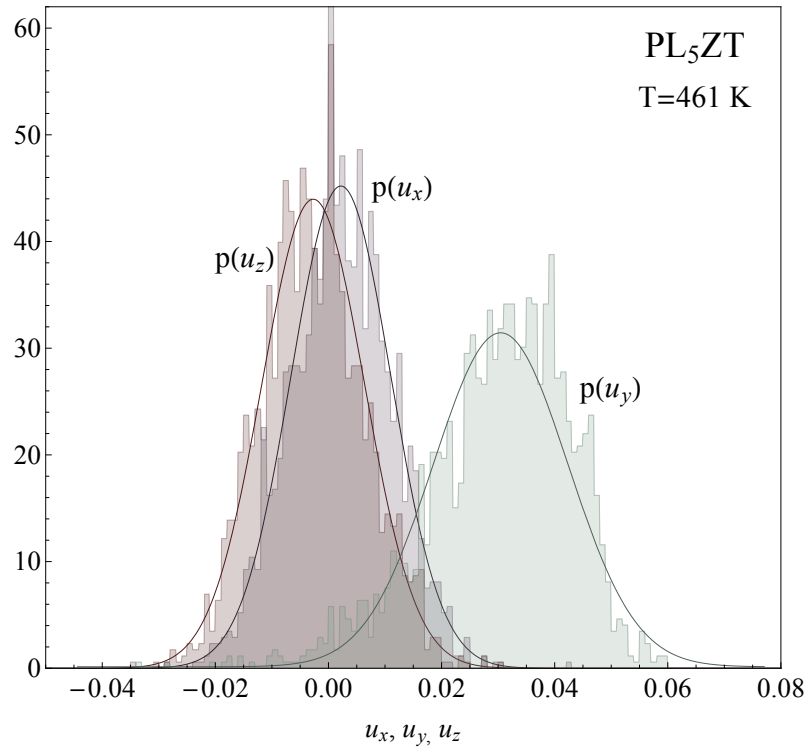
Fig. 3.24: Probability histograms for the averaged over sweeps unit cell local mode components of PL_5Z_{60}T_{40} in the tetragonal phase ( T = 461 K) in the close vicinity of the transition.
