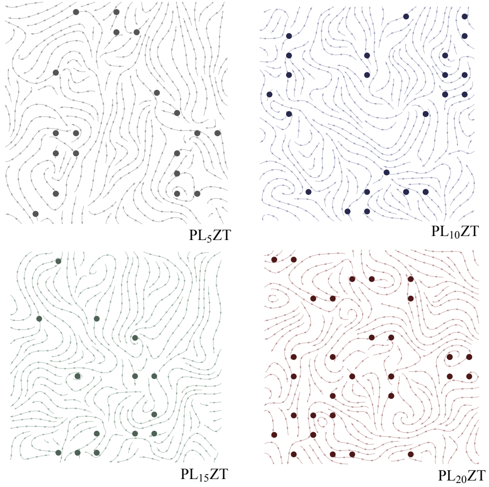
Fig. 3.48: Integral curves associated to the local modes vector fields within a (x, y) plane and projection onto the plane of topological defects (represented by points) for PL_5ZT , PL_{10}ZT , PL_{15}ZT and PL_{20}ZT . Results correspond to T \geq T_m , specifically, T = 441K , T = 340K , T = 203K and T = 170K for 5%, 10%, 15% and 20%, respectively.
