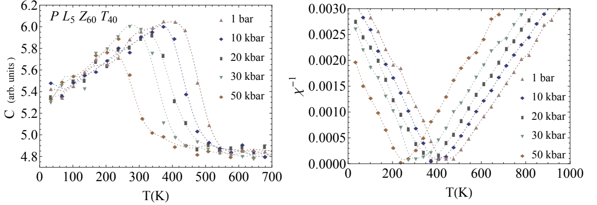
Fig. 3.41: Evolution with temperature of the specific heat (left) and the inverse dielectric response (right) for PL 5 Z 60 T 40 under 1 bar, 10 kbar, 20 kbar, 30 kbar and 50 kbar. The temperature at which the specific heat peaks is used for the determination of T_C while that at which the dielectric response peaks corresponds to T_m .
