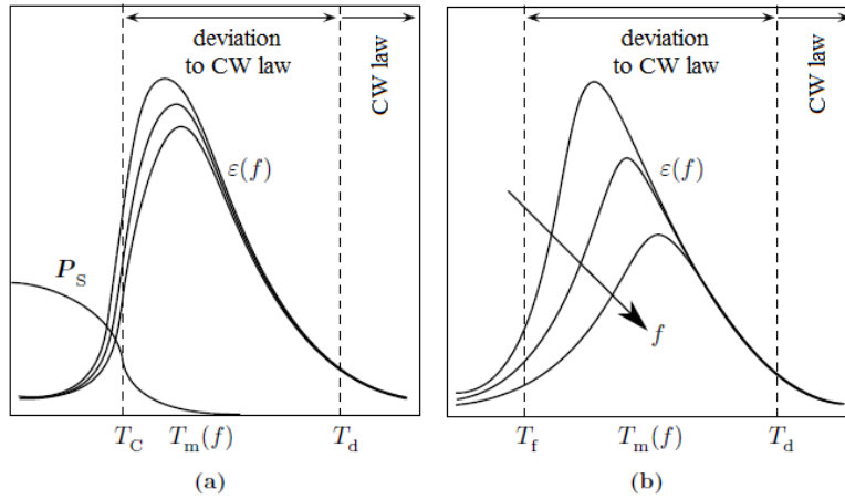
Fig. 1.32: Schematic temperature dependence of the dielectric permittivity and spontaneous polarisation, after Hirota et al. [3]: (a) relaxors with a diffuse relaxor-to-ferroelectric phase transition. T_C is below T_m(f) and spontaneous polarisation occurs already above T_C . (b) canonical relaxors. At the Burns temperature T_d , polar regions nucleate and after growing with decreasing temperature, they freeze to a non-ergodic state at T_f . Polarisation appears only under an external electric field.
