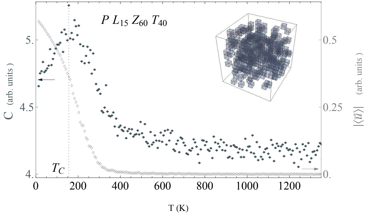
Fig. 3.4: Temperature evolutions of the specific heat (filled symbols) and the scaled polarization (open symbols) in PL_{15}Z_{60}T_{40} system. The inset shows the distribution of the quenched (lanthanum containing) unit cells inside the supercell. Dotted vertical line corresponds to T_C .
