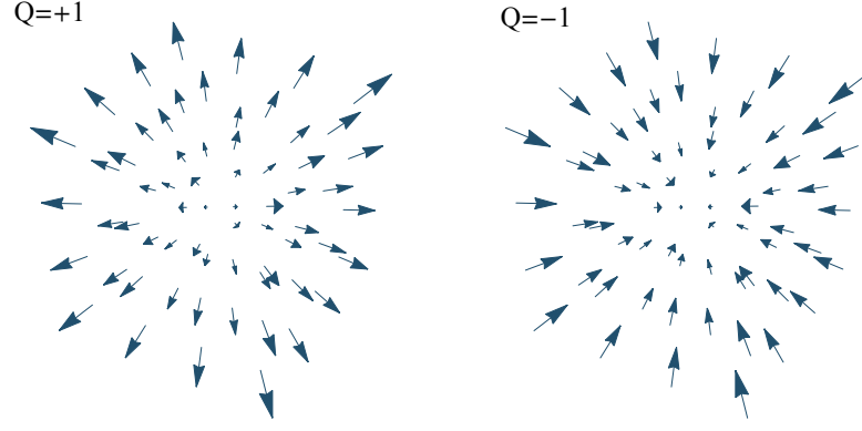
Fig. 3.47: Schematic view of dipole configurations showing ideal hedgehogs of charges Q = +1 (source-like) and Q = -1 (sink-like).
