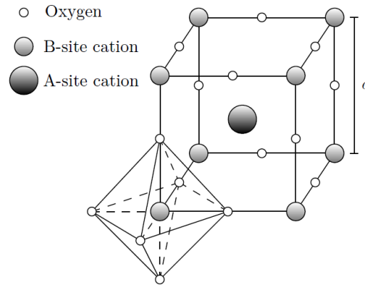
Fig. 1.1: Schematic view of the cubic prototype perovskite-type structure with the formula \text{A}^{2+}\text{B}^{4+}\text{O}^{2-} . The space group is Pm\bar{3}m with a lattice constant a \sim 4 \text{ \AA} .
