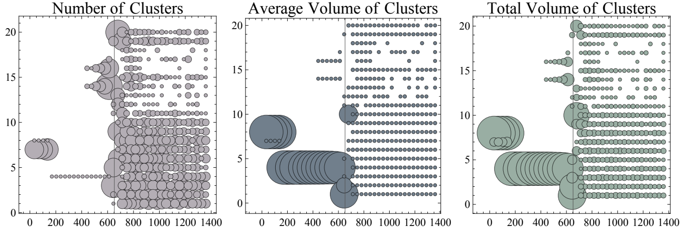
Fig. 3.33: PZ 60 T 40 : Temperature evolution of the number of clusters ( N_{Cl} ), their average volume ( V_{Cl}^{av} ) and their total volume ( V_{Cl}^{tot} ) per face. The y axis refers to the face label, the x axis denotes temperature. Let's first put our attention on the high-temperature region. (i) High temperatures are characterized by small values of N_{Cl} , V_{Cl}^{av} and V_{Cl}^{tot} for all faces. Thus spatial correlations are very weak, and all directions are equivalent. This is merely indicative of full disorder. (ii) While approaching T_C (indicated by a vertical line) from above, one observes signatures of critical fluctuations, such as emergence of preferred orientations (some directions are no longer represented while large spatial clusters corresponding to certain equivalent rhombohedral orientations appear) and scale invariance (indicated by the fact that differently populated directions acquire equal number of clusters). (iii) Below T_C , up to \sim 440 K, one observes the condensation of only several clusters oriented in [1, -1, 1] and [1, -1, -1] directions (faces 4, 14 and 16). Whereas the single cluster corresponding to [1, -1, 1] (major phase) direction stands out in terms of large volume, the clusters with [1, -1, -1] (minor phase) orientation are numerous and, in contrast, relatively much smaller in volume. This latter observation shows that below T_C the percolation of [1, -1, 1] clusters has been achieved, however the volume corresponding to the major phase is not simply connected. This situation is not persistent since a further decrease of the temperature drives this minor phase to gradually shrink, ultimately disappearing at 440K. (iv) At temperatures below \sim 440 K the ground state is achieved. It is important to mention that what could appear as a switching of direction is, in fact, only an artifact of Metropolis Monte-Carlo method.
