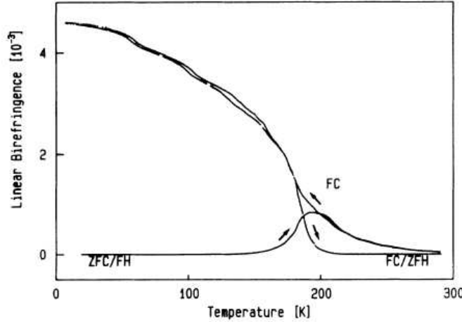
Fig. 1.19: Linear birefringence measured subsequently as a function of temperature on zero-field cooling (ZFC), field heating with E = 1.2\text{kV/cm} , E < E_{\text{cr}} (FH), field cooling (FC) and zero-field heating (ZFH), illustrating the nonergodic behaviour of PMN crystal. (After Kleemann et al. [123])
