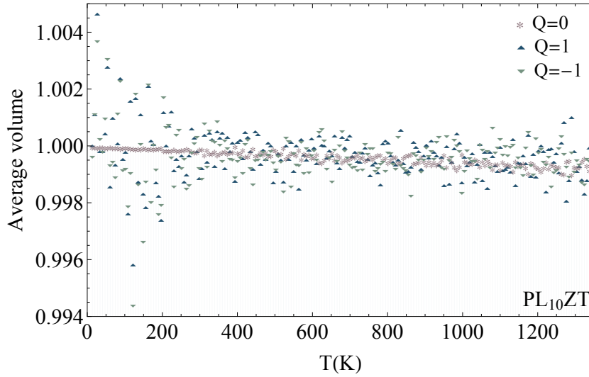
Fig. 3.56: Evolution with temperature of the average volume of zero-charged unit cells ( Q=0 ) and of topologically defective cells (with Q=1 and Q=-1 ) for \text{PL}_{10}\text{ZT} .
