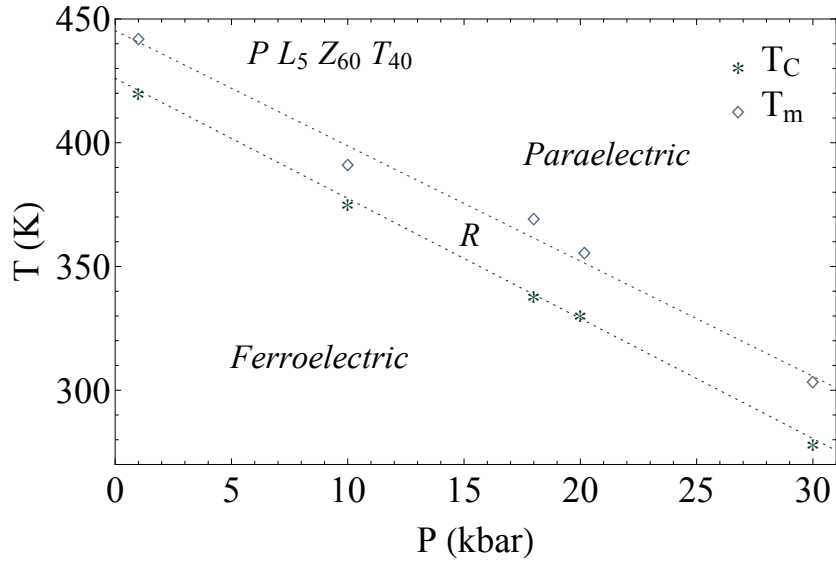
Fig. 3.42: Temperature-Pressure phase diagram for PL 5 Z 60 T 40 . Dotted lines delimit the relaxor region and their slopes are extracted from linear fits of the T_C and T_m data, dT_C/dP = -4.85 K/kbar and dT_m/dP = -4.66 K/kbar respectively.
