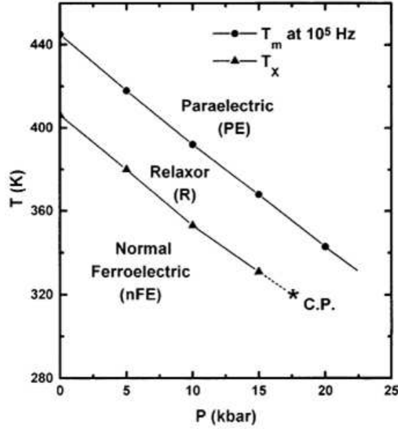
Fig. 1.40: Temperature-Pressure phase diagram of PLZT 6/65/35 (After Samara [104]).
