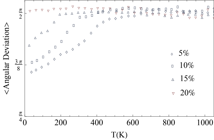
Fig. 3.29: Temperature evolution of the mean angular deviation between the local modes u_i and the local fields E_i^{\text{RF}} , for PL 10 ZT, PL 15 ZT and PL 20 ZT systems.
