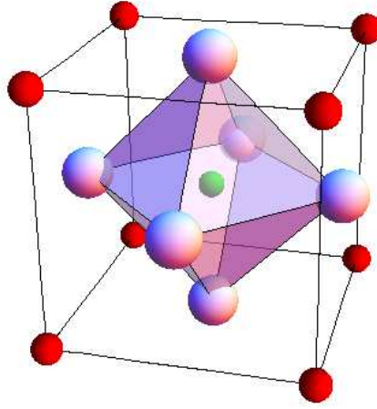
Fig. 2.20: Perovskite cubic structure ABO_3 , where A and B atoms are respectively located at the corners and in the center of the cube. The octahedra connect O atoms.
