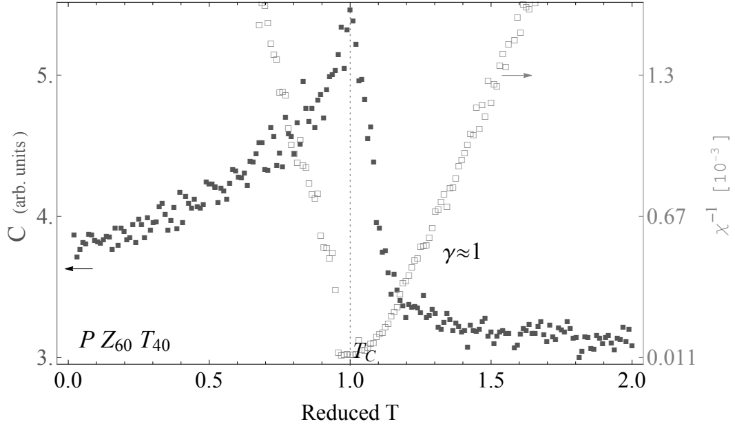
Fig. 3.11: Temperature evolution of the inverse dielectric susceptibility and the specific heat for \text{PZ}_{60}\text{T}_{40} . T_C = 652 K corresponds to the maximum of the specific heat and the reduced temperature refers to T/T_C . The inverse dielectric susceptibility at T > T_C can be well approximated to a Curie-Weiss form \chi^{-1} = C(T/\Theta - 1)^{-\gamma} with \gamma \simeq 1 and \Theta \simeq T_C .
