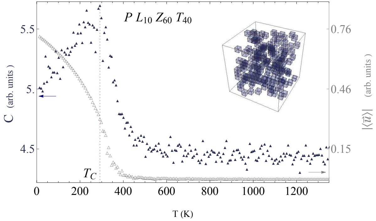
Fig. 3.3: Temperature evolutions of the specific heat (filled symbols) and the scaled polarization (open symbols) in PL_{10}Z_{60}T_{40} system. The inset shows the distribution of the quenched (lanthanum containing) unit cells inside the supercell. Dotted vertical line corresponds to T_C .
