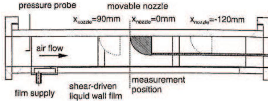
Figure 6.12 : Sketch of the experiment of Ebner et al. [73]
