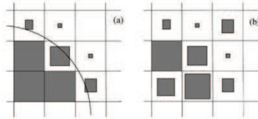
Figure 1.11 : Interface reconstruction in Volume Of Fluid methods. The liquid volume fraction is represented by shaded squares. Left: Straightforward reconstruction of the interface. Right: No clear determination of the interface. From Scardovelli & Zaleski [308]
