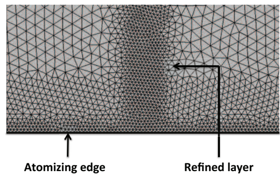
Figure 8.7 : Top view of the prefilmer surface mesh showing the FINE refined layer
