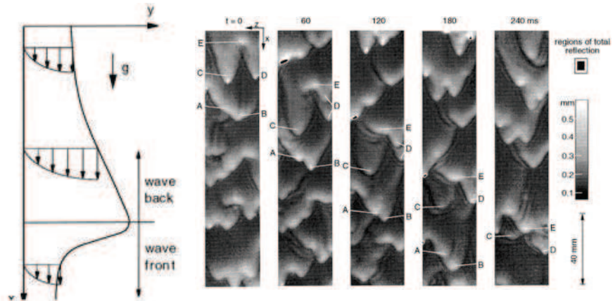
Figure 4.6 : Temporal development of 3D-wave structures at Re_l=27 , from [2]
