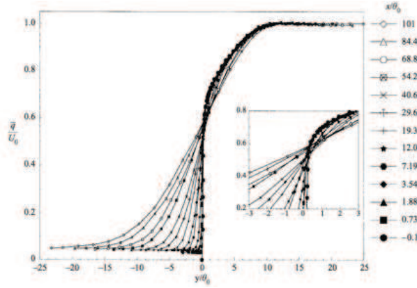
Figure 7.14 : Mean velocity magnitude normalized with the free stream velocity U_0 a plane versus the vertical position, for several horizontal locations, from [239]
