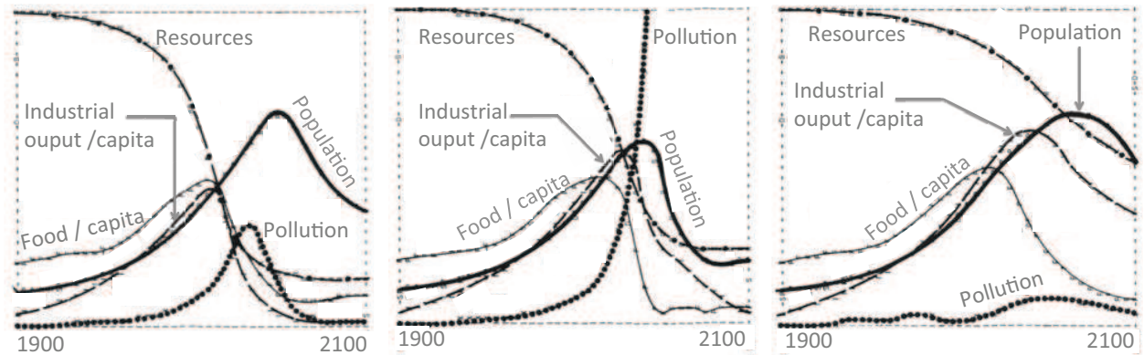
Figure 1.1 : Output from the LtG modeling for the three scenarios that span the technological and social response explored in LtG. Left: standard run. Middle: doubled natural resource reserves assumption. Right: unlimited resources and pollution control assumption. Adapted from [230]
