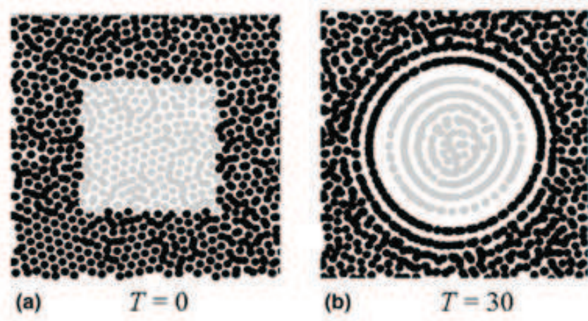
Figure 1.13 : Visualization of surface tension effect with SPH approach. Black and grey particles represent gas and liquid particles, respectively. a) Initial condition presents a non-equilibrium: particles located at the square corners undergo a stronger attraction towards the interior than particles located at the middle of faces. b) Equilibrium is reached when all interface particles are subject to the same attraction. From Tartakovsky & Meakin [338]
