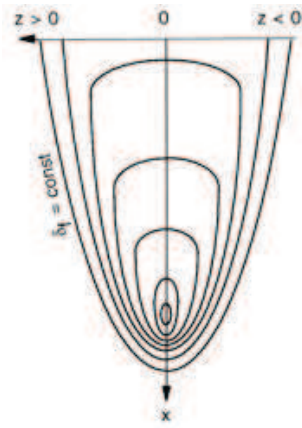
Figure 4.5 : Contour lines of the film thickness of an idealized 3D-wave, from [2]
