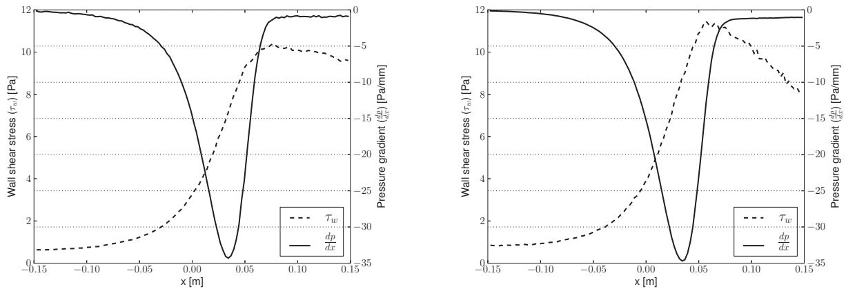
Figure 6.19 : Longitudinal profile of the wall shear stress and pressure gradient computed by AVBP on ITS1 (left) and ITS2 (right)
