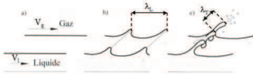
Figure 4.7 : Illustration of 3D structures arising from a Kelvin-Helmholtz instability, in a thick film configuration, from [152]
