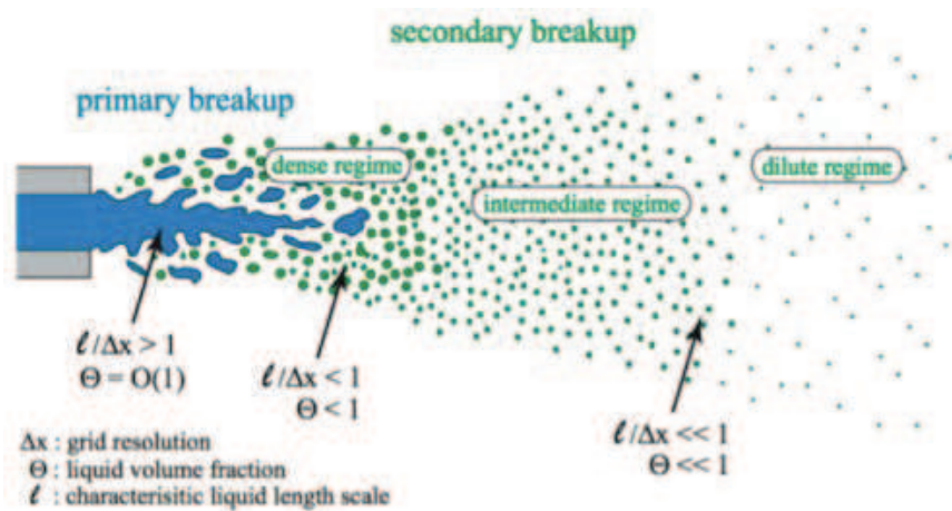
Figure 1.10 : Grid requirements related to characteristic length scales of the spray. (Source: M. Hermann, Summer Program of the CTR, Stanford).
