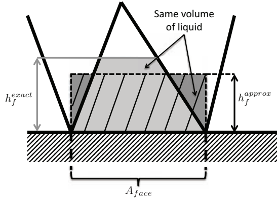
Figure 6.4 : Error associated to the no-scattering method on a regular mesh
