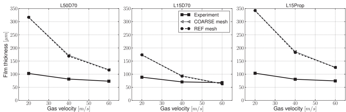
Figure 8.26 : Comparison of the mean film thickness with experimental data
