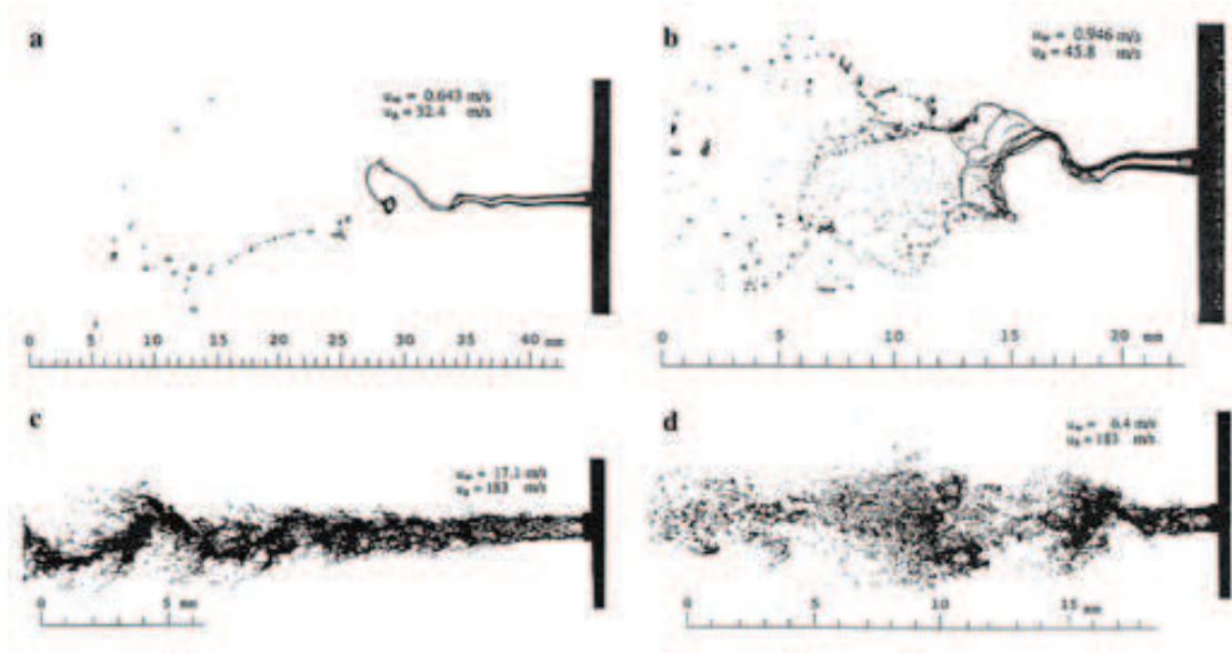
Figure 4.14 : Atomization regimes for an axial liquid jet in the presence of a coflowing gas stream, adapted from [80]
