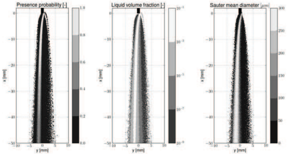
Figure 8.44 : Projection of spray characteristics for U60Prop REF
