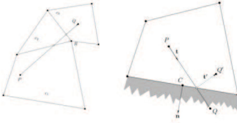
Figure 5.2 : Illustration of Haselbacher's algorithm, from [138]. Left: particle is initially located at point P and it travels to point Q . This algorithm tests every face of cell c_1 to check which one is crossed by PQ segment. Once the proper face is discriminated, the same process is applied to cell c_2 , and cells are iteratively tracked to Q position. Right: when the trajectory crosses a wall boundary, the trajectory is changed following an appropriate behaviour (from Q to Q' ) and the remaining path to achieve is updated.
