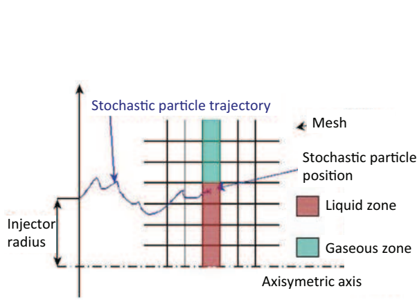
Figure 4.24 : Schematic of the phase reconstruction from the stochastic particle position, adapted from [167]
