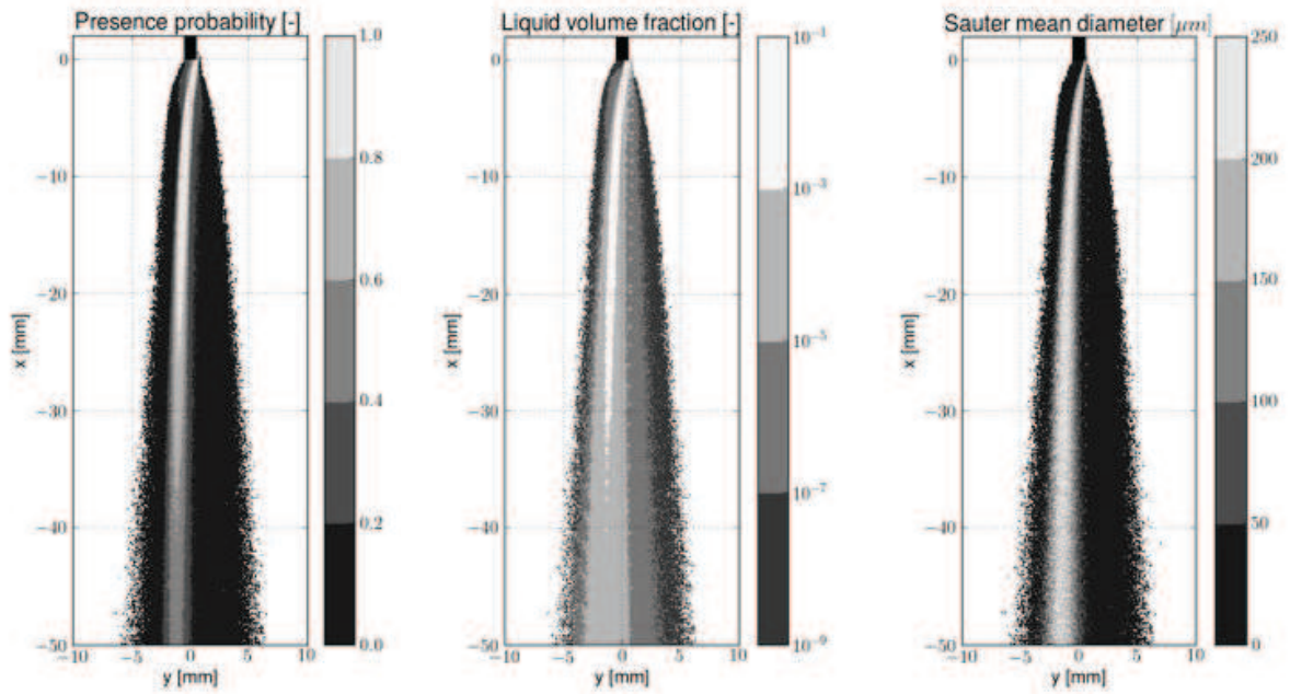
Figure 8.42 : Projection of spray characteristics for U60D70 REF
