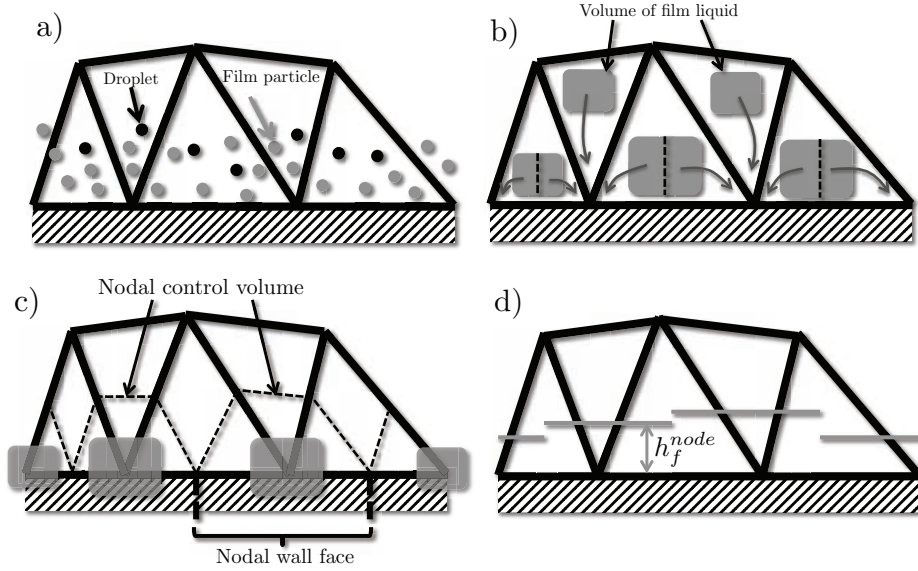
Figure 6.3 : Illustration of film thickness computation with scattering. a) Only film particles are accounted for the film liquid volume. b) Film liquid volume calculated in a) is equally distributed to surface nodes. c) Film volume at surface node (calculated in b)) is divided by the nodal wall surface. d) Resulting film thickness value is attributed at surface node.
