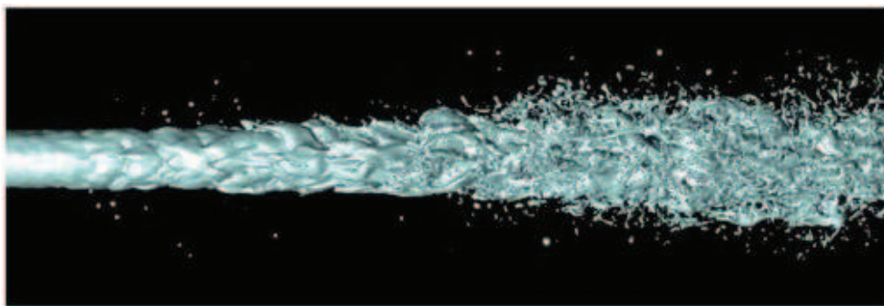
Figure 4.20 : DNS of the primary breakup of a turbulent jet, from [231]
