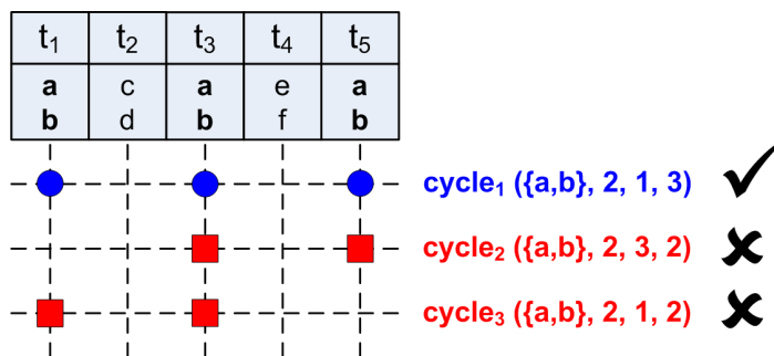
Figure 3.1: Examples of cycles and non-cycles
