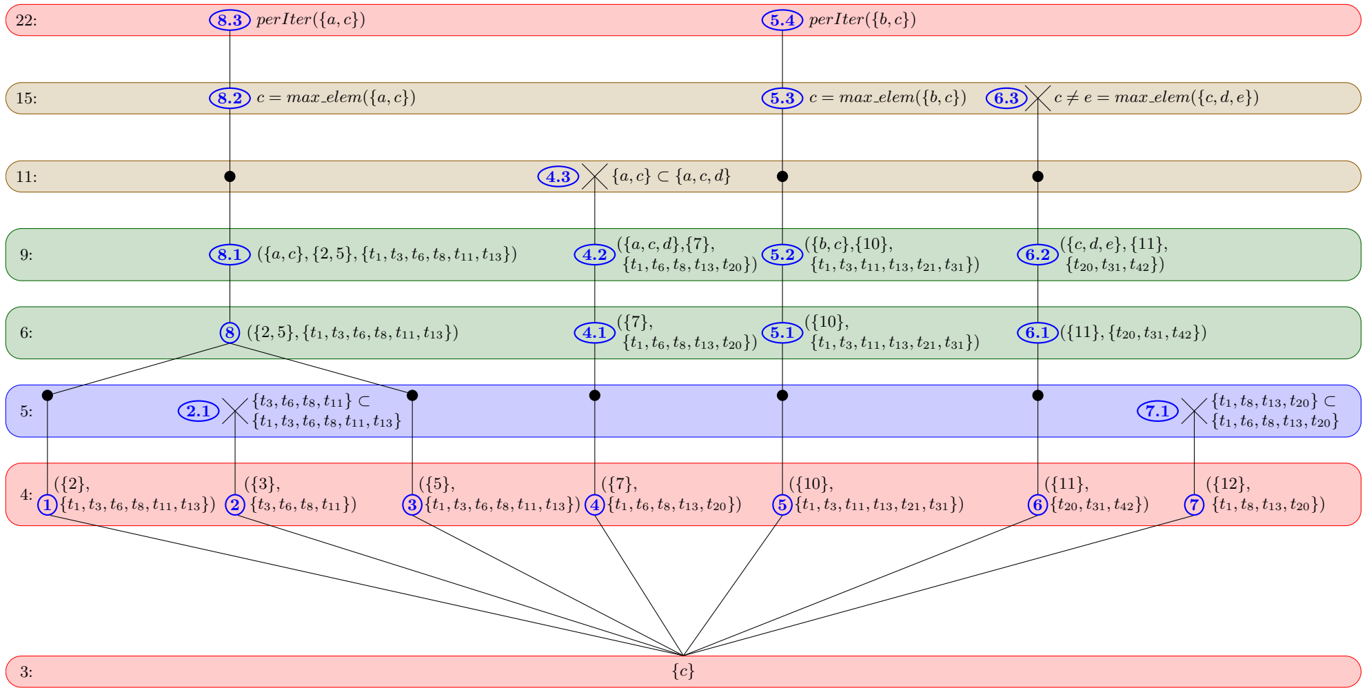
Figure 4.3: Graphical visualization of perIter execution
