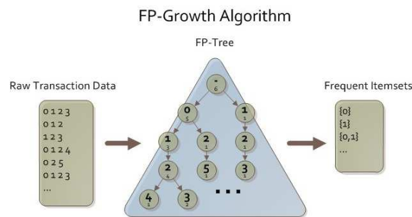
Figure 9.5: FP-growth
