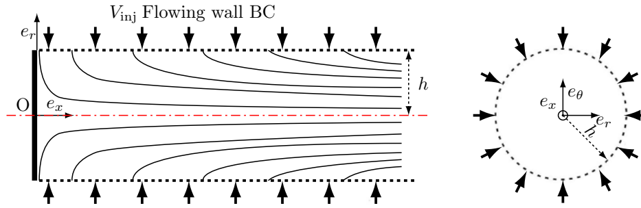
Figure 1.29: Parameters and analytical streamlines of the Taylor flow.
