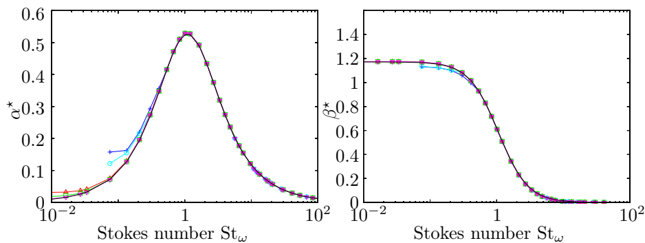
Figure 12.3: Attenuation and dispersion for different coupling time steps (Monochromatic wave, monodisperse spray, SAP1 code, K_p = 0.25 ) – Line: analytic; + : K_g = 2 ; o : K_g = 1 ; △ : K_g = 0.9 ; □ : K_g = 0.5 ; ▽ : K_g = 0.2 .
