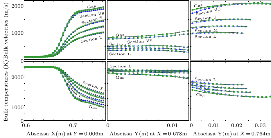
Figure 12.18: Velocities and temperatures along cuts (left: cut A-A, middle: cut B-B, right: cut C-C) – Solid: MF-PEG reference (BWC); \triangle : MF BWC; \square : MF ACS – Empty symbols: disperse phase; Full symbols: gas.
