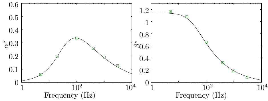
Figure 12.5: Attenuation and dispersion of a monochromatic acoustic wave in a polydisperse spray – Line : analytic; \square : SAP1 (ACS splitting, 10 sections).
