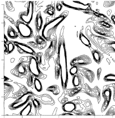
Figure 3.7: Number concentration contours in a one-way coupled turbulent flow (Squires and Eaton 1991b) showing segregation (or preferential concentration).
