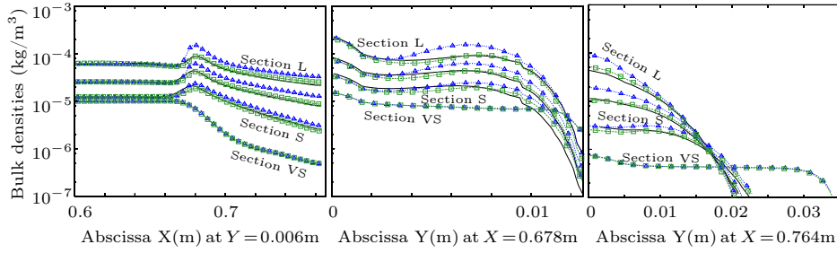
Figure 12.17: Particle mass concentrations along cuts (left: cut A-A, middle: cut B-B, right: cut C-C) – Solid: MF-PEG reference (BWC); \triangle : MF BWC; \square : MF ACS.
