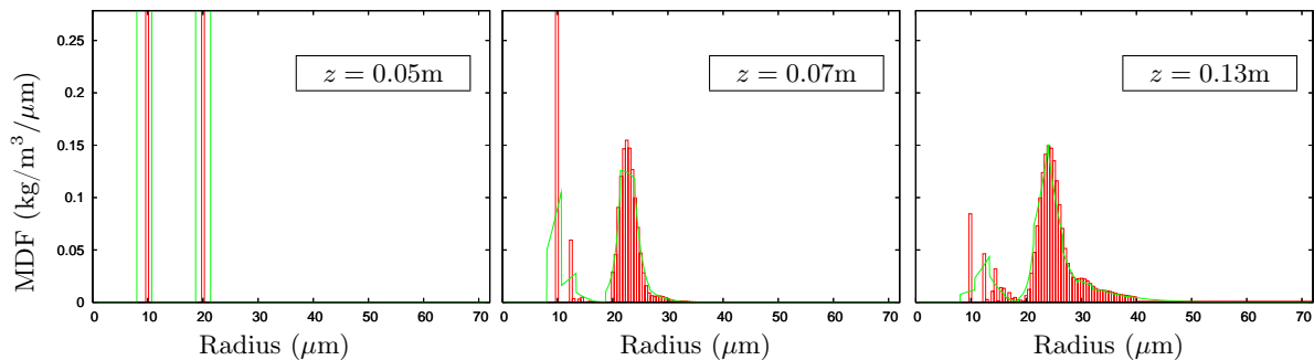
Figure 9.8: Mass concentration distribution at different abscissa - Boxes : One size moment hybrid MF with 80 sections; Line : Two size moment hybrid MF with 16 sections.
