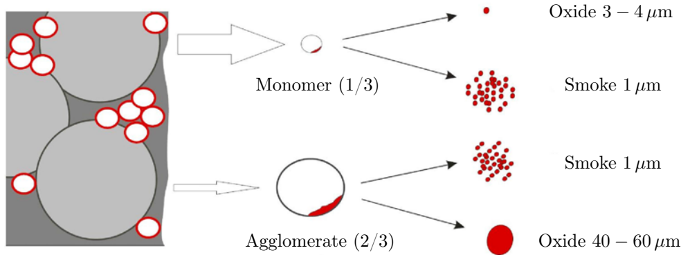
Figure 1.17: Aluminum and aluminum oxide dragging from propellant surface combustion (case of Ariane 5) – White: Metal Al, Red: Oxide (Duterque and Lambert 1998).
