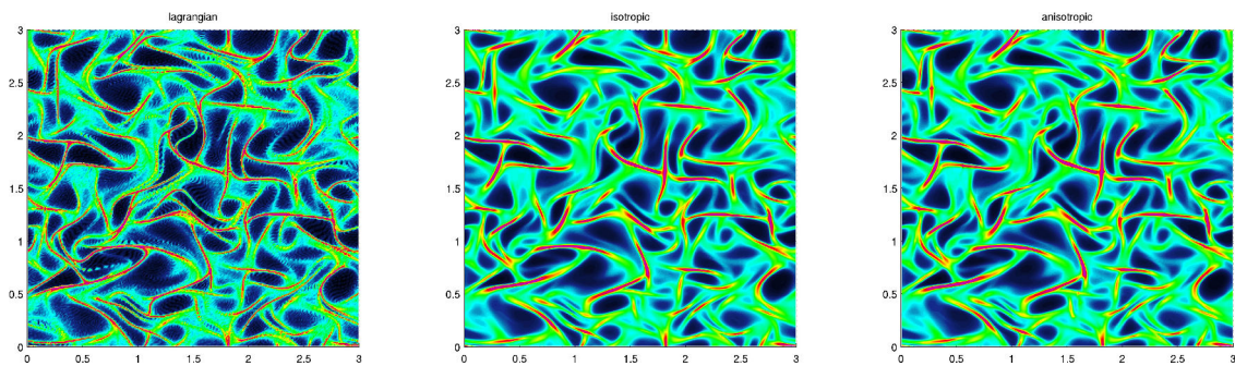
Figure 11.14: HIT case for St = 1 : number density field at time t = 3.6 for the stochastic-Lagrangian (left), and the Eulerian isotropic (center) and anisotropic (right) Gaussian closures.
