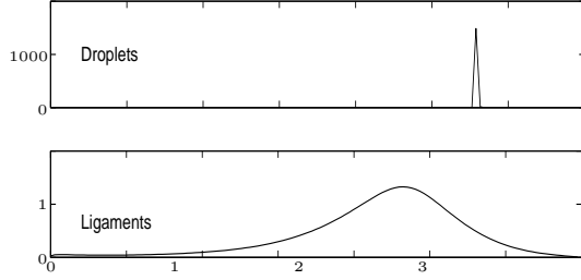
Figure C.6: NDF of droplets and of ligaments with the Two-Layer GPBE model.
