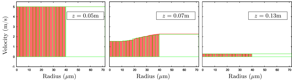
Figure 9.9: Velocity per section at different abscissae - Boxes: One size moment hybrid MF with 80 sections; Boxes: Two size moment hybrid MF with 16 sections.
