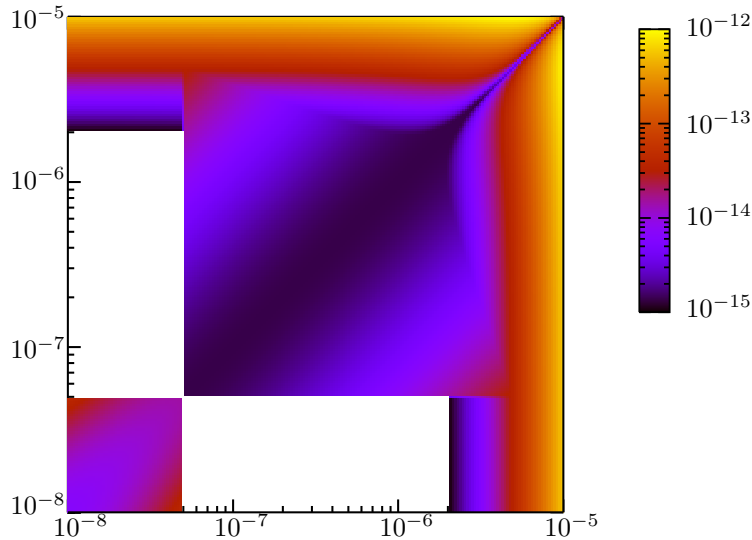
Figure 9.5: Polydisperse coalescence kernel ( m^3/s ) for monokinetic sprays ( u_g = 5 m/s , T_g = 3600 K , \mu_g = 96.10^{-6} Pa.s , \lambda_0 = 50 nm , \rho_l = 1600 kg/m^3 ) - The dif-kin domain has not been represented for no kernel is known.
