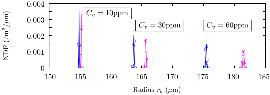
Figure 7.15: NDF after 2 m in a 10, 30 and 60 ppm fog – □: constant \beta model; ○: variable \beta model.
