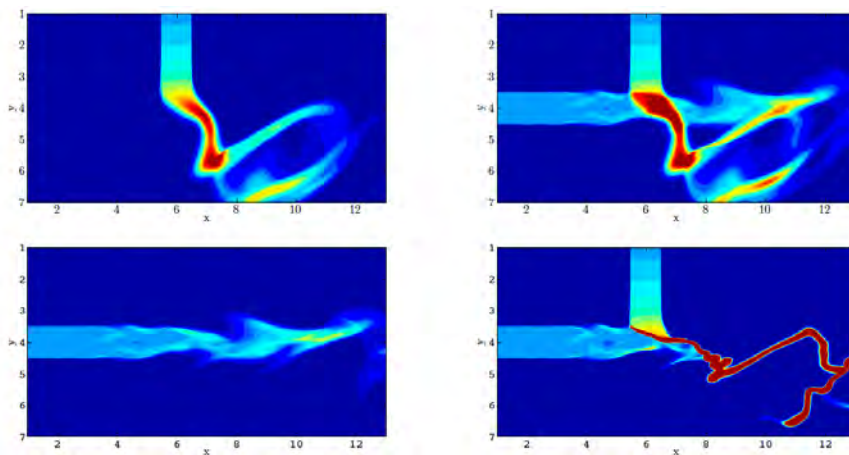
Figure 4.13: Total number density of two particle jets with MUSES3D – Top left: Vertical jet with EMVM; Bottom left: Horizontal jet with EMVM; Top right: Two crossing jets with EMVM; Bottom right: Two crossing jets with a monokinetic closure(Kah 2010).
