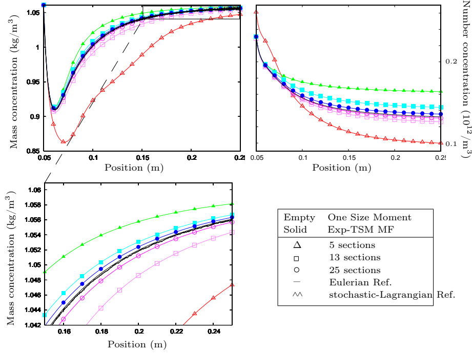
Figure 13.15: Top: Mass and number concentrations along nozzle – Bottom: close up view on the nozzle’s end.
