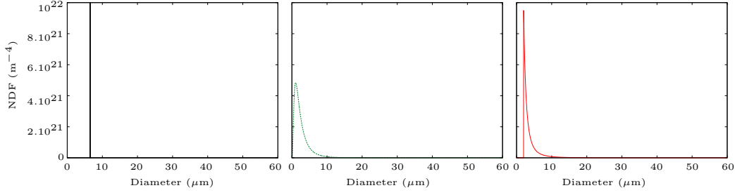
Figure 7.1: Different number density functions (NDF) with the same total bulk density and average diameter d_{31} – Left: Dirac size distribution (monodisperse); Middle: lognormal size distribution; Right: window size distribution.
