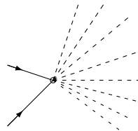
Figure 4.2: Statistical collisions yield ensemble velocity dispersion.
