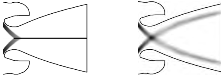
Figure 4.4: Illustration of a monokinetic or Kn = 0 crossing jet (left) versus a fully resolved Kn = +\infty crossing jet (right).
