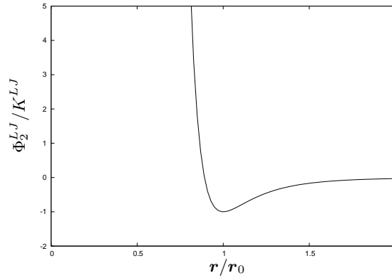
Figure 8.4: Lennard-Jones potential.
