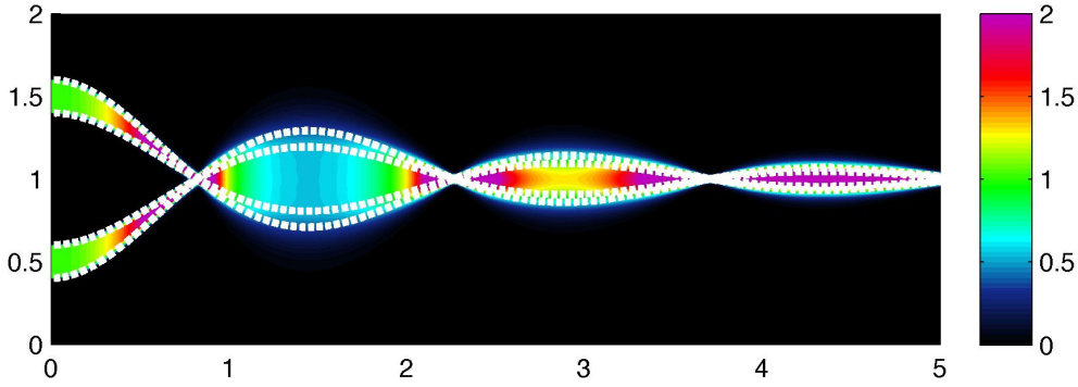
Figure 11.1: Steady solution of two inertial particle jets ( St = 20 ) injected in a compressive velocity field: Particle number density ( m^{-3} ). White lines represent the lower and upper Lagrangian trajectories for each jet.
