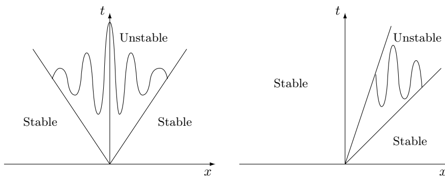
Figure 1.31: Absolute instability (left) and convective instability (right) in 1D space-time diagram.
