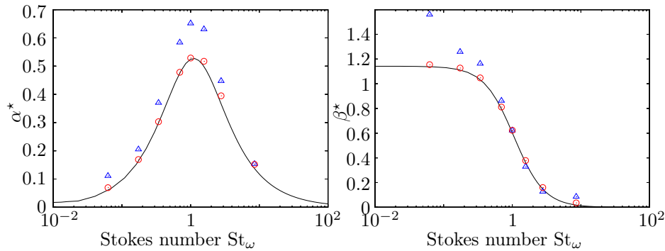
Figure 12.8: Attenuation and dispersion of a monochromatic acoustic wave in a monodisperse spray – Line: analytic; \Delta : CEDRE (BWC technique); \circ : CEDRE (ACS splitting).
