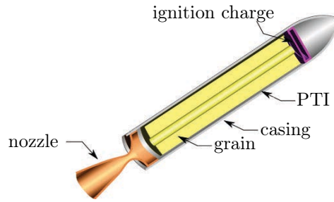
Figure 1.1: General structure of a SRM (source: Wikipedia).
