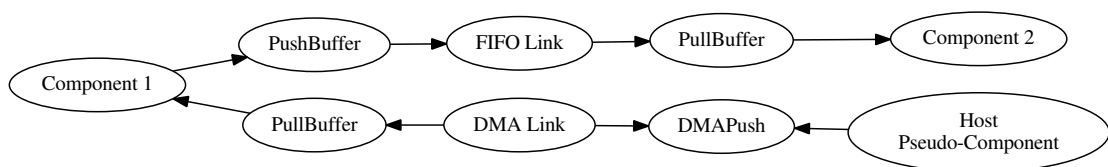
Figure 5.2: NPM Component Communication Interfaces.
