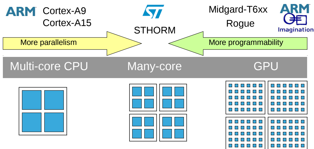
Figure 2.8: OpenCL as a Standard of Convergence
