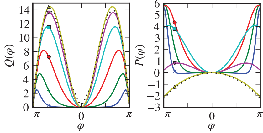
Figure 4.9: Phase dependence of the dissipative parts of the response at several temperatures: T/E_{Th} = 16(\Delta) , 8(\nabla) , 4(\square) , 2(\circ) , 1(+) , 0.5(\times) . The dotted lines represent the analytic high-temperature approximations to which Q and P tend for T \gg E_{Th} . Left: Function Q(\varphi, T) describing the phase-dependent dynamic contribution to the response. Right: Function P(\varphi, T) describing the phase dependence of the dissipative part of the admittance at low frequencies. After [95]
