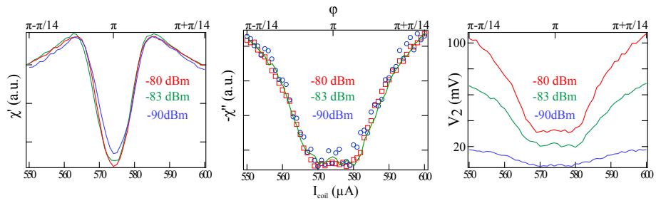
Figure 6.19: Close-up view of the response around \varphi = \pi at T = 445 \pm 2 \text{ mK} , f = 5 \text{ GHz} for several powers. In phase and out-of-phase responses do not depend on the applied power. There are small deviations at P_{\text{att}} = -100 \text{ dB} due to the looseness of the feedback loop. V_2 , the voltage of the 2 nd harmonics, changes with power, indicating that the applied power effectively changes.
