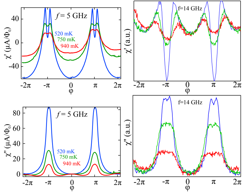
Figure 6.18: In-phase \chi' and out-of-phase \chi'' susceptibility at f = 5 \text{ GHz} and f = 14 \text{ GHz} for several temperatures.
