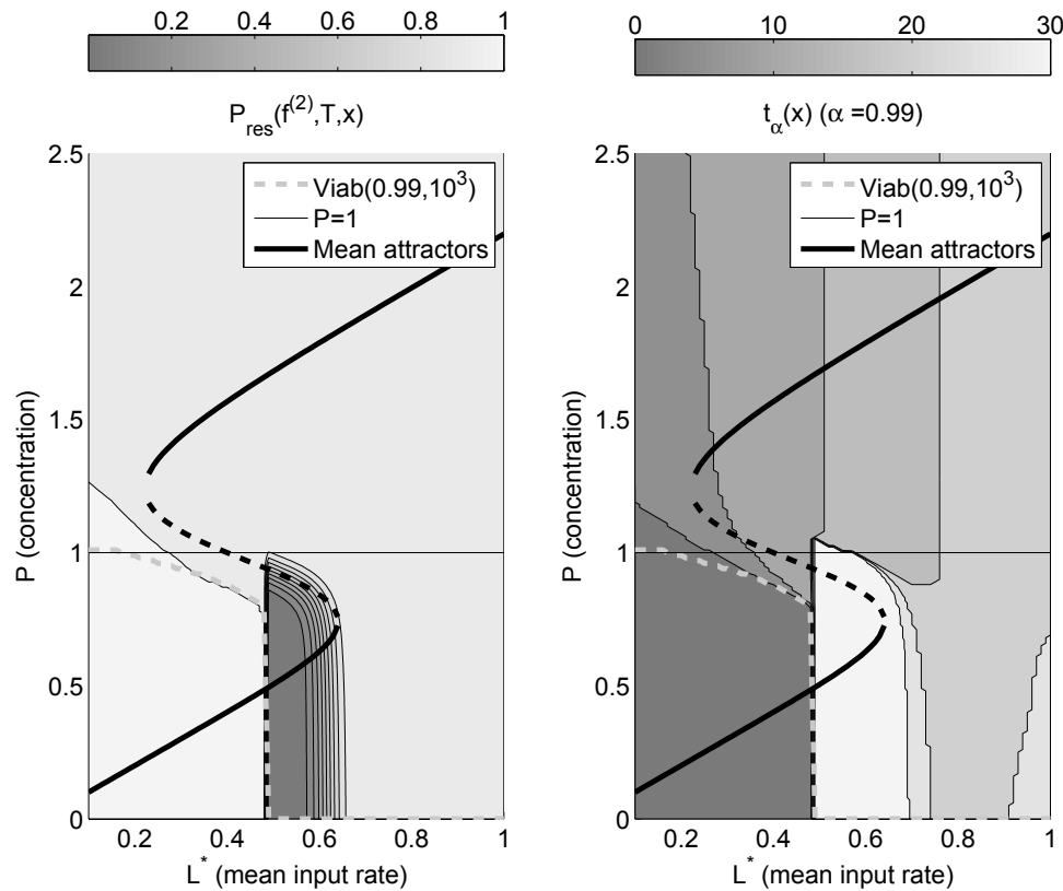
FIGURE 2.9 – Probability of resilience at T = 30 and entry time t_\alpha for strategy f^{(2)} . By default, t_\alpha(x) = 30 when the probability of resilience is smaller than 0.99 over the management horizon.
