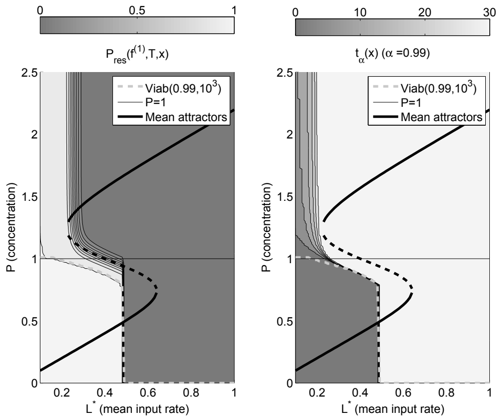
FIGURE 2.8 – Probability of resilience at T = 30 and entry time t_\alpha for strategy f^{(1)} . By default, t_\alpha(x) = 30 when the probability of resilience is smaller than 0.99 over the management horizon.
