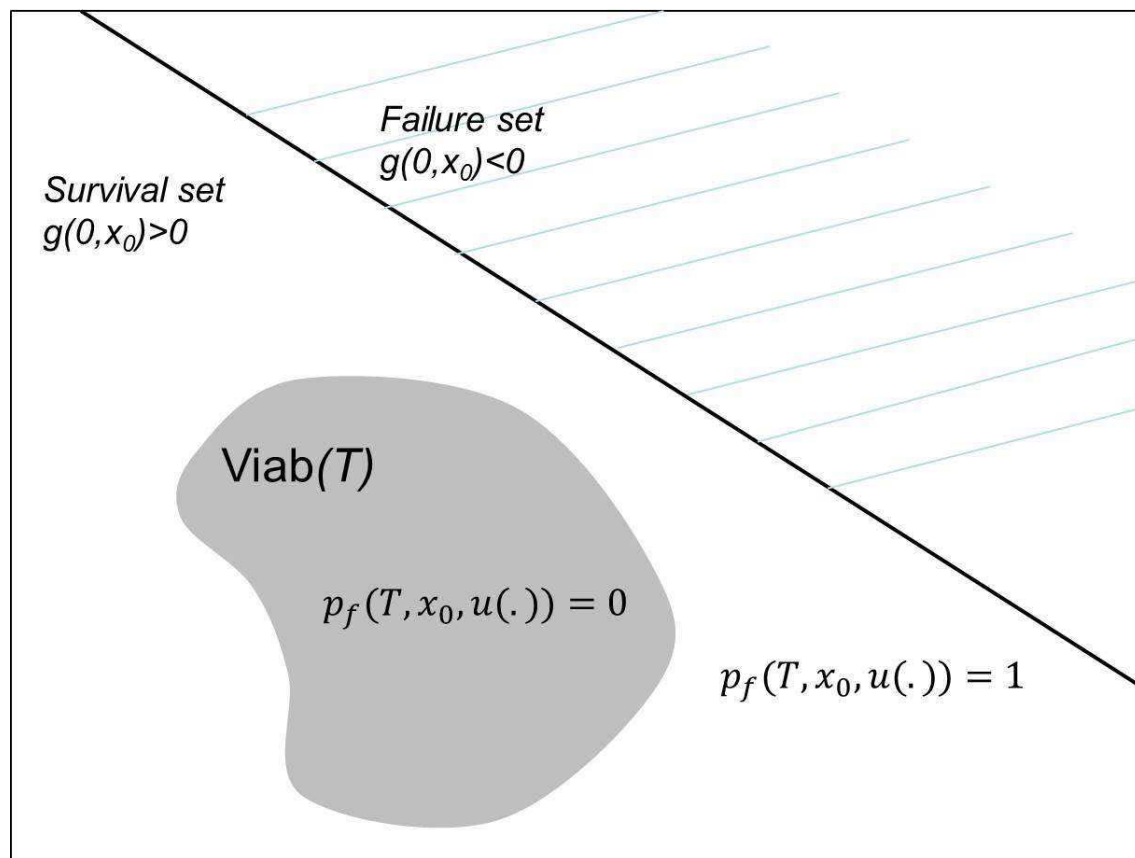
FIGURE 3.1 – Link between the viability kernel \text{Viab}(T) and the probability of failure p_f(T, x_0, u(.)) with deterministic controlled dynamics. All sets are represented at the initial date t = 0 .
