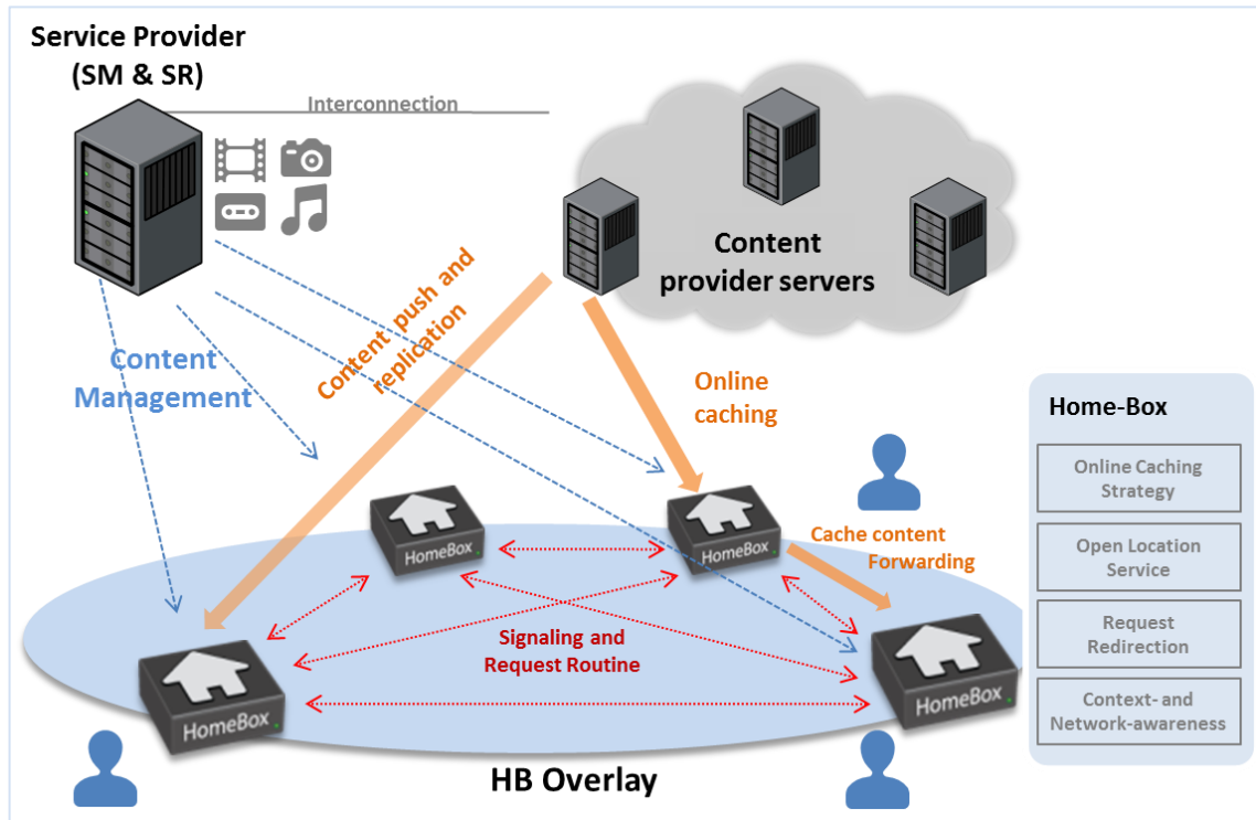
Figure 27: Online Collaborative Caching Approach
