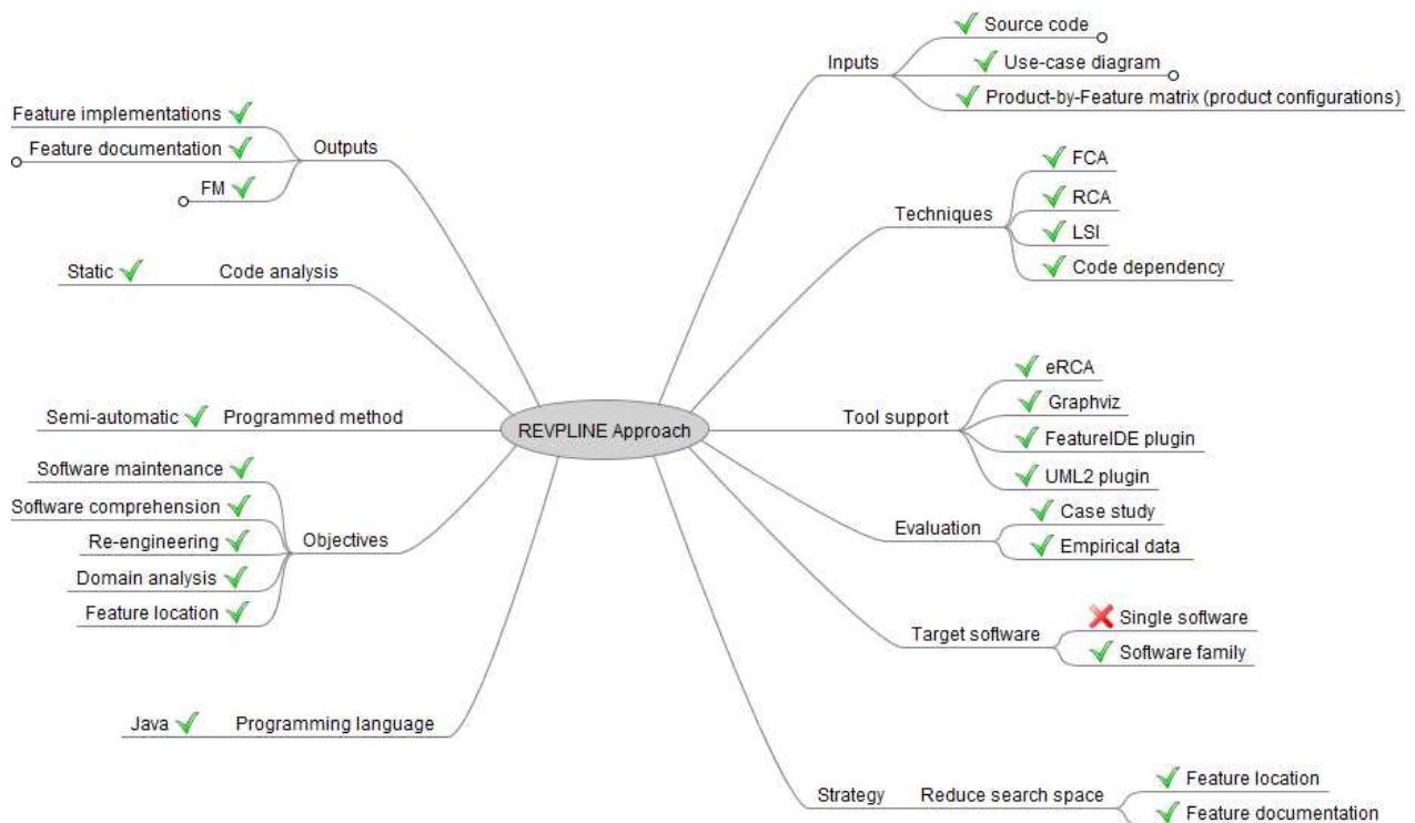
Figure 8.2 : The basic elements of REVPLINE approach.
