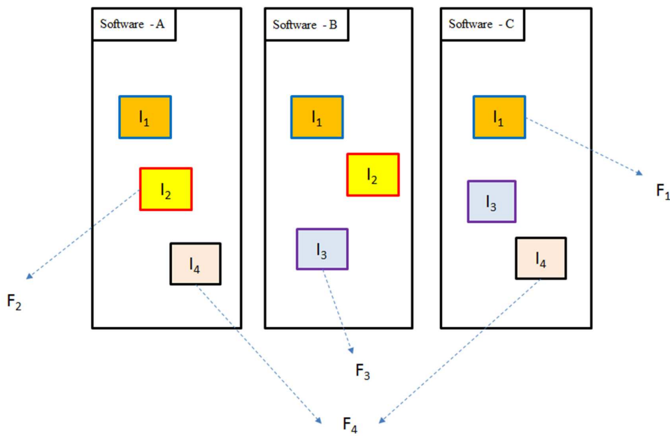
Figure 4.1 : Feature location in a collection of software product variants.
