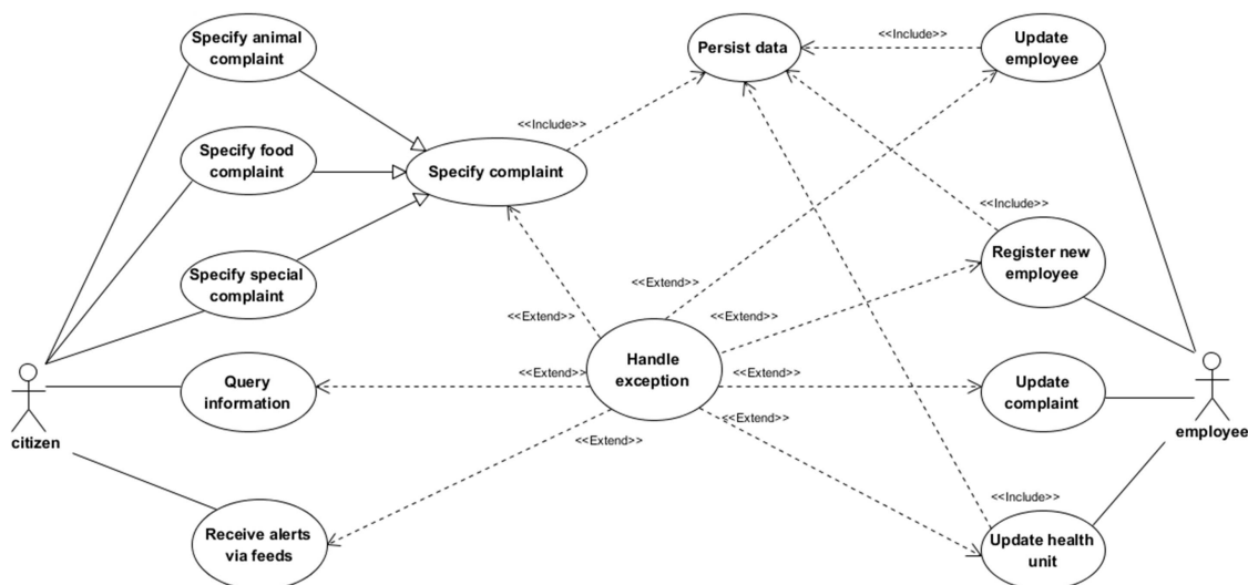
Figure 7.8 : Public Health complaint-SPL use case diagram.
