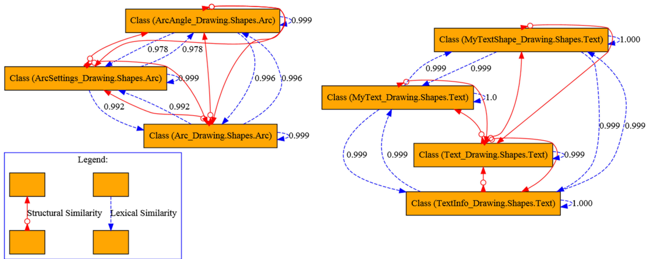
Figure 4.8 : The lexical and structural similarity between OBEs of ( Concept_1 ) in Figure 4.6 as a directed graph.
