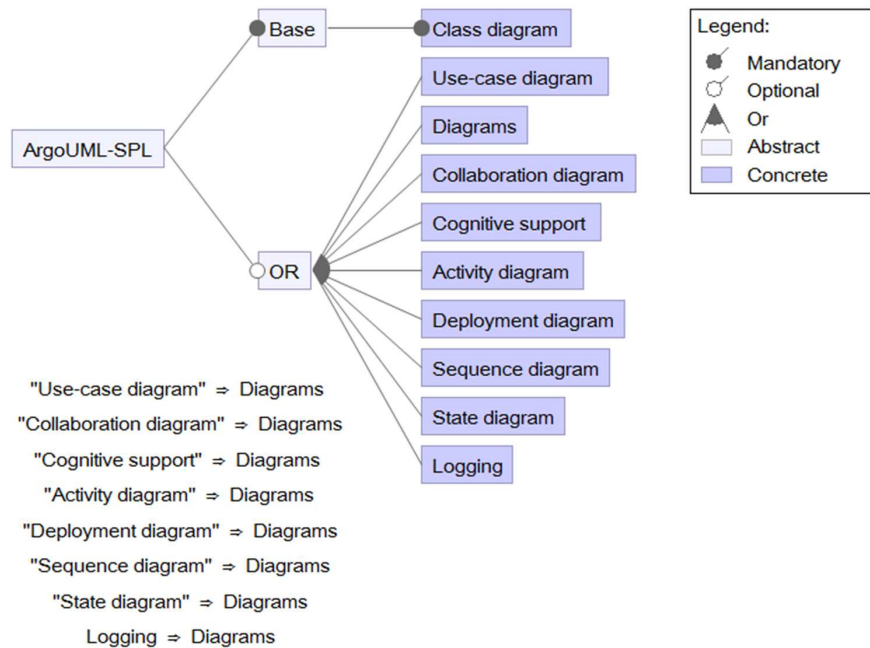
Figure 7.4 : The extracted FM from Table 7.9.
