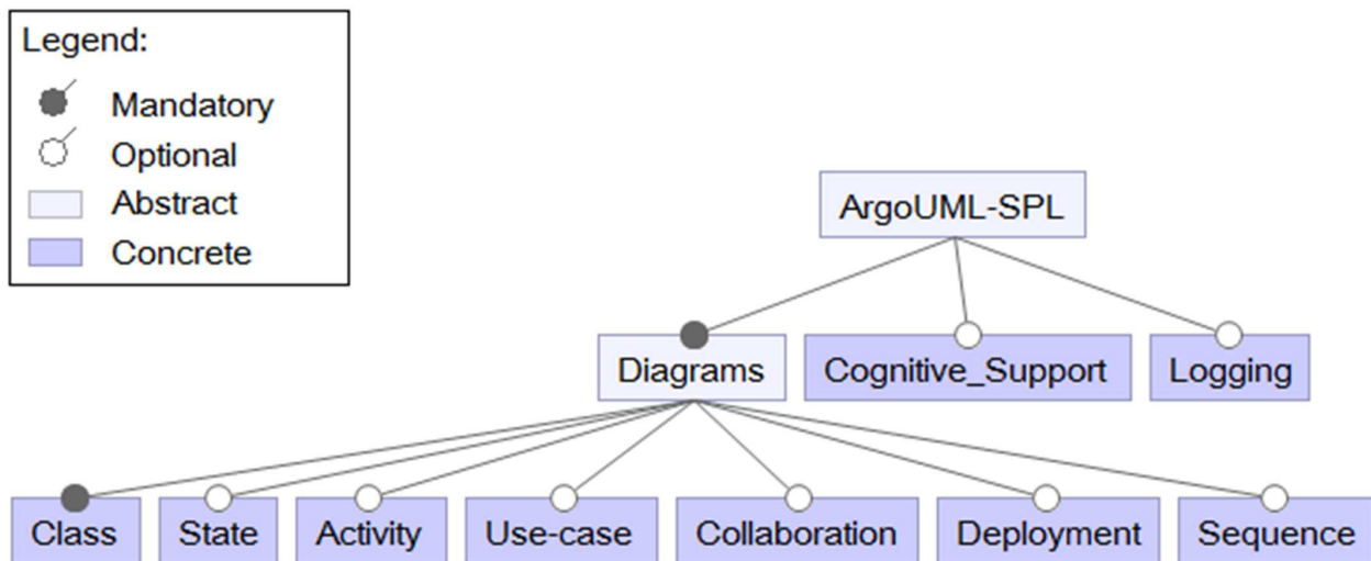
Figure 7.1 : ArgoUML-SPL feature model [Couto et al. , 2011].
