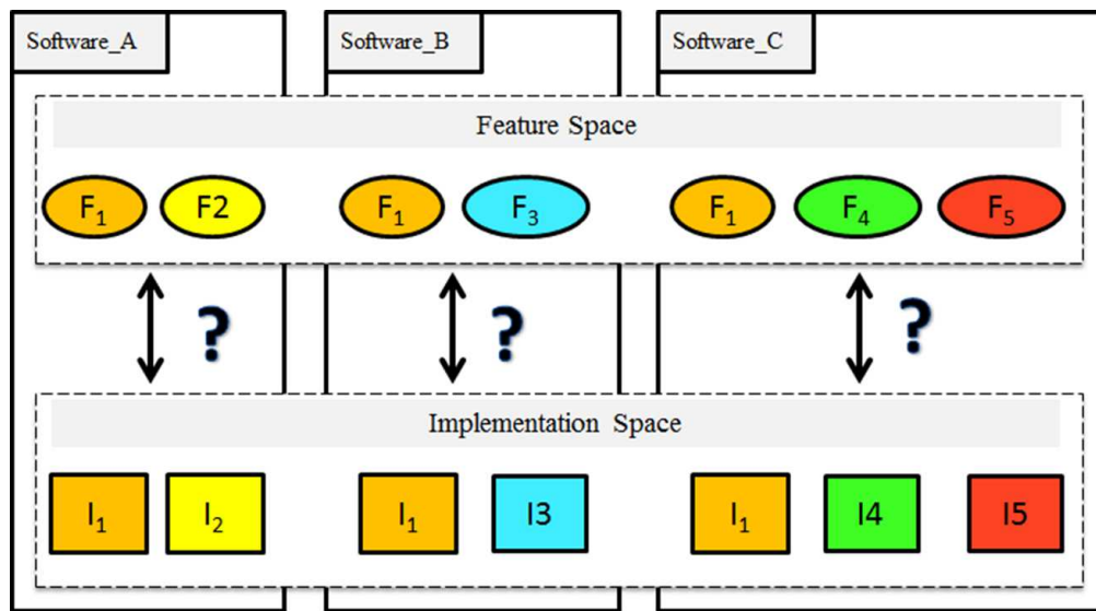
Figure 3.3 : Feature location in product variants.
