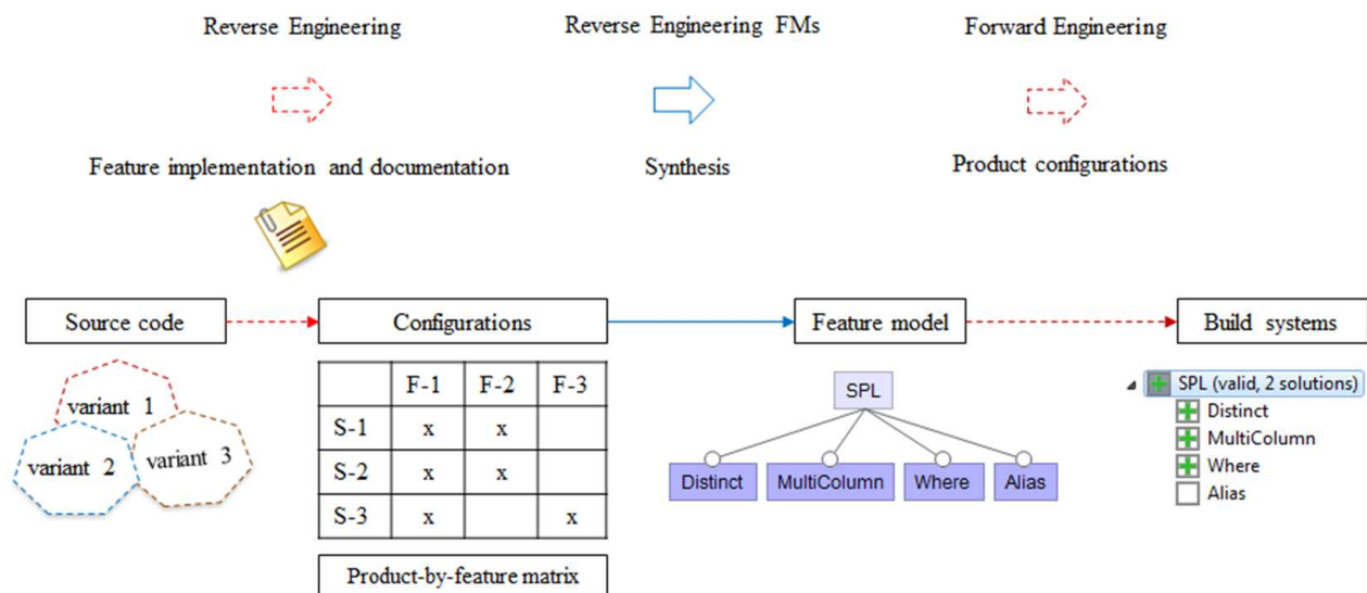
Figure 6.1 : From configurations to a feature model (inspired by [Acher et al. , 2013a]).
