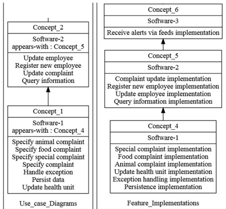
Figure 7.9 : Parts of the CLF of the RCF for feature documentation of health complaint software variants.
