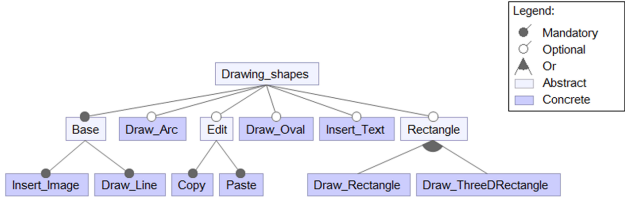
Figure 4.4 : Drawing shapes software variants feature model.
