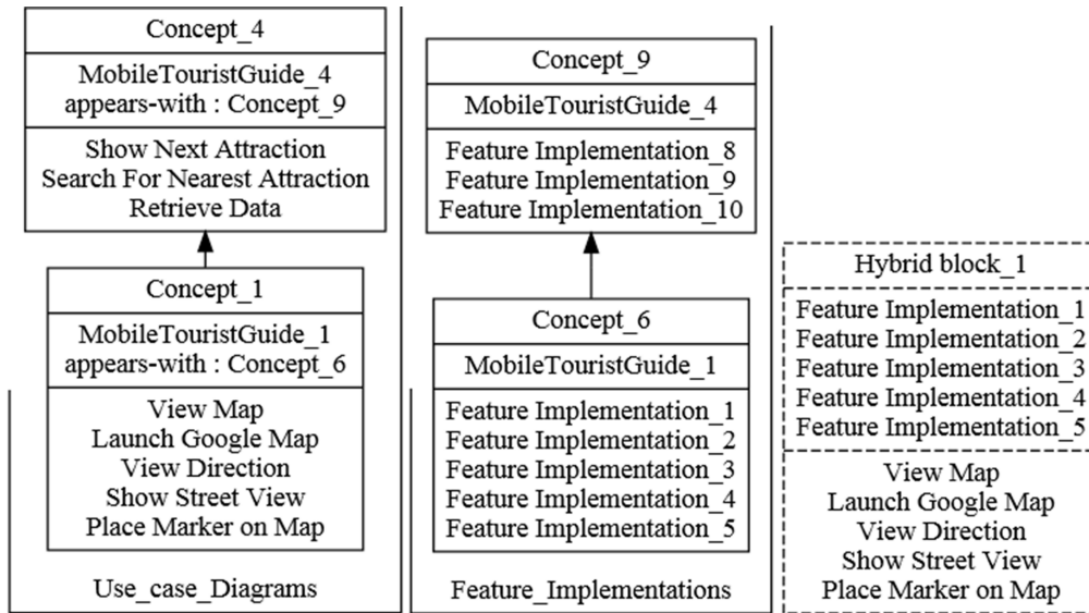
Figure 5.8 : Exploring and filtering the hybrid blocks CLF to identify features documentation.
