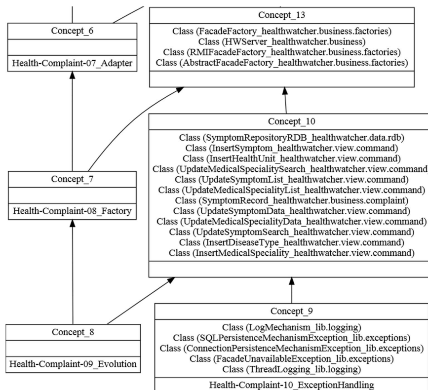
Figure 7.6 : Part of the AOC-poset of Health complaint-SPL.
