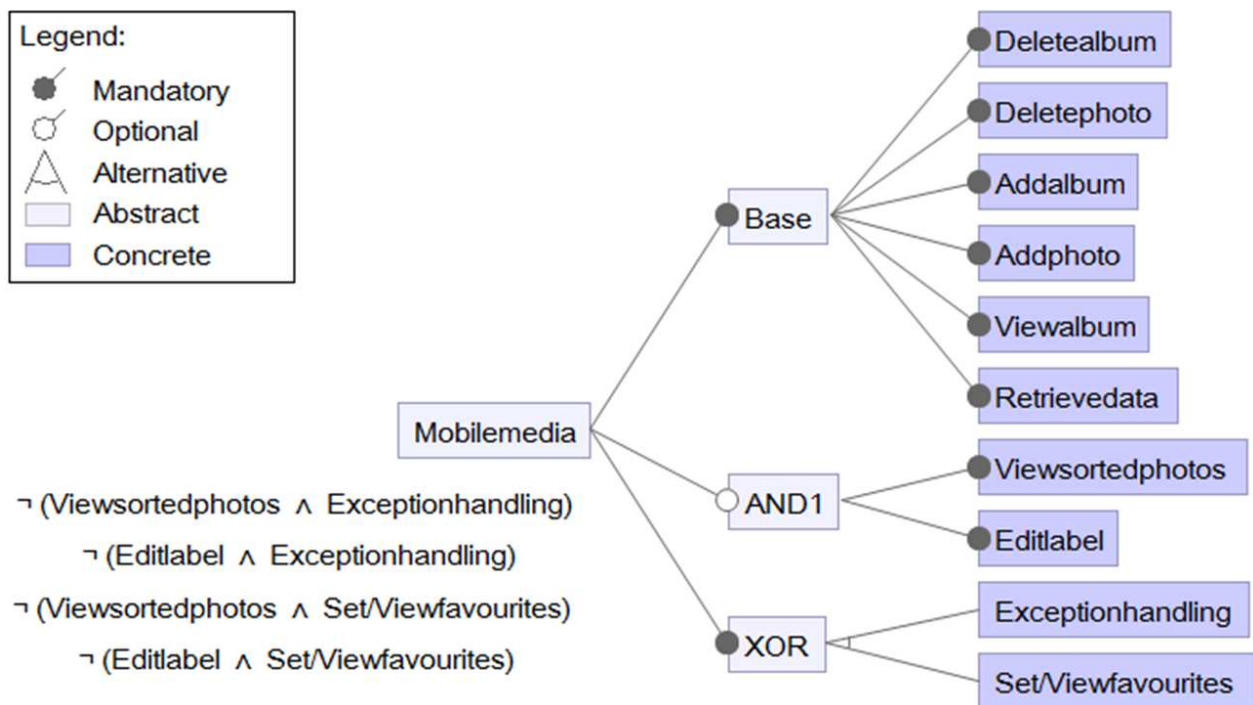
Figure 7.16 : The mined FM from the Mobile Media via FeatureIDE plugin.
