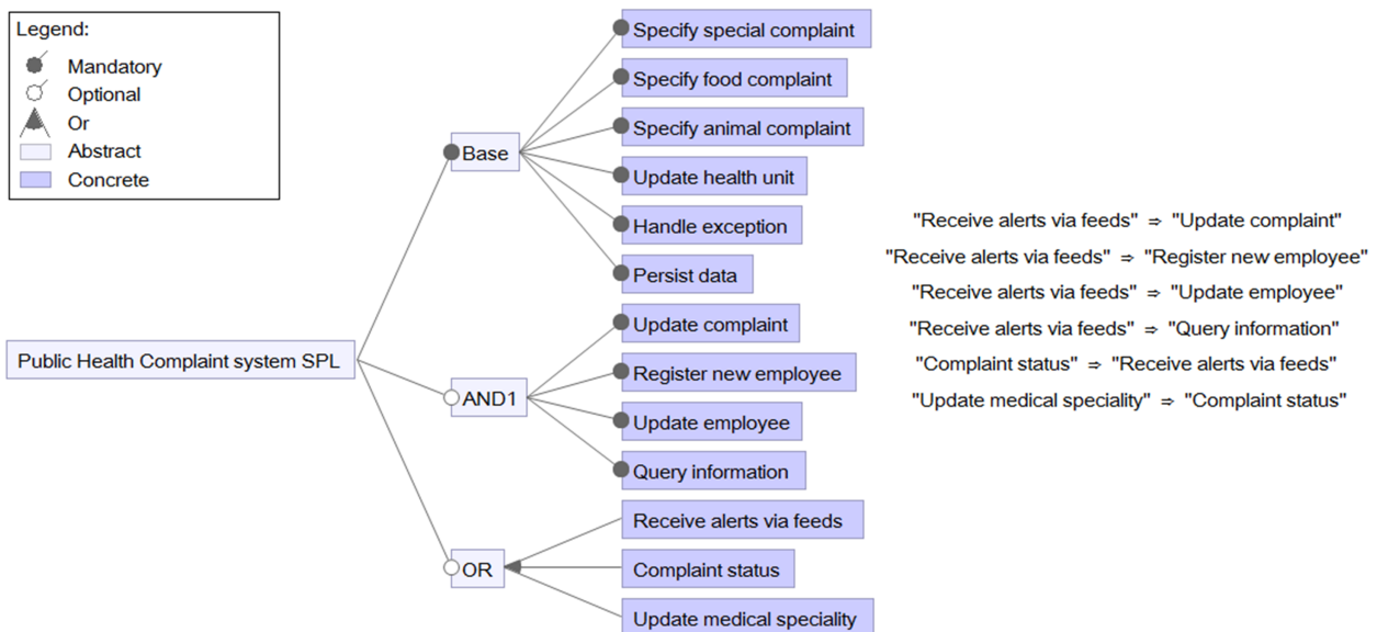
Figure 7.11 : The extracted FM from Table 7.14.
