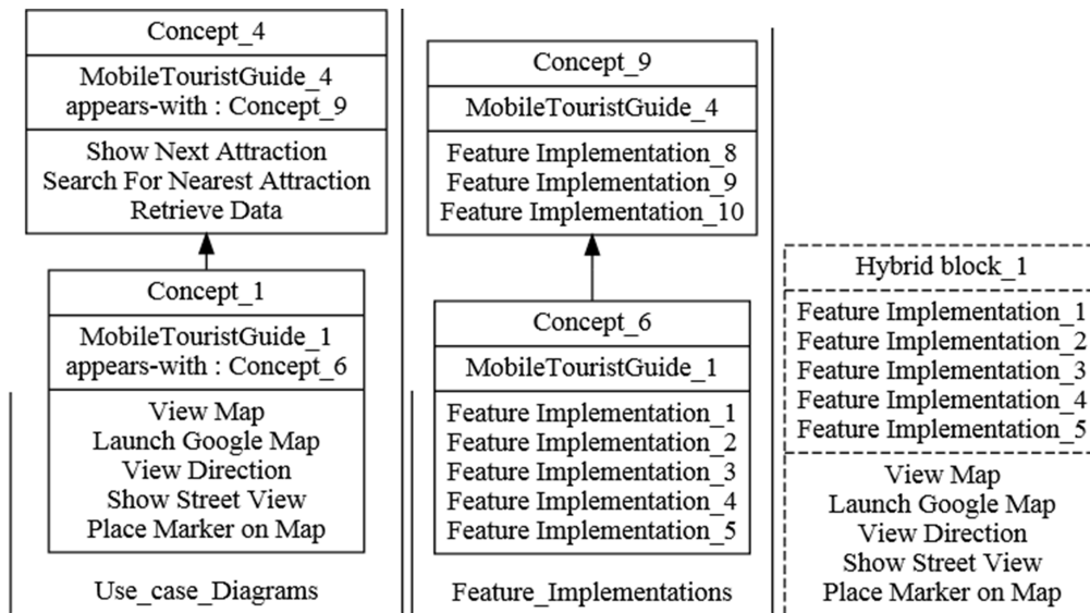
Figure 5.8 : Exploring and filtering the hybrid blocks CLF to identify features documentation.
