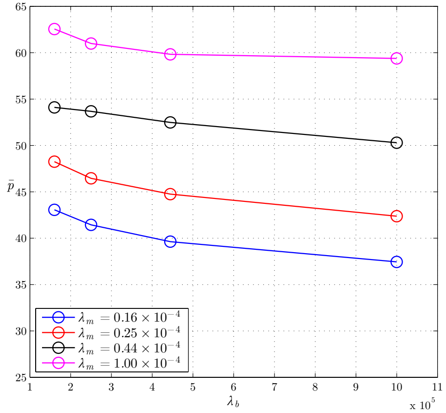
Figure 4.4: The CC Algorithm: Change of the average total power \bar{p} with respect to intensity of BSs \lambda_b for increasing values of intensity of mobiles \lambda_m = (0.16, 0.25, 0.44, 1.00) \times 10^{-4} \frac{\text{points}}{\text{m}^2} , A = 4 \text{ km}^2 , P_0 = 12 \text{ W} .
