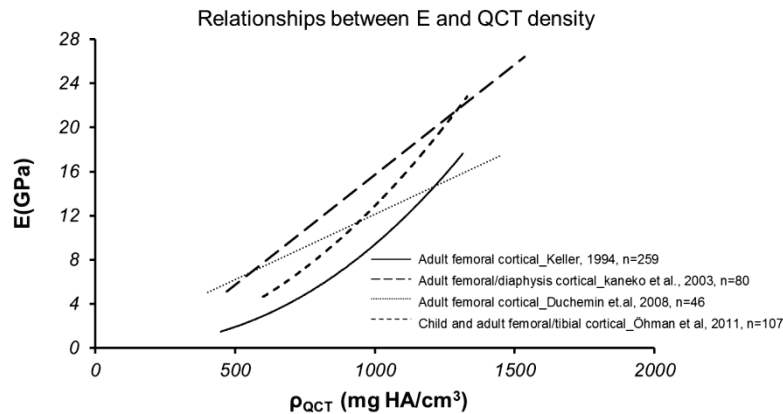
Figure 1.23: Relationships between Young's modulus ( E ) and QCT densities ( \rho_{\text{QCT}} ) (the data of Öhman et al., 2011 are derived from a combination of Öhman et al., 2011 and Kaneko et al., 2003).
