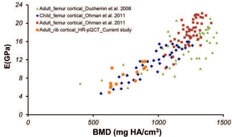
Figure 3.14: Correlations between the BMD and mechanical properties (the data of Öhman et al., 2011 are derived from a combination of Öhman et al., 2011 and Kaneko et al., 2003).
