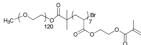
Scheme 1. Structure of PEO- b -PMEA copolymer
