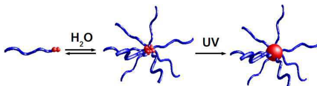
Scheme 2. Self-assembly and photo-cross-linking of block copolymer micelles.
