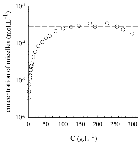
Figure 8. Molar concentration of star polymers as a function of the weight concentration of the polymers.
