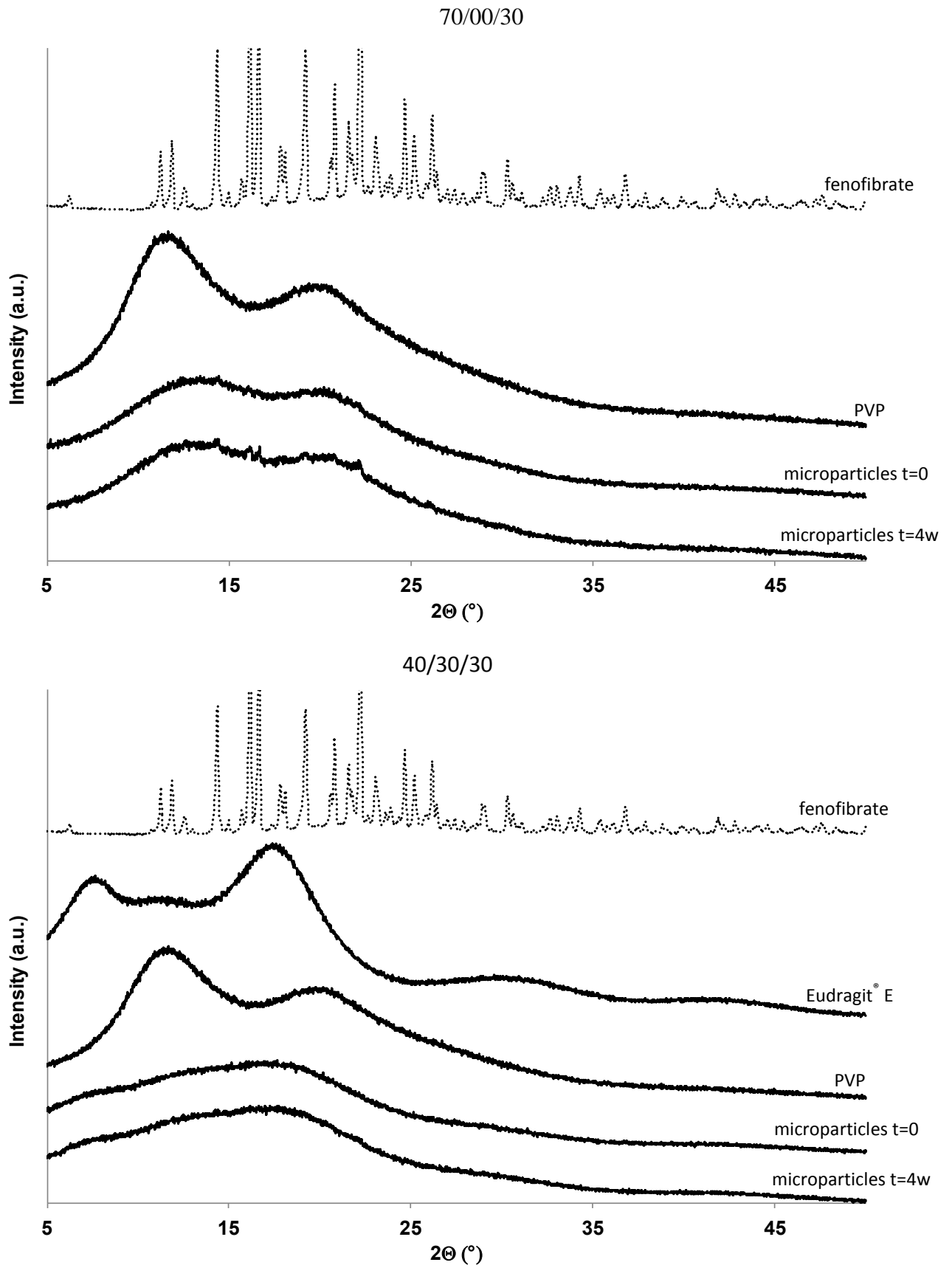
Figure IV.4 X-ray diffraction patterns of fenofibrate powder (as received), PVP powder (as received), Eudragit ® E powder (as received), and PVP/Eudragit ® E/fenofibrate microparticles containing 30 % drug (the composition is indicated in the diagrams) before and after storage (as indicated).
