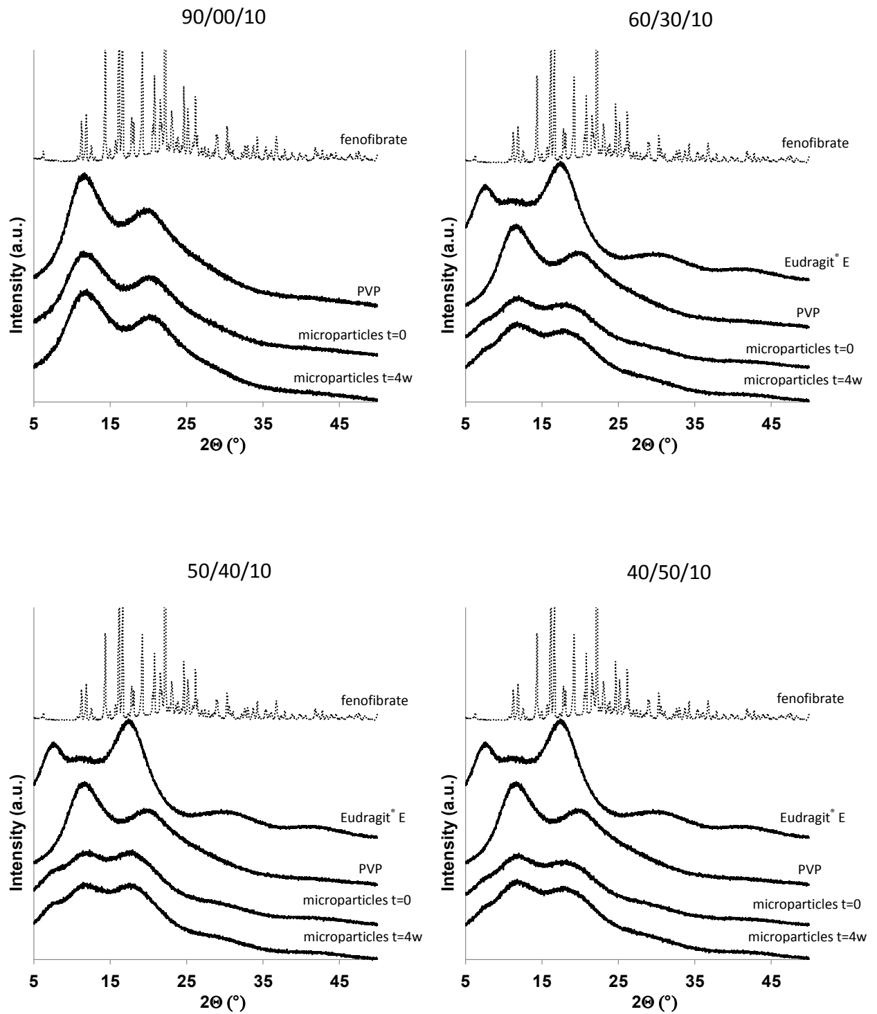
Figure IV.2 X-ray diffraction patterns of fenofibrate powder (as received), PVP powder (as received), Eudragit ® E powder (as received), and PVP/Eudragit ® E/fenofibrate microparticles containing 10 % drug (the composition is indicated in the diagrams) before and after storage (as indicated).
