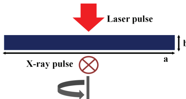
Fig 4.2 Schema of the APS setup with the crystal orientation.
