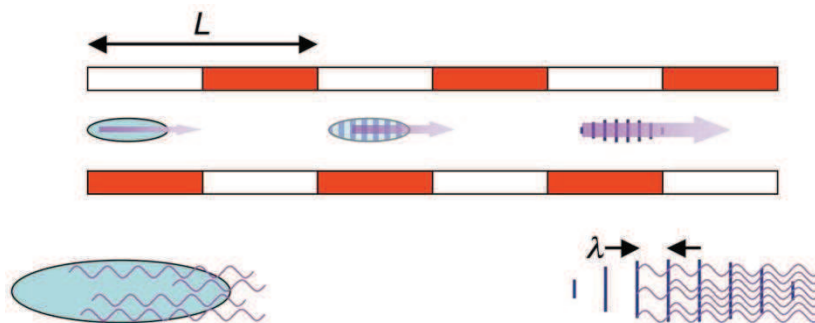
Fig 2.21 During the pathway, due to Lorentz force, electrons form bunch with X-ray periodicity.
