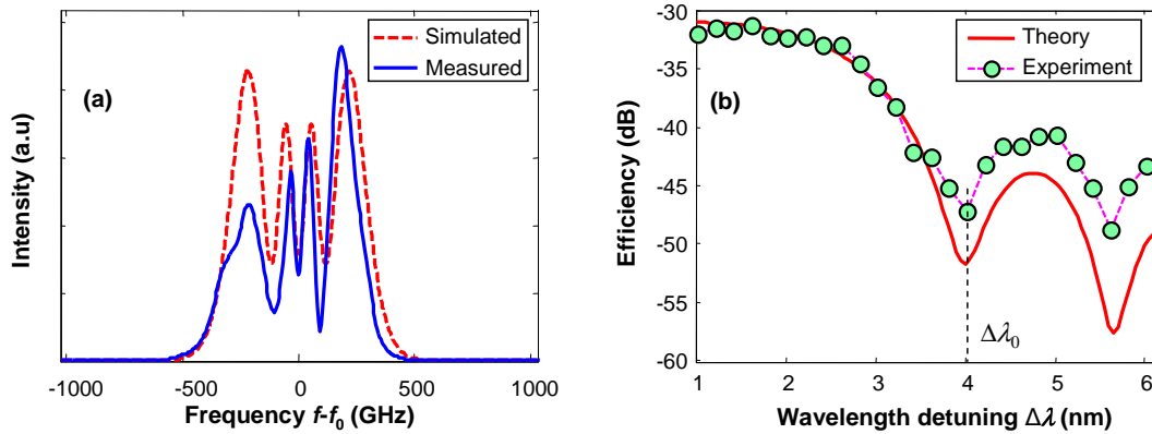
Figure 3.48: (a) SPM spectra at the output of the GeAsSe2011 fiber with the input peak power P_0 of 1.18 W, and (b) FWM efficiencies of two CW signals related to wavelength detuning \Delta\lambda .
