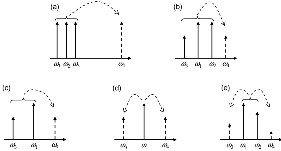
Figure 1.37: Five typical types of FWM.
