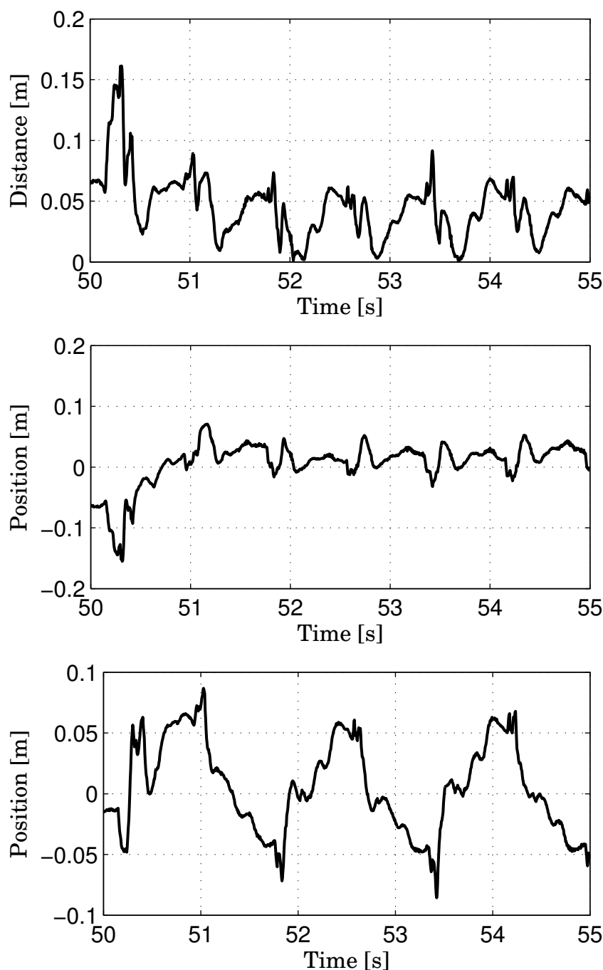
Figure 5.18: Distance to weighted middle point (top) and vector ZMP-weighted middle point ( x and y components: middle and bottom respectively), between t = 50s and t = 55s . The total experiment goes from t = 45s to t = 80s . These values are less discontinuous than the two previous sets of data.
