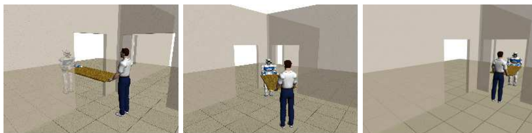
Figure 3.1: Example of scenario. The human-robot dyad has to carry the table through two doors that form a 90° angle. The dimensions of the table are too big to perform the task with a single bend, so that the human has to pass backward through the first door and forward through the second one. The human assumes the leadership of the task as he is walking backward through the first door, and then is guided by the robot through the second door.
