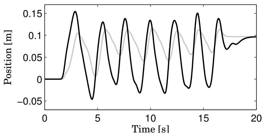
Figure 5.41: Gripper's vertical intended (grey) and effective (black) trajectories with the proactive control scheme.
