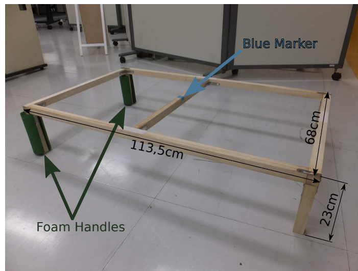
Figure 4.2: Object to transport jointly and its dimensions. The beam is made of wood, reinforced with steel brackets at corners. 2cm-thick green foam handles are added on the robot side so that the robot can safely grasp the object. The total weight is 1.6kg. A blue marker is added at the center of the table: the task is over as soon as this marker aligns with (i.e. reaches) the second doorway (See Fig. 4.3).
