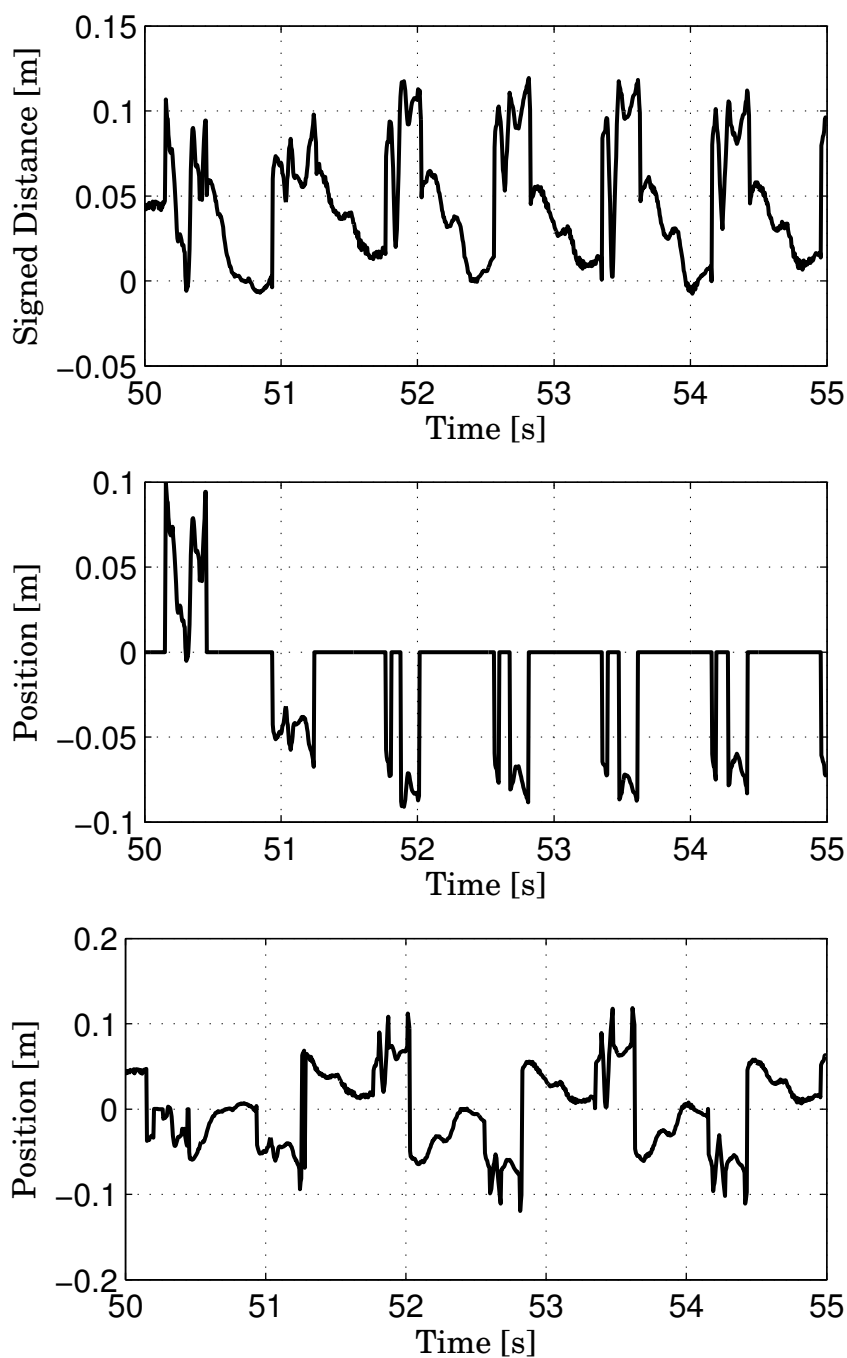
Figure 5.14: Signed distance to the support polygon (top) and vector that realizes this distance ( x and y components: middle and bottom respectively), between t = 50\text{s} and t = 55\text{s} . The total experiment goes from t = 45\text{s} to t = 80\text{s} . The main observation is that these values are highly discontinuous.
