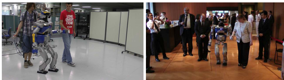
Figure 5.36: HRP-2 being guided by the hand in a lab environment (left) and at the French Embassy in Japan on July 14th 2012 (right).
