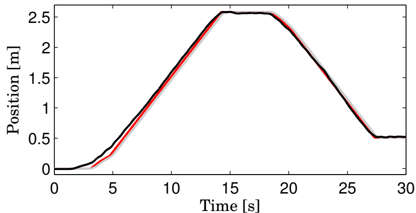
Figure 3.7: Trajectories of the object: the admittance controller output X in black, follower desired trajectory X_d in gray, motion primitives \mathcal{X} in red (integral of \mathcal{V} ).
