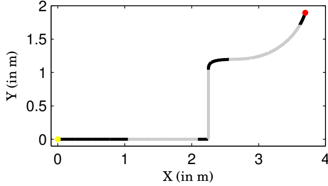
Figure 3.11: Example of desired trajectory from yellow dot to red dot. The sequence of primitives is Stop , Walk , Walk (with a different \mathcal{V} ), Stop , Side , Walk , Walk/Turn , Stop . The alternation of black and gray pictures the alternation of primitives. The sequence of \mathcal{V} used is given by Table 3.2.
