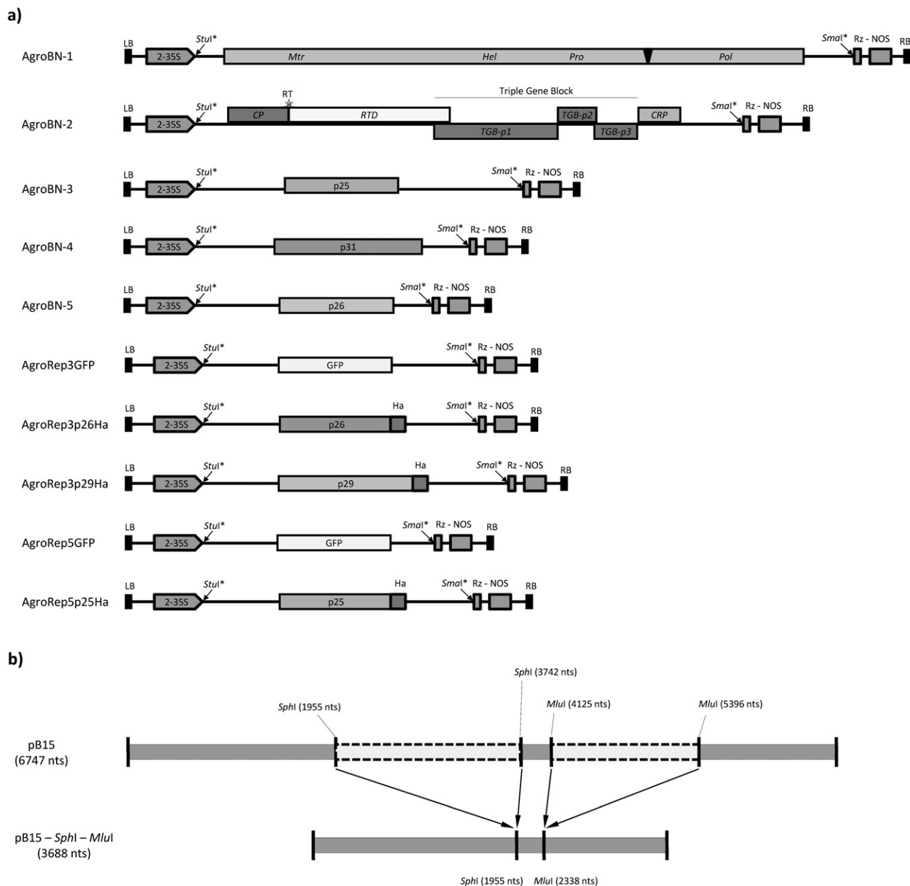
Fig. 1 (a) Beet necrotic yellow vein virus (BNYVV) constructs built and used in this study. Each clone has the same pJL89-derived backbone. Double Stul / Sma I (*) restriction digestion allows the insertion of blunt-end polymerase chain reaction (PCR) fragments between the double 35S promoter (2-35S) and the hepatitis delta virus ribozyme (Rz) followed by a Nos terminator. LB and RB represent the left and right borders of the T-DNA. Mtr, methyltransferase; Hel, helicase; Pro, protease; Pol, RNA polymerase; RT, readthrough; RTD, readthrough domain; star, suppressible UAG stop codon; CRP, cysteine-rich protein; GFP, green fluorescent protein; Ha, haemagglutinin tag. (b) Schematic representation of pB15 and pB15- Sph I- Mlu I clones used for the production of AgroBN-1. Broken lines represent segments between restriction sites Sph I and Mlu I removed from BNYVV RNA-1 clone (pB15) in order to facilitate cloning in the pJL89- Sph I plasmid.
