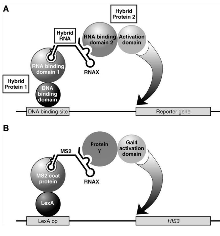
Fig. 3.2: Schematic illustration of yeast three hybrid test. (A) General strategy of the system. (B) Specific proteins and RNA components used (adapted from Bernstein et al. , 2002).
