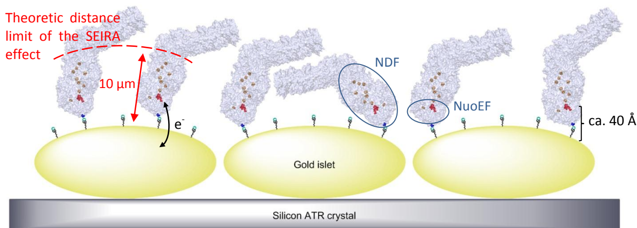
Figure 1.7.1 : Representation of Complex I immobilized on a NiNTA SAM at a SEIRA-active gold surface. The cofactors of Complex I are shown as colored dots, with FMN in red. The location of the Histag is indicated by the blue dots. The distance between FMN and the gold surface is at least 40 Å.
