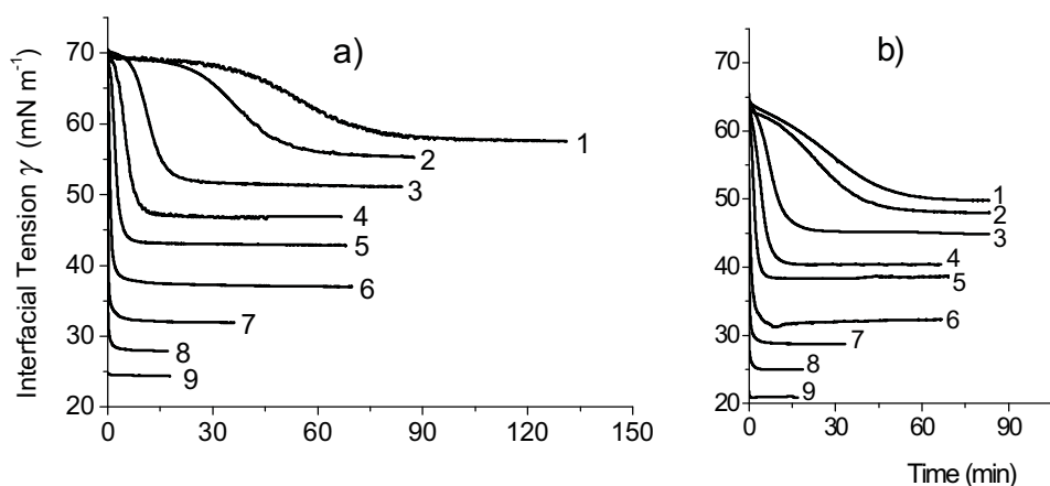
Figure S2. Interfacial tension \gamma at 25°C of DiC 8 -PC at a) the air/HEPES buffer interface, and b) at the PFH-saturated air/HEPES buffer interface, as a function of time. Concentrations of the PL solution (mol L -1 ) were: 1: 5 \times 10^{-7} ; 2: 10^{-6} ; 3: 2.5 \times 10^{-6} ; 4: 5 \times 10^{-6} ; 5: 10^{-5} ; 6: 2.5 \times 10^{-5} ; 7: 5 \times 10^{-5} ; 8: 10^{-4} ; 9: 2.5 \times 10^{-4} .
