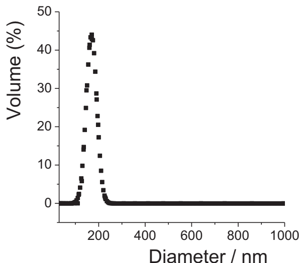
Figure S2. Dynamic light scattering of Fe 3 O 4 nanoparticles dispersed in the HEPES/NaCl buffer at pH 7. The 10 nm NPs form narrowly dispersed clusters of ~170 nm in diameter.
