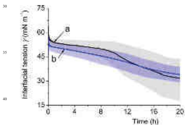
Figure S2. Kinetics of adsorption of DPPC/BSA mixture at the surface of an air bubble at 37^\circ\text{C} . The DPPC/BSA concentrations were: a) 1 \cdot 10^{-3}:7.5 \cdot 10^{-7} \text{ mol L}^{-1} and b) 1 \cdot 10^{-3}:1.5 \cdot 10^{-6} \text{ mol L}^{-1} . The bubble was submitted to oscillations ( T = 10 \text{ s} , \Delta A = 15\% ) for 20 \text{ h} . The lightly colored area represents the fluctuations in interfacial tension associated with the oscillations. The solid lines correspond to mean values obtained by treating the data through a low-pass digital filter.
