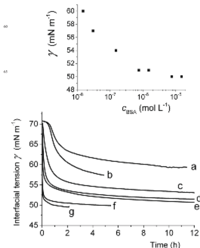
Figure 1. Kinetics of adsorption of BSA on the surface of an air bubble at 37°C (static bubbles). BSA concentrations in Hepes buffer were a) 1.5 \cdot 10^{-8} \text{ mol L}^{-1} ; b) 3.0 \cdot 10^{-8} \text{ mol L}^{-1} ; c) 7.5 \cdot 10^{-8} \text{ mol L}^{-1} ; d) 1.5 \cdot 10^{-7} \text{ mol L}^{-1} ; e) 7.5 \cdot 10^{-7} \text{ mol L}^{-1} ; f) 1.5 \cdot 10^{-6} \text{ mol L}^{-1} ; and g) 1.5 \cdot 10^{-5} \text{ mol L}^{-1} (arrow). The inset shows the variation of the interfacial tension \gamma of an aqueous BSA solution as a function of BSA concentration c_{\text{BSA}} at 37°C.
