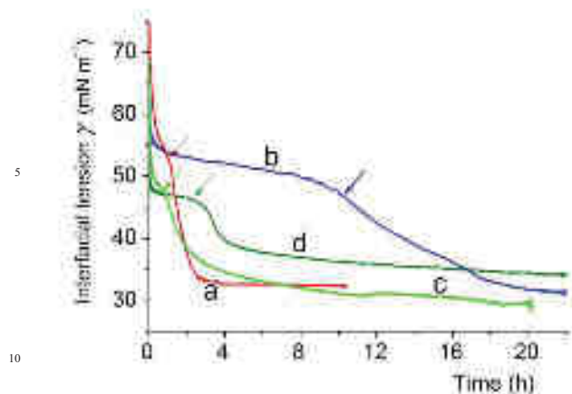
Figure 5. Kinetics of adsorption (37°C) at the surface of an air bubble of a) and c) DPPC alone ( 10^{-3} mol L ^{-1} , provided as a dispersion of vesicles); b) and d) DPPC/BSA ( 1 \cdot 10^{-3} : 7.5 \cdot 10^{-7} mol L ^{-1} ) combination; the DPPC, or DPPC/BSA combination, is adsorbed at the surface of a bubble of air (a) and b)) or at the surface of a bubble of air saturated with F -hexane (c) and d)). All the bubbles were submitted to oscillations ( T 10 s, \Delta A 15%) throughout the experiments. The solid lines correspond to mean values obtained by treating the data through a low-pass digital filter.
