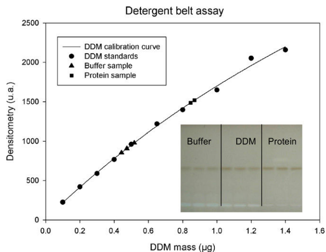
Fig. 5. Evaluation of the final detergent protein ratio following RC-LH1-pufX purification. DDM standards in Tris-NaCl (circles) ranging from 0.1 to 1.4 µg are fitted by a Michaelis-Menten calibration curve. 5 µL of elution buffer (triangles) and 1 µL of the purified PM (0.79 mg/ml) (square) were applied in triplicate.
