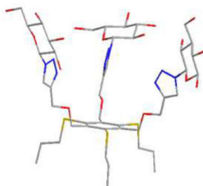
Figure 2.25 – Structure 3D du C3Glu3
