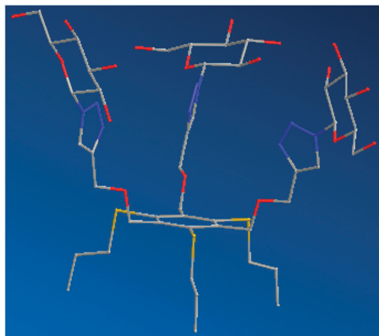
Fig. 3 Representation of a stick molecular model of the tripod C3Glu3 (Chem3D Pro 11.0).
