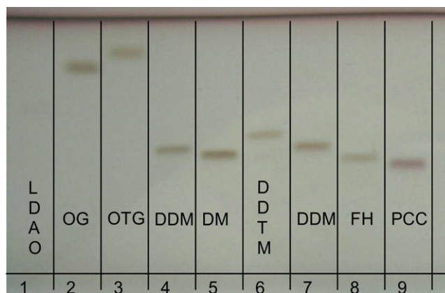
Fig. 7. Separation of surfactants frequently used in the field of MP via HPTLC. 1 \mu g of each surfactant in water is sprayed-on and developed with optimized migration conditions. Lanes (1) N,N-dimethyldodecylamine-N-oxide (LDAO); (2) octyl \beta -D-glucopyranoside (OG); (3) octyl- \beta -D-thioglycopyranosides (OTG); (4 and 7) dodecyl- \beta -maltoside (DDM); (5) n-decyl- \beta -D-maltopyranoside (DM); (6) n-dodecyl- \beta -D-thiomaltopyranoside (DDTM); (8) F4H5- \beta -maltoside (FH); (9) PCC- \alpha -maltoside (PCC).
