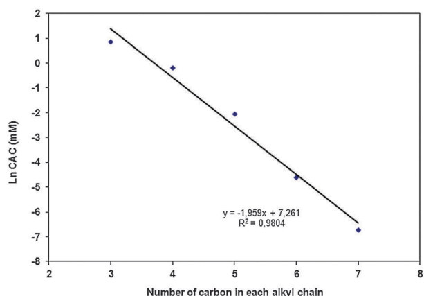
Fig. 4 logCAC plotted vs. number of carbons of the hydrophobic chains.
