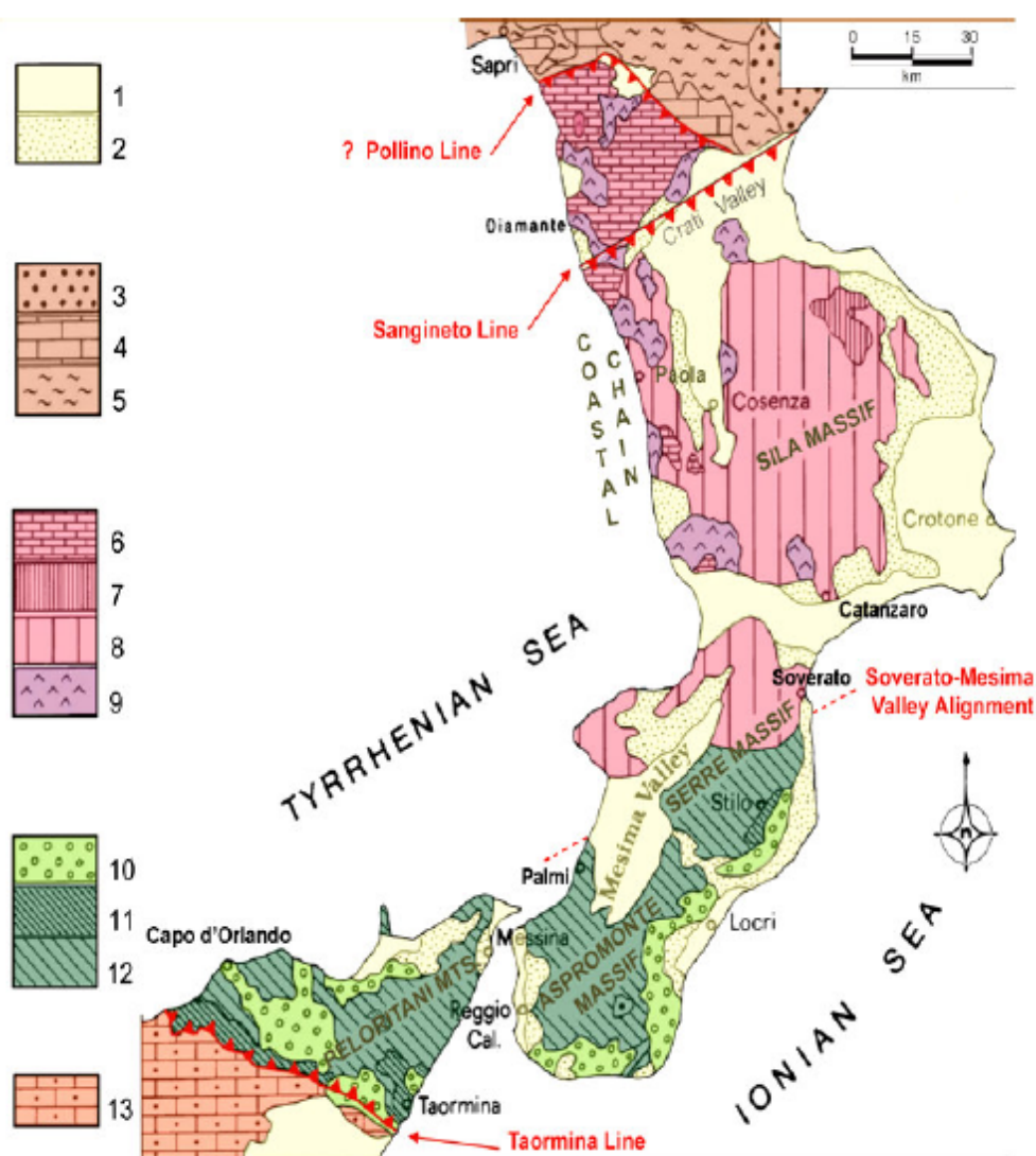
Figure 2: geological map of the Calabro-Peloritani arc, including the Milazzo Peninsula (from Macaione et al., 2010)
